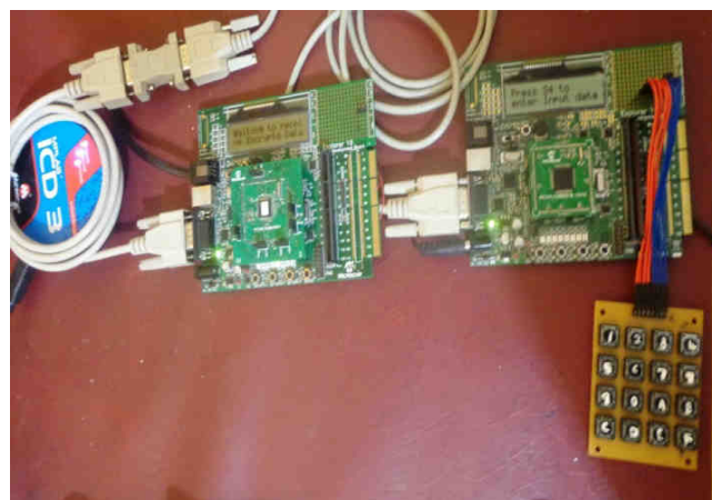
Figure 8. Experimental Setup for Hardware Testing
