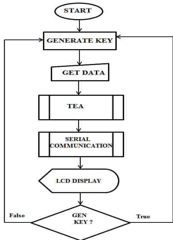
Figure 3. Flowchart for Encryption Unit
