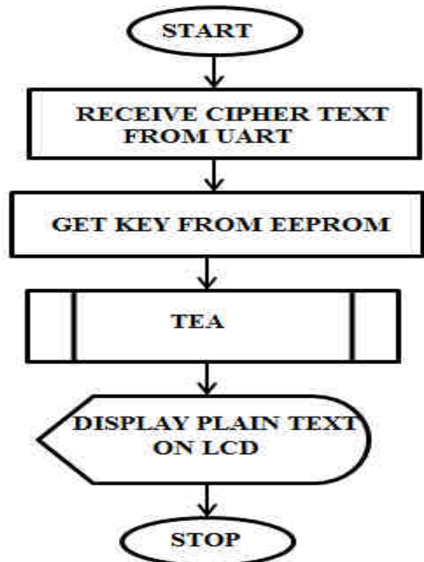
Figure 4. Flowchart for Decryption Unit
