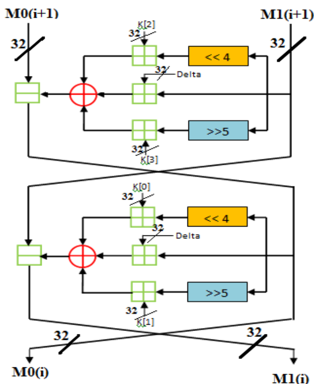
Figure 7. TEA Decryption Process
