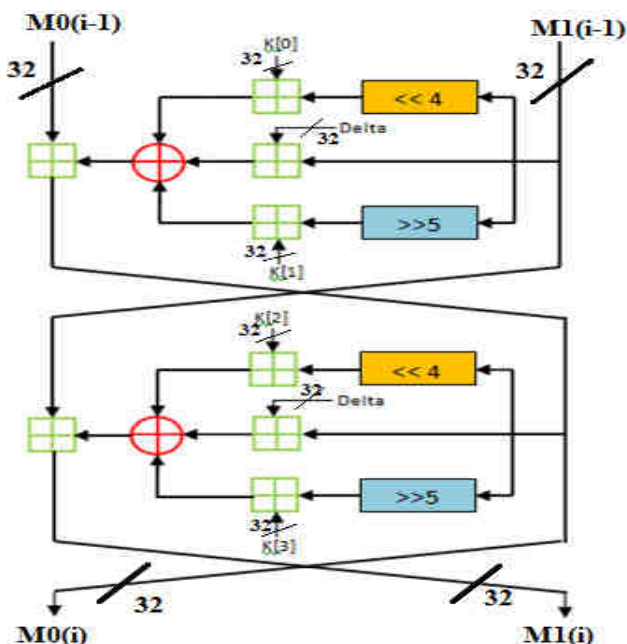
Figure 6. TEA Encryption Process
