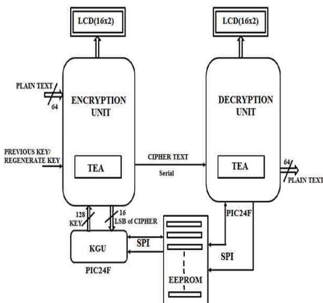
Figure 2. Block diagram of proposed system
