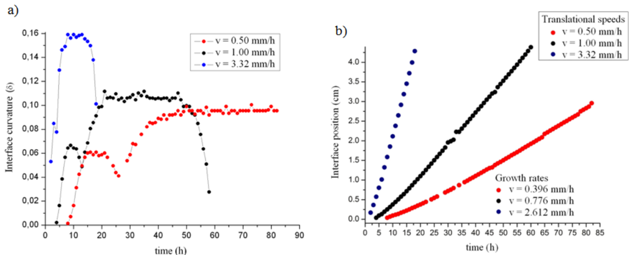
Figure 6. (a) Interface curvature as a function of the simulation time, for the three simulated translational speeds; (b) Interface position as a function of the simulation time for the three simulated translational speeds
