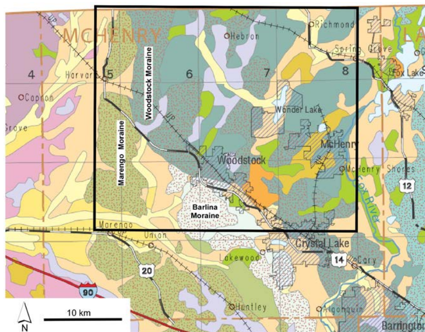
Figure 2. Surficial geologic map of McHenry County and surrounding areas (Modified from Stiff et al., [28]). Study area is outlined in black. Positions of the major moraines are indicated. Pink = Illinoisan units; Oranges = various outwash facies of the Henry Formation; Pale purple = Equality Formation, Dull green and teal = Wedron Formation, Bright green = Grayslake Peat; Yellow = Cahokia Alluvium
