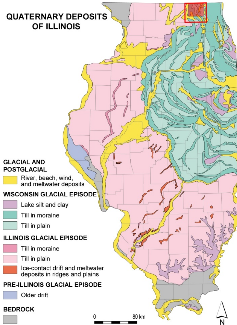
Figure 1. Surficial geologic map of Illinois showing the distribution of Quaternary glacial deposits. McHenry County is outlined in red. The pale red shading within is the study area. Map is modified ISGS Staff, 2005, Quaternary deposits: Illinois State Geological Survey, ISGS 8.5 × 11 map series
