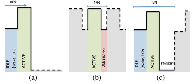
Figure 5: Power behavior for single capture (a), standard sequential capture (b) and sequential capture with aggressive standby mode (c)
