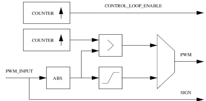
Fig. 5. Block diagram of the PWM modulator.
