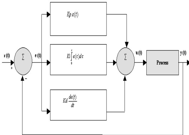
Figure 1 : Block diagram of PID controller
