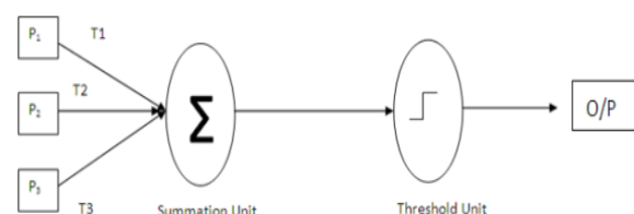
Figure 6: Shows the Neuron model for a web session
