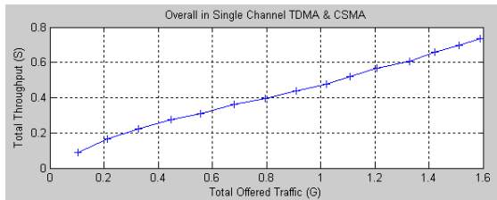
Figure 5 Total throughput for Single Channel combined System
