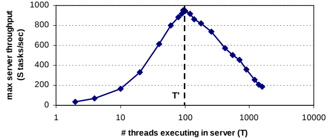
Figure 3: Threaded server throughput degradation : This benchmark has a very fast client issuing many concurrent 150-byte tasks over a single TCP connection to a threaded server as in Figure 2 with L = 50\text{ms} on a 167 MHz UltraSPARC running Solaris 5.6. The arrival rate determines the number of concurrent threads; sufficient threads are pre-allocated for the load. As the number of concurrent threads T increases, throughput increases until T \geq T' , after which the throughput of the system degrades substantially.
