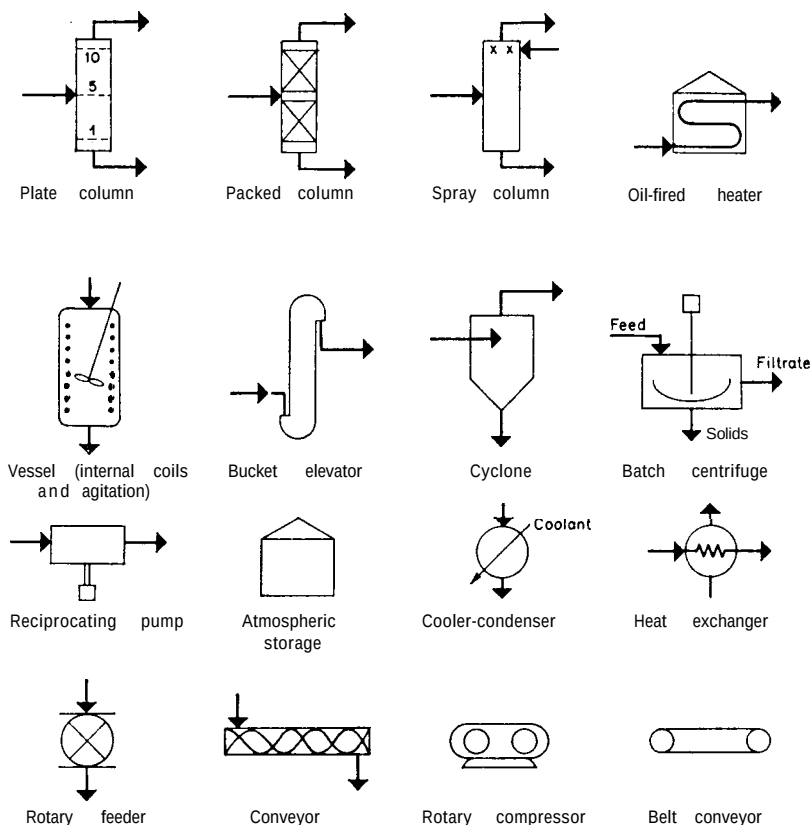
Figure 4-1 Typical flowsheet symbols.
