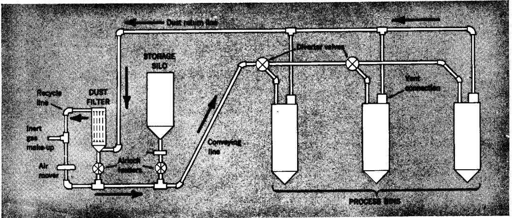
Figure 4-5 A closed loop system which can operate under either vacuum or pressure. Courtesy Kraus, M.N.: "Pneumatic Conveyors," Chemical Engineering , Oct. 13, 1969, p. 61.
