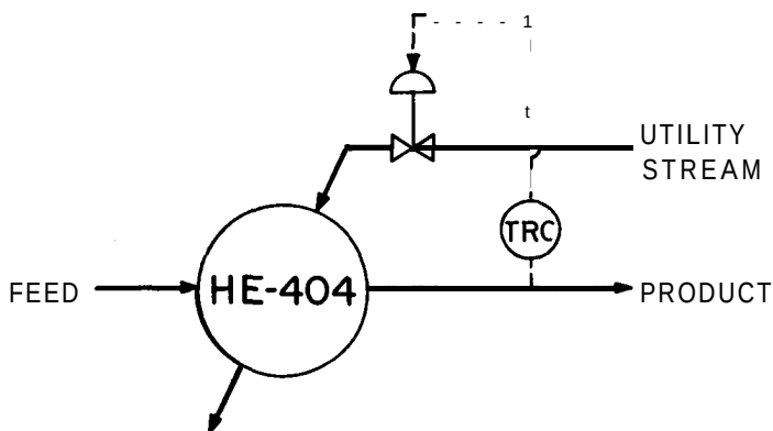
Figure 7-9 Cascade temperature control.
