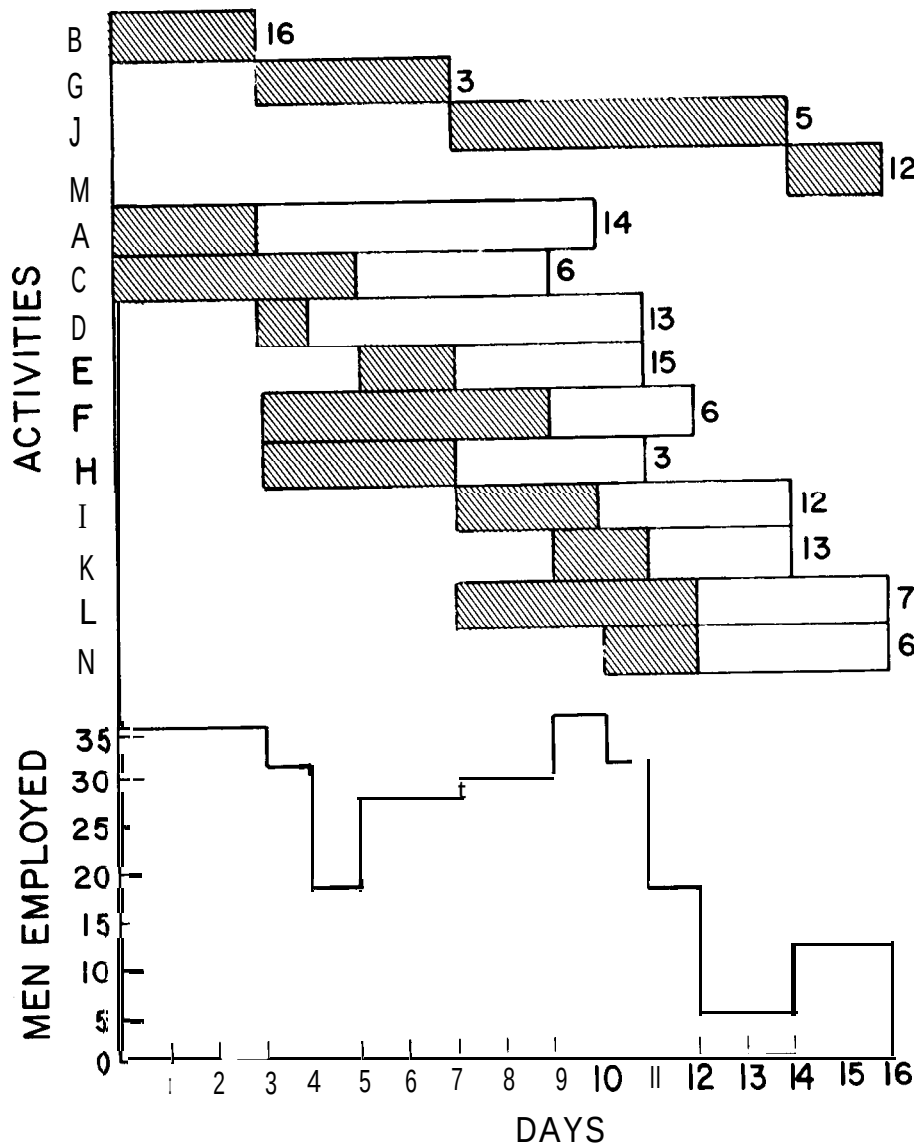
Figure 13-4 The number of men employed in each activity and totally if each activity for a project begins as soon as it can.
