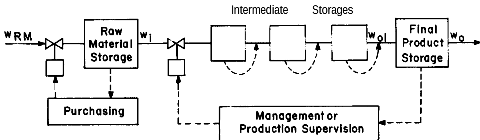
Figure 7-3 Overall material balance control with intermediate material balance controls in the direction of flow.
