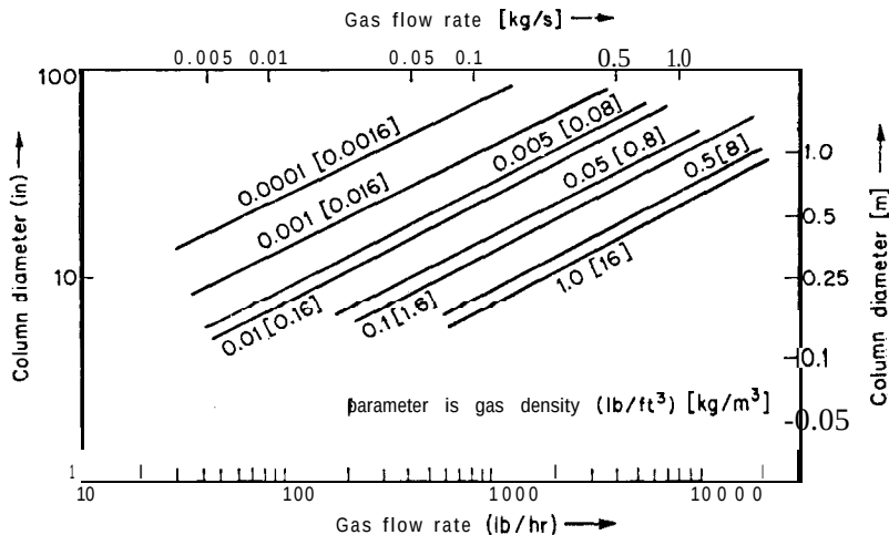
Figure S-2 Estimation of packed column diameters.
