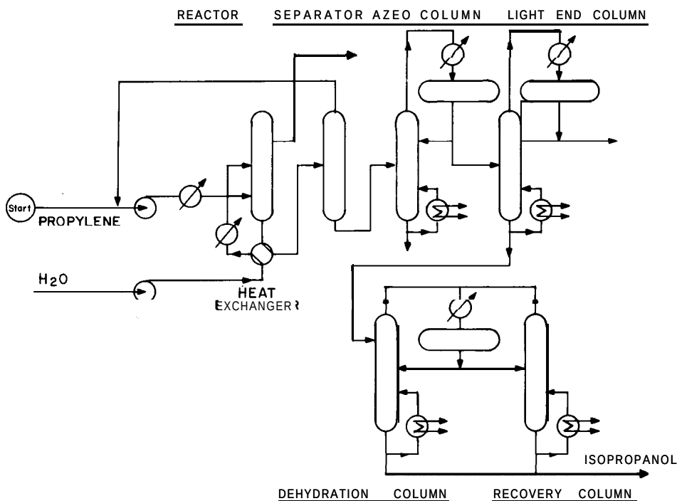
Figure 9-5 Isopropanol production flow sheet.
