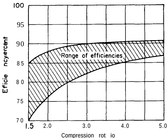
Figure 8-8 Reciprocating compressor efficiencies.
