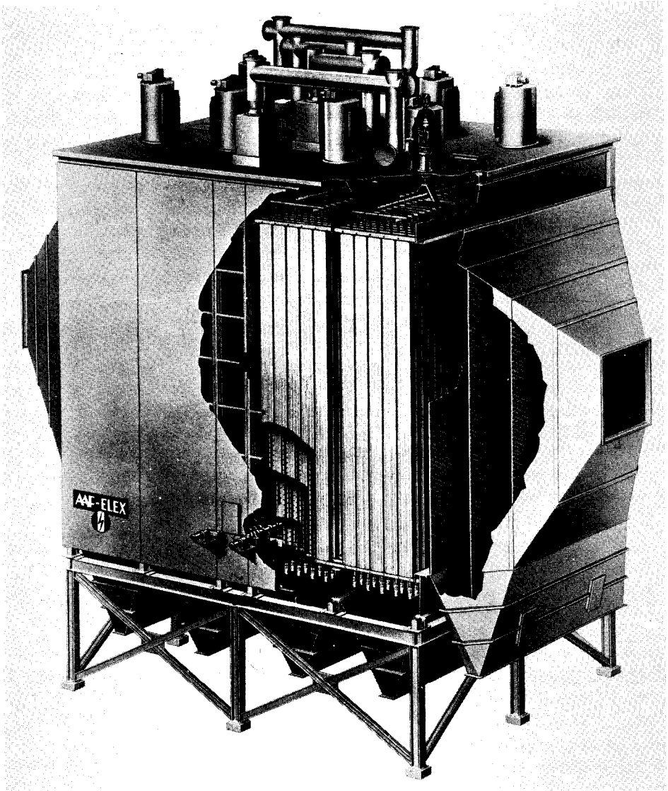
Figure 16-1 A cutaway view of an electrostatic precipitator. The gas flows in one side and out the other. The particles in the incoming air are attracted to the charged plates. The plates are periodically rapped. This causes the particles to fall to the bottom where they are collected. Courtesy of the American Air Filter Company.
