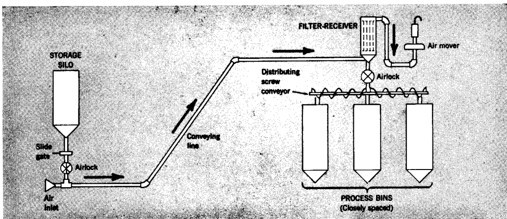
Figure 4-3 A vacuum system for transferring solids from storage silos to one receiver. Courtesy Kraus, M.N.: "Pneumatic Conveyors," Chemical Engineering , Oct. 13, 1969, p. 60.
