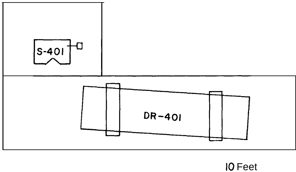
Figure 6E-3 Finishing building: drying area. Front view.
