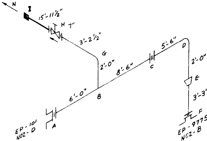
Figure 12-3 A portion of pipe sketch. At point A is a flange connecting nozzle D on a piece of equipment EP- 101 with the line. Similarly, at point F a flange connects nozzle B of equipment EP-9775 to the line. H is a valve, E is a reducer, and C is a joint. The distances of each pipe segment are given in feet and inches. Courtesy of E. I. duPont de Nemours & Company.
