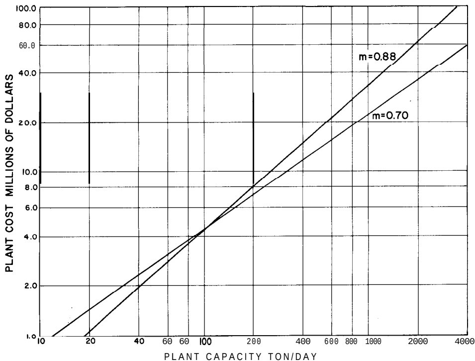
Figure 9-1 Plant cost as a function of capacity for two different cost exponents. The curve form m = 0.88 is the same as that given by Berk, J. M. and Haselbarth, J. E. for Ammonia Plants in "Cost Capacity Data IV" Chemical Engineering , Mar. 20, 1961, p. 186.
