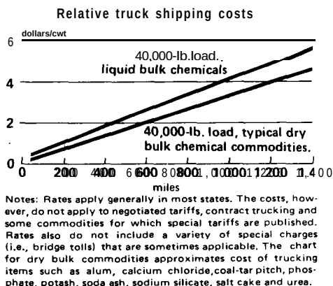
Figure 2-2 Relative Truck Shipping Costs. Courtesy of Winton, J.M.: "Plant Sites '74," Chemical Week , Oct. 17, 1973, p. 45.
