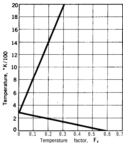
Figure 9-2 Temperature factor curve used in the Zevnik-Buchanan method.
