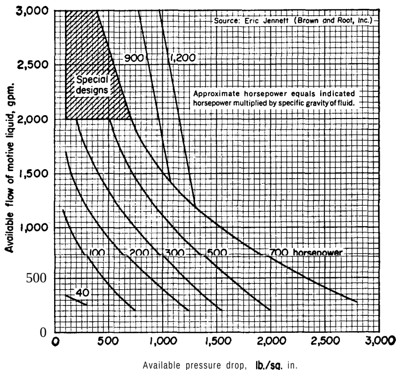
Figure 8-1 The energy that may be recovered from fluids by using pump-turbines. Source: Miller, R.J., Jr.: "Process Energy Systems," Chemical Engineering , May 20, 1968, p. 130.
