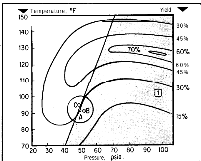
Figure 14-5 A response surface that is not strongly unimodal Courtesy: Baasel, W.D., "Exploring Response Surfaces to Establish Optimum Conditions," Chemical Engineering , Oct. 25, 1965, pg. 149.
