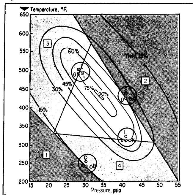
Figure 14-4 A graphical method of finding the optimum.
