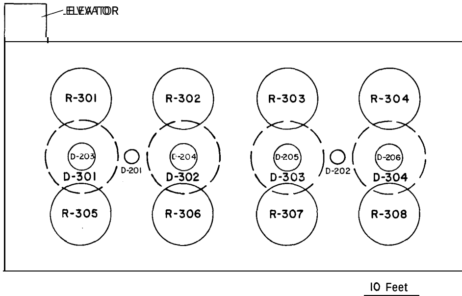
Figure 6E-2 Reactor building - top view.
