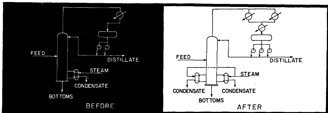
Figure 5-1 Auxiliary units for a distillation column before and after expansion.
