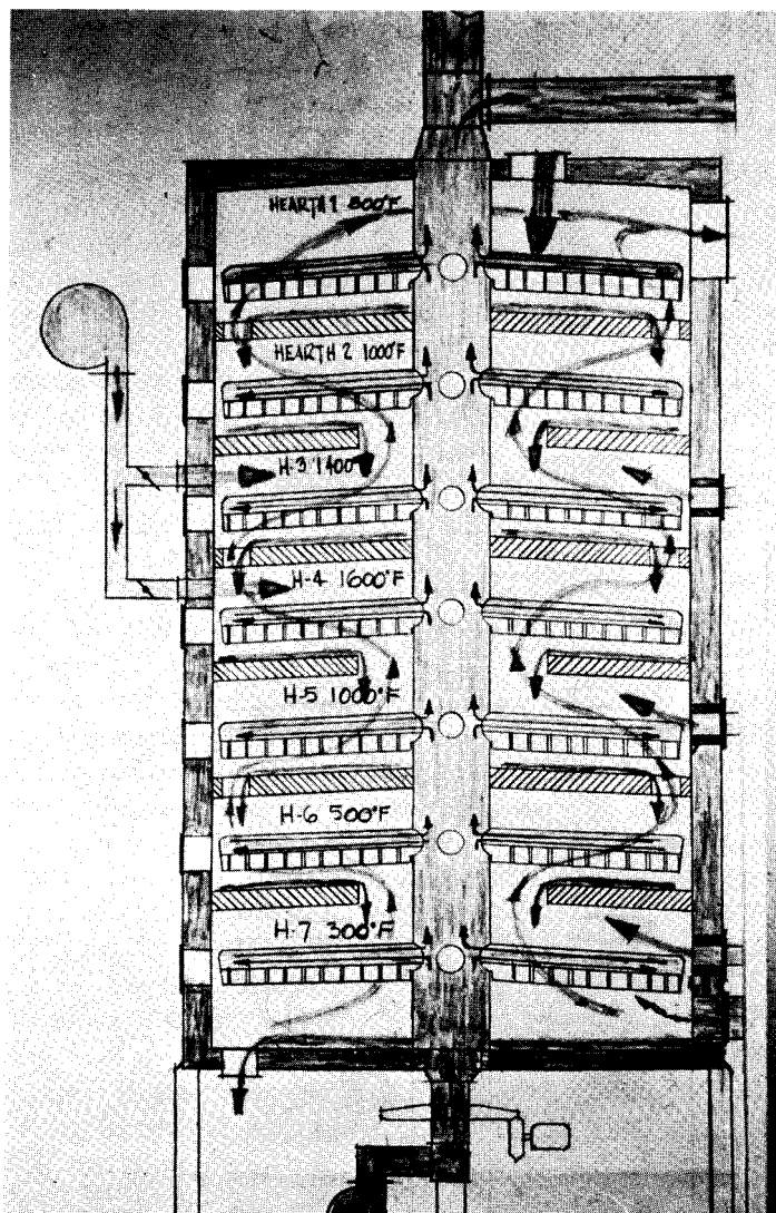
Figure 16-6 Multiple-hearth incinerator. The wet solids enter at the top of the incinerator onto the top hearth. A rake-like device plows the sludge across the top to drop holes where they descend to the hearth below. The agitation of the sludge exposes the maximum amount of surface to the hot gases, which promotes drying. Courtesy of the North American Manufacturing Company.
