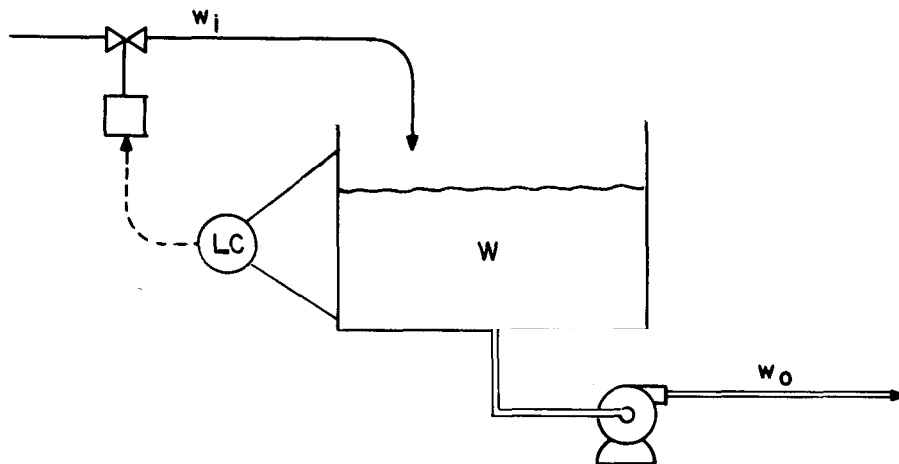
Figure 7-5 Material balance control in the direction opposite to flow.
