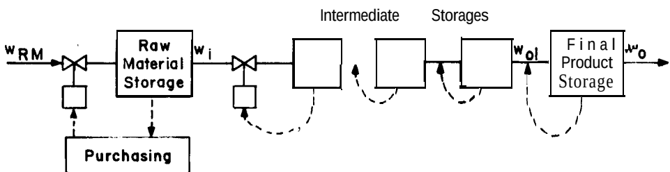
Figure 7-4 Overall material balance control in direction opposite to flow.
