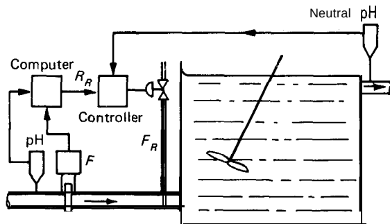
Figure 7-10 A control system for the neutralization of waste by reagent R. Source: Friedman, P.G., Moore, J.A.: "For Process Control Select the Key Variables," Chemical Engineering , June 12, 1972, p. 90.
