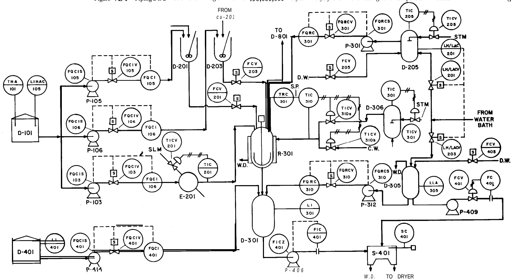
Figure 7E-1 Piping and Instrument Diagram for a 150,000,000 lb/year Polystyrene Plant Using the Suspension Process. a
