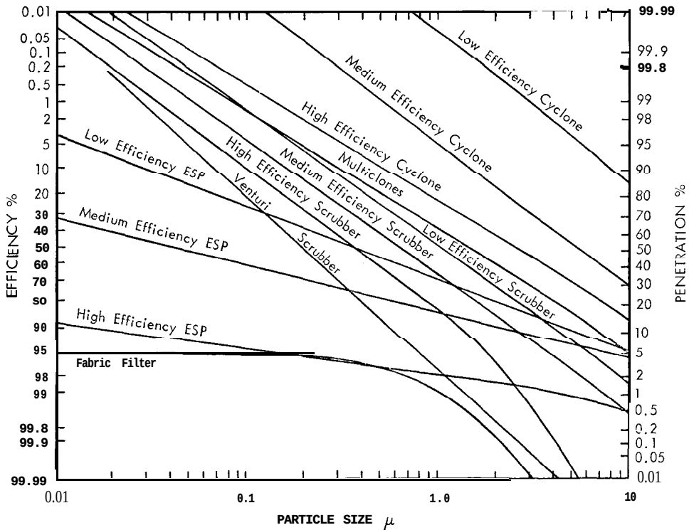
Figure 16-3 The fractional efficiency of various devices for removing various size particles from air. Vandegrift, the originator of this figure, cautions that in the region below 0.5 microns the data are rather sparse. ESP stands for electrostatic precipitator. Source: Vandegrift, A.E., Midwest Research Institute.
