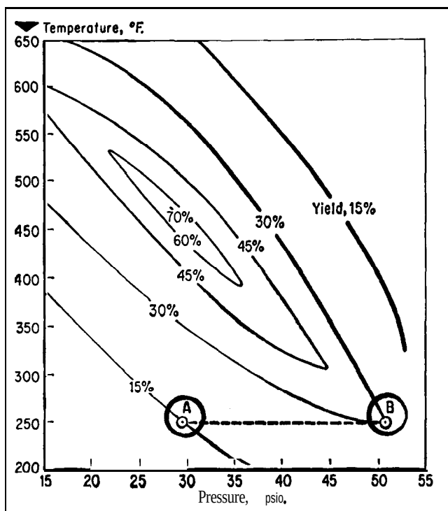
Figure 14-1 Possible response surface for a Chemical Reactor.
