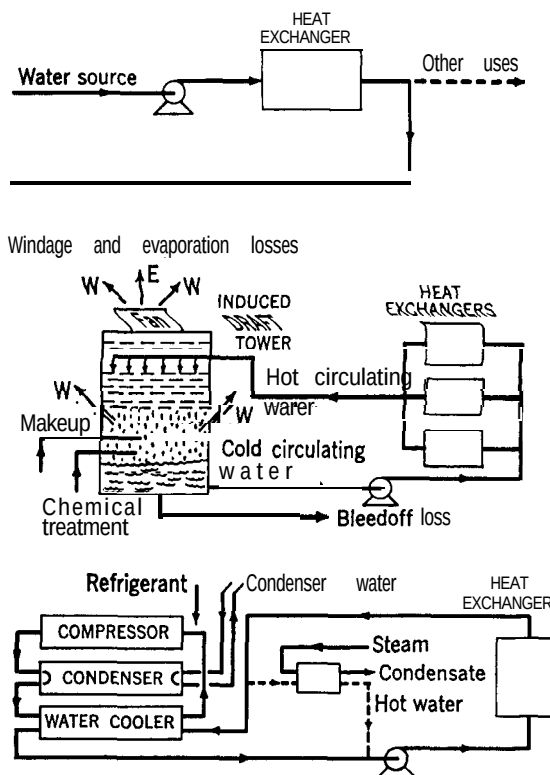
Figure 8-3 Three basic types of cooling water systems. Top: the once-through system where the cooling water is used once and then discharged. Middle: the open recirculation system where the water is cooled and recycled through a system in which it comes in direct contact with air. Bottom: a closed recirculation system where the water is cooled and recycled without coming in direct contact with the atmosphere. Source: Silverstein, R.M., Curtis, S.D.: "Cooling Water," Chemical Engineering , Aug. 9, 1971, p. 88.
