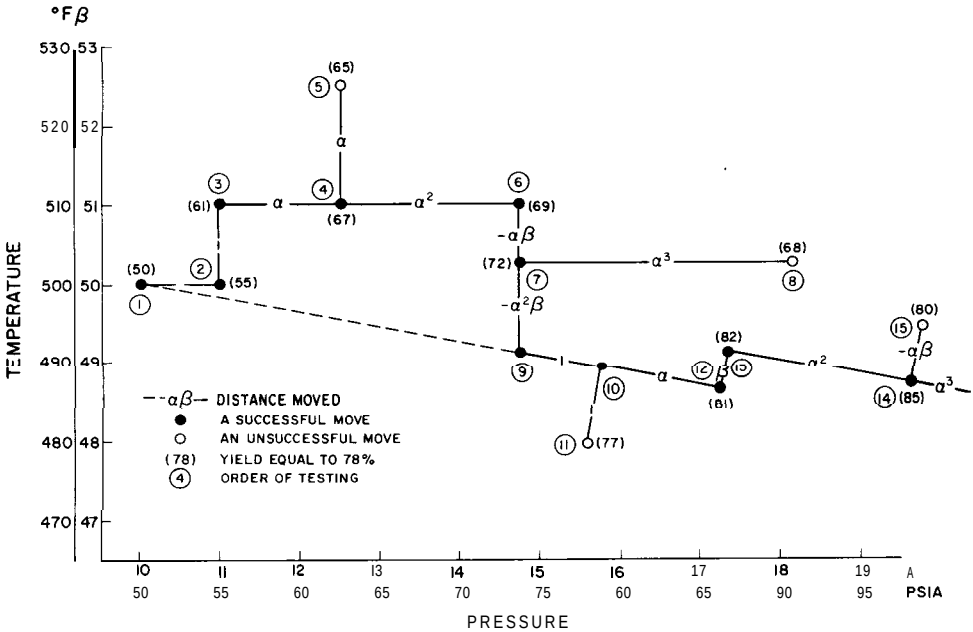
Figure 14-3 Rosenbrock's method for determining the optimum reactor conditions.
