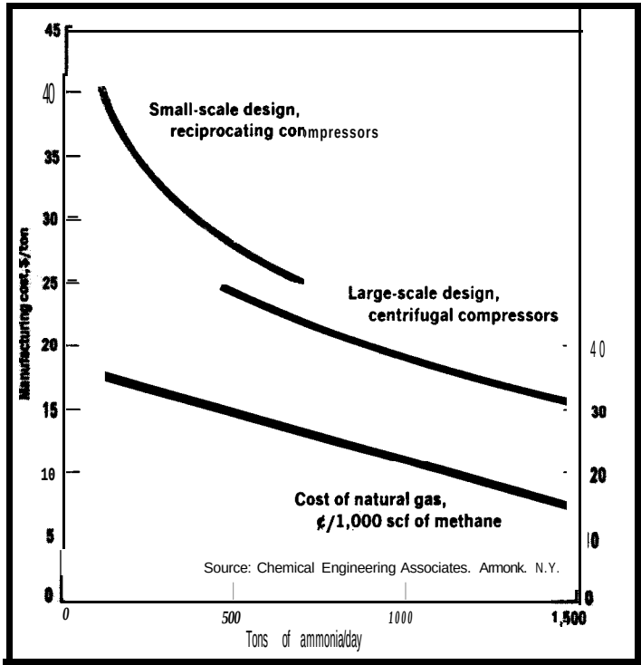
Figure 3-1 Cost vs. capacity curve for ammonia in 1967. Source: "Bell Tolls for Little Plants," Chemical Week , Oct. 28, 1967, p. 127.
