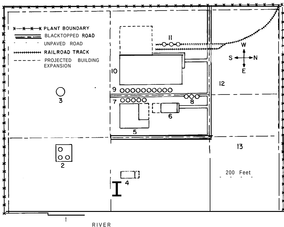
Figure 6E-6 Plant layout for a 150,000,000 lb / year polystyrene plant using the suspension process.
