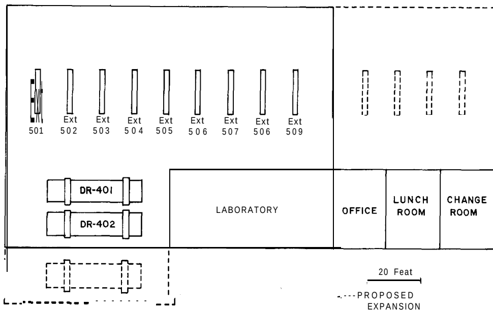
Figure 6E-5 Finishing building — top view.
