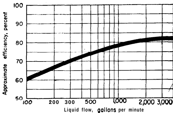
Figure 8-5 The approximate efficiencies of process pumps. Source: Miller, R.J., Jr.: "Process Energy Systems," Chemical Engineering , May 20, 1968, p. 130.
