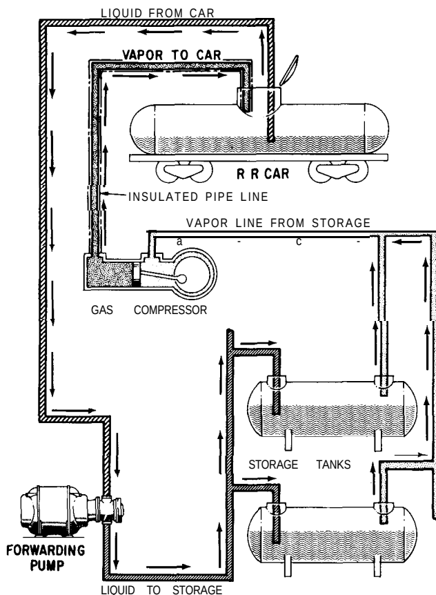
Figure 4-2 A typical tank car unloading system for unloading compounds with low boiling points. Courtesy Dow Chemical Company, U.S.A.
