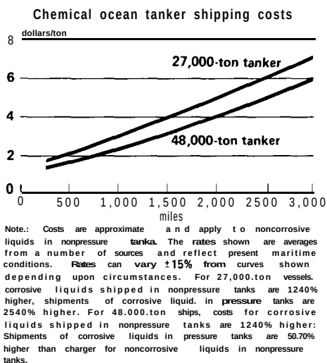
Figure 2-3 Chemical ocean Tanker shipping costs. Courtesy of Winton, J.M.: "Plant Sites '74," Chemical Week , Oct. 17, 1973, p. 45.
