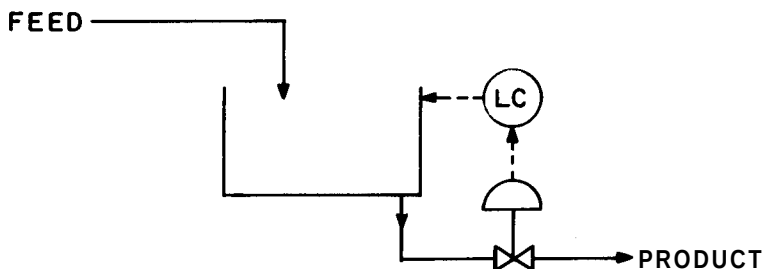
Figure 7-1 Feedback level control system.
