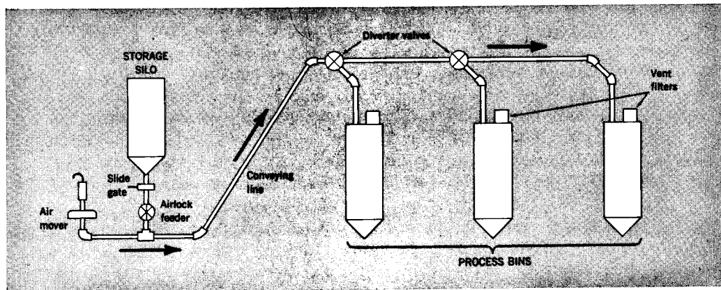
Figure 4-4 A positive pressure system which can deliver product to many receivers. Courtesy Kraus, M.N.: "Pneumatic Conveyors," Chemical Engineering , Oct. 13, 1969, p. 61.
