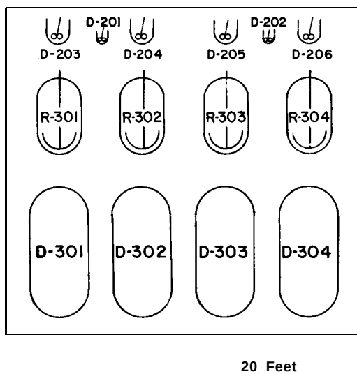
Figure 6E-1 Reactor building — front view.
