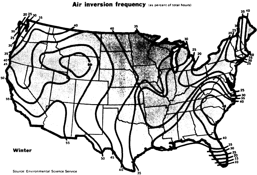
Figure 2-8 Air inversion frequency. Courtesy of Winton, J.M.: "Plant Sites Report '68," Chemical Week , Oct. 5, 1968 p. 96.
