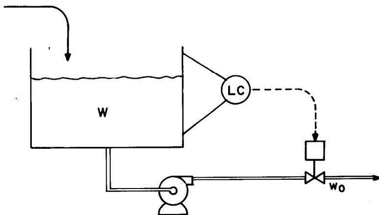
Figure 7-2 Material balance control in the direction of flow (Averaging Control).
