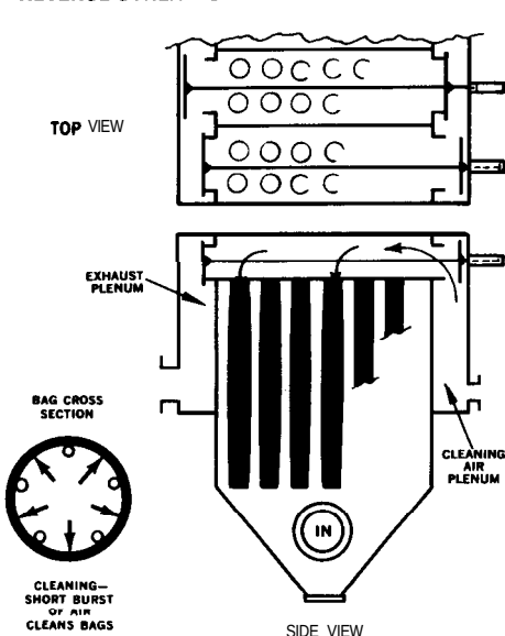
Figure 16-2 A cloth filter. The dirty air enters in the side near the bottom as shown in the figure on the left. The large particles drop to the bottom. The small particles are carried upward and deposited on the exterior surface of bag (shown in black). The air passes through the bag and exits through the exhaust plenum. The bags are cleaned periodically, but only a few at a time. When this occurs the exhaust plenum is closed as shown in the figure on the right. A burst of air is admitted to the inside of the bags; this knocks the small particles off the sides and they settle to the bottom where they are discharged through a rotary valve. Courtesy of the Dustex Division of American Precision Industries, Inc.
