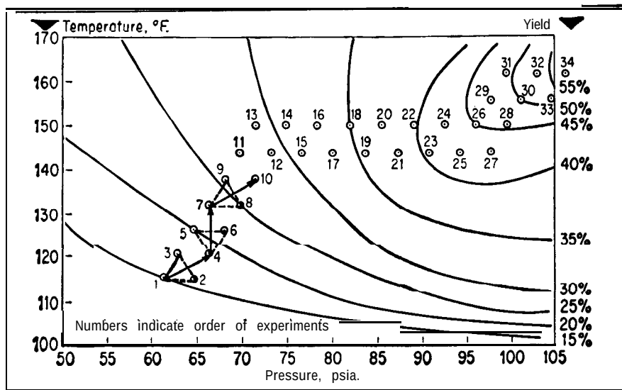
Figure 14-6 The simplex method for finding the optimum.
