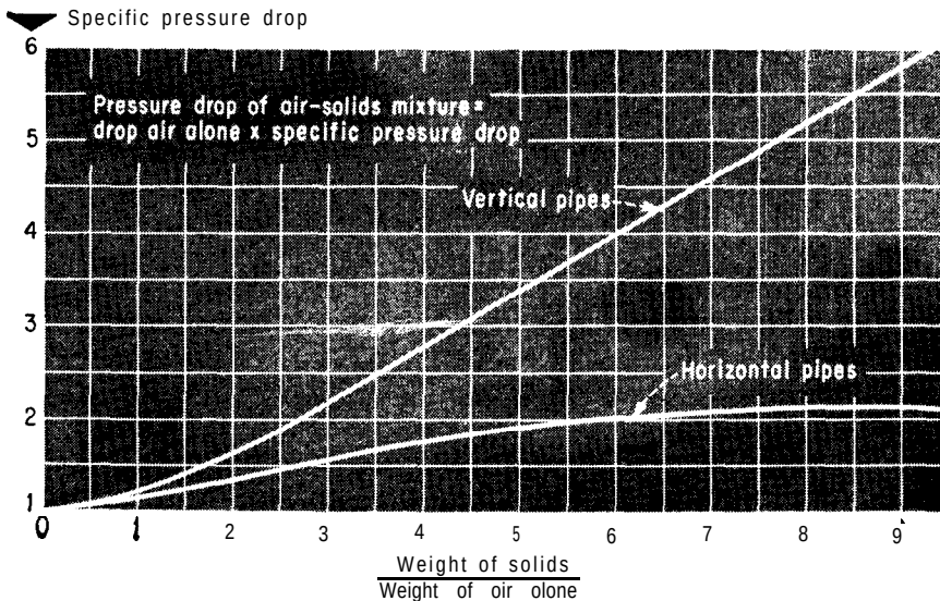
Figure 8-11 Ratio of the pressure drop for fluids containing solids to that for the fluids without solids. Source: Constance, J.D.: "Calculating Pressure Drops in Pneumatic Conveying Lines," Chemical Engineering , Mar. 15, 1965, p. 200.
