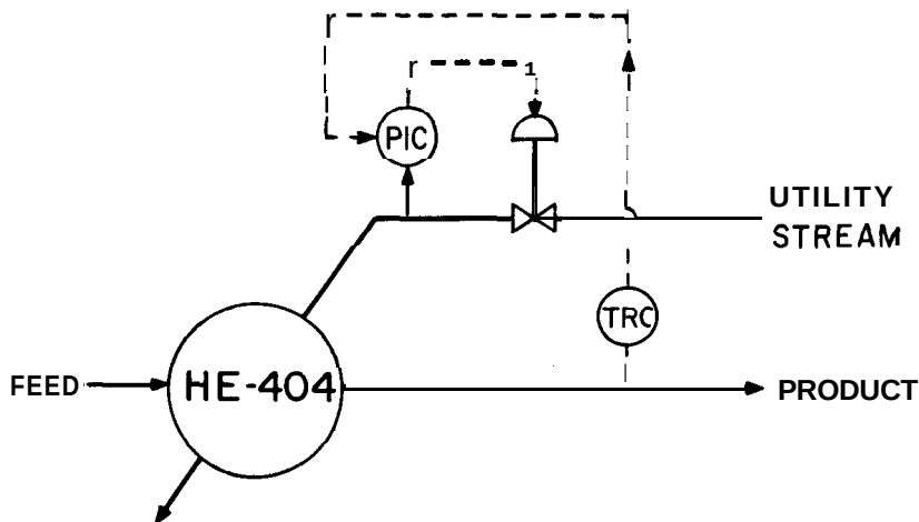
Figure 7-8 Feedback temperature control.
