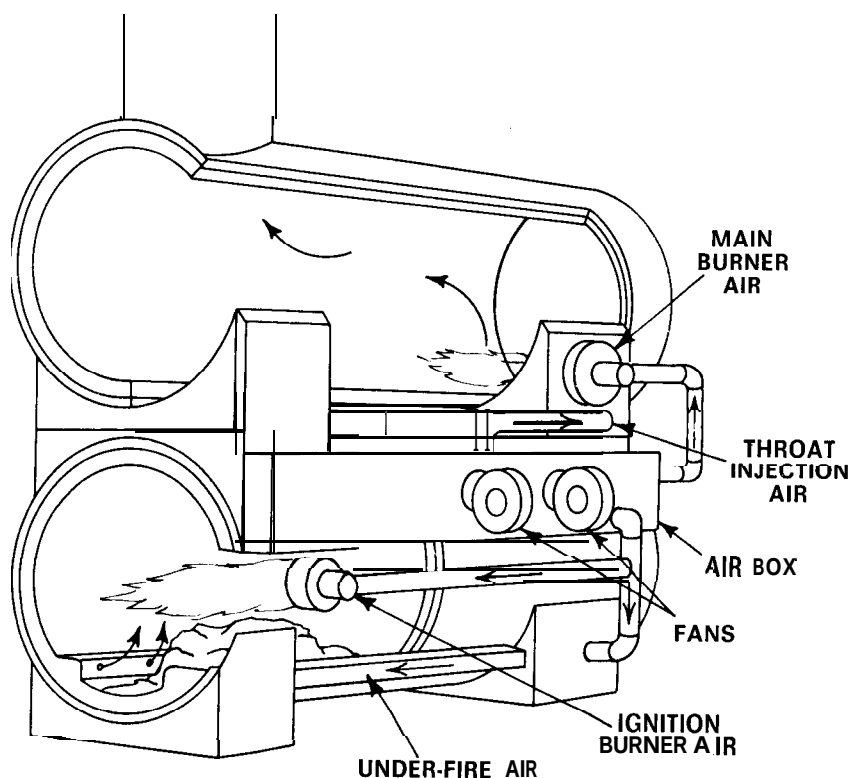
Figure 16-7 A two-chamber incinerator. The raw waste is charged to the lower incinerator- Here it is burned with a limited air supply in order to develop a high temperature which will gasify most of the solid waste material. Between the chambers the gases pass a restriction (throat) where air is injected. They then enter the second chamber and the flame of the main burner.
