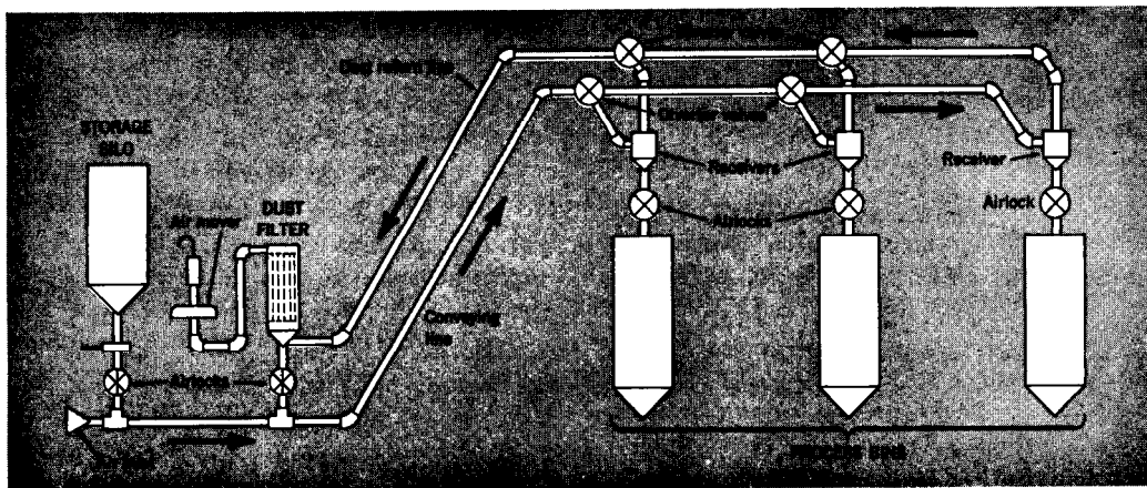
Figure 4-7 A parallel dust return system which permits a vacuum system to distribute material to more than one receiver.
