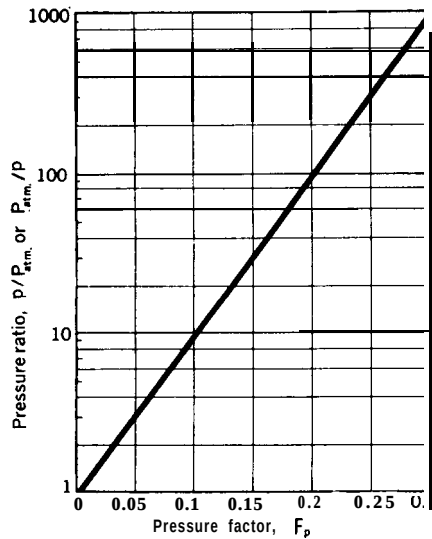
Figure 9-3 Pressure factor curve used in the Zevnik-Buchanan method. Source: Zevnik, F.C., Buchanan, R.L.: "Generalized Correlation of Process Investment," Chemical Engineering Progress , Feb. 1963, p. 71.
