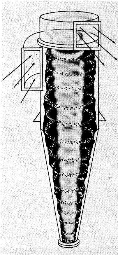
Figure 8-10 A cyclone separator. The air enters tangentially and the solids are thrown out to the sides and leave through the bottom. The air exits at the top either horizontally as shown or, frequently, vertically. Courtesy of American Air Filter Company, Inc.
