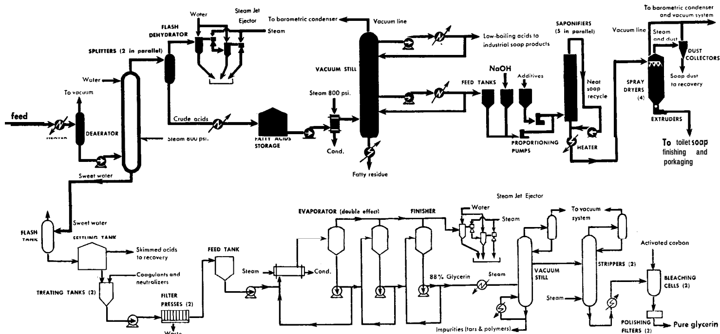
Figure I- 1 Flow Diagram for Armour's Soap Plant. Courtesy of Ladyn, H. W., "Fat Splitting and Soap Making Go Continuous," Chemical Engineering ; Aug. 17, 1964, p. 106.
