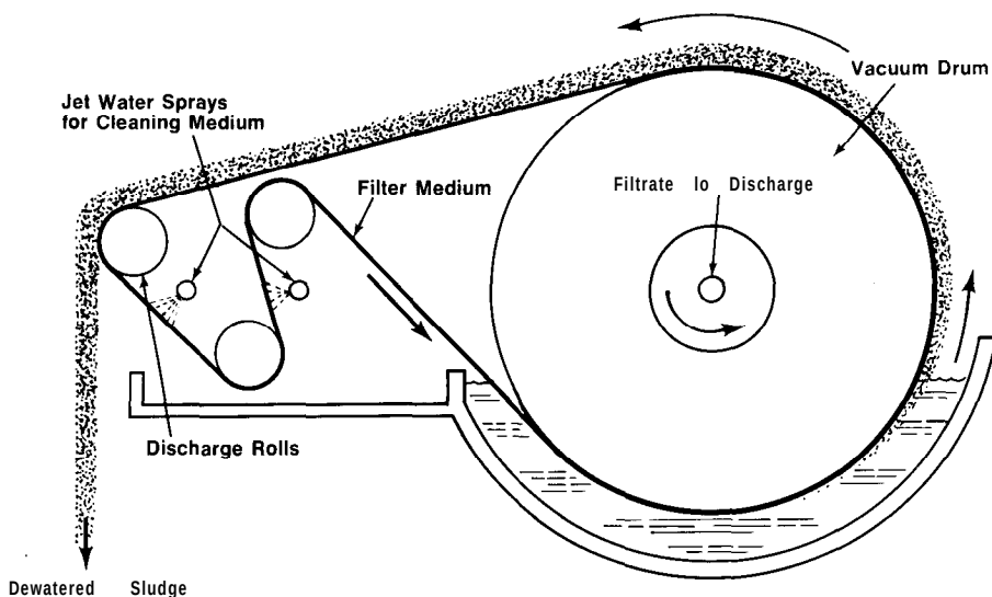
Figure 16-5 A continuous belt drum filter. This works on the same principal as the vacuum drum filter. The drum is immersed in the liquid to be filtered. A vacuum is pulled in the drum to create the pressure drop necessary to cause the fluid to flow through the filter media into the drum. The solids are retained on the surface of the filter medium. After the belt and the adhered solids leave the fluid, the vacuum continues and most of the liquid in the solids is removed. The solids are then discharged and both sides of the belt are cleaned. Courtesy of EIMCO, the Processing Machinery Division of Envirotech Corp.
