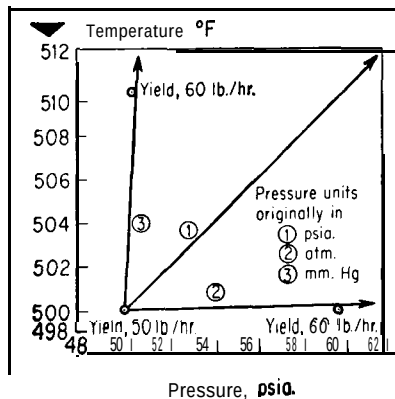
Figure 14-2 Three different paths of steepest ascent which result from using the same data but different units.
