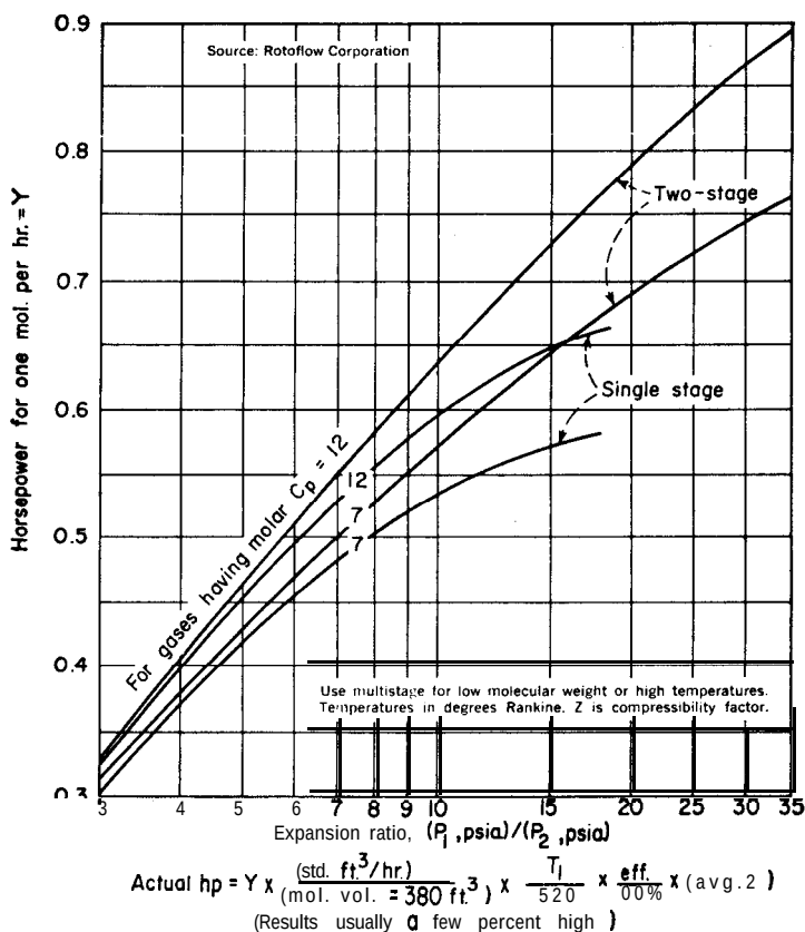
Figure 8-2 The energy that may be recovered from gases by using turbo-expanders. Source: Miller, R.J., Jr.: "Process Energy Systems," Chemical Engineering , May 20, 1968, p. 130.
