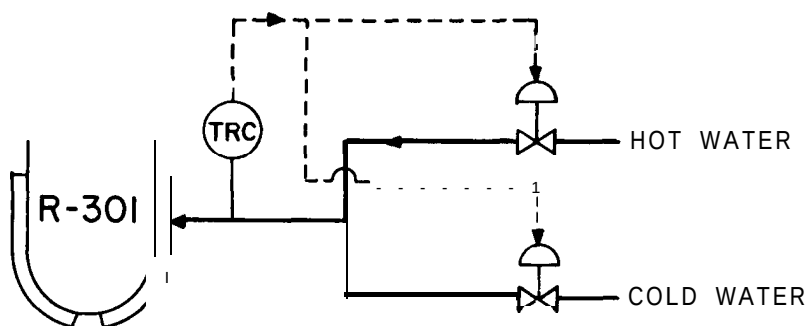
Figure 7-6 Tempered water system.
