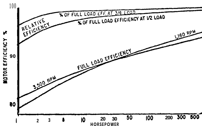
Figure 8-6 Efficiencies of commercial induction motors.
