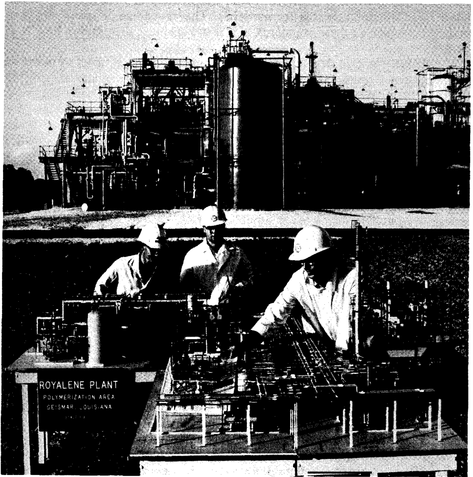
Figure 12-2 Scale Model used in the construction of an ethylene-propylene synthetic rubber plant. The completed plant is partially shown in the background. The model is built to a scale of \frac{3}{8} inch to 1 foot. After construction was completed, it was used to train technicians. Courtesy of Uniroyal.
