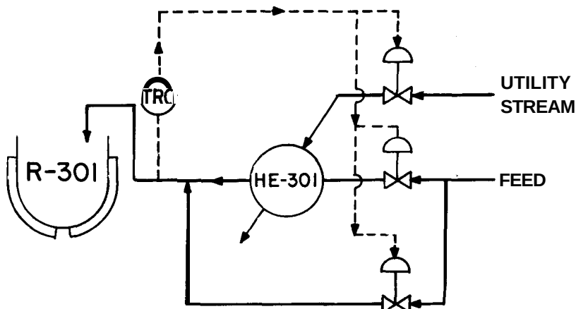
Figure 7-7 Precise temperature control of the feed to a reactor.
