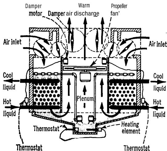
Figure 8-4 A wet surface air cooler.
