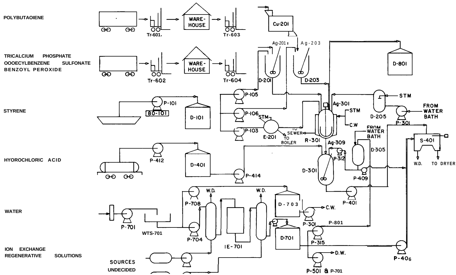
Figure 4E-4 Flow Diagram for a 150,000,000 lb. Per Year Polystyrene Plant Using the Suspension Process
