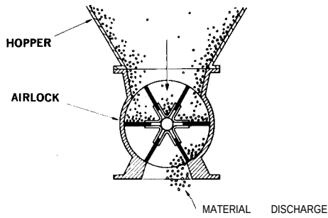
Figure 8-9 Cutaway drawing of a rotary valve. The valve is turned at a given rate by a motor. Courtesy of MicroPul Division of the United States Filter Corporation.
