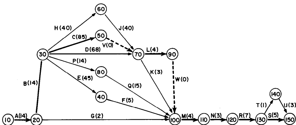
Figure 13-2 An arrow diagram for the installation of a scrubber in an existing process. If the numbers in the circles are ignored, this diagram is typical of one used for a CPM problem; if the projects are identified by numbers and the normal or most likely times are replaced by the
