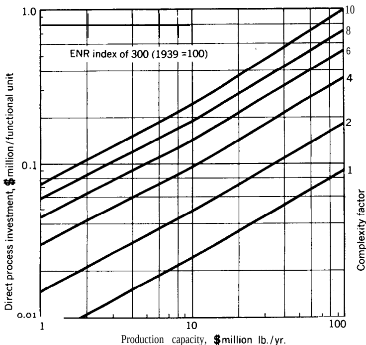
Figure 9-4 Process investment versus process capacity correlation.
