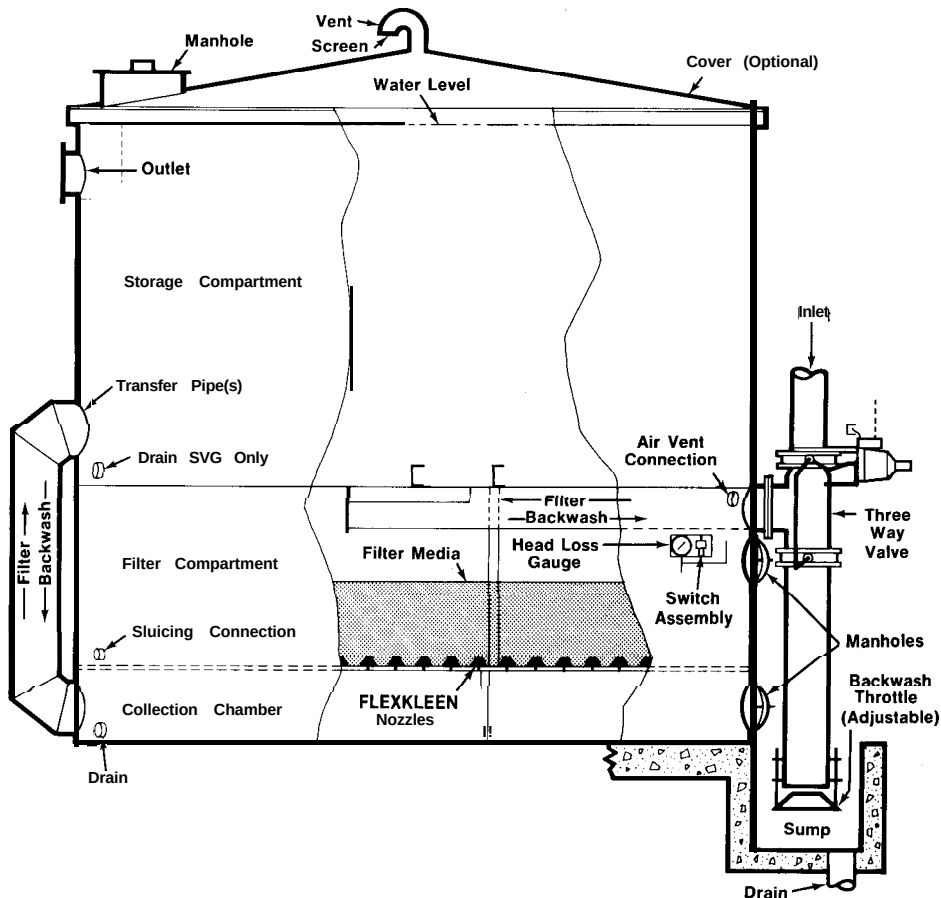
Figure 16-4 A media (sand) filter.
