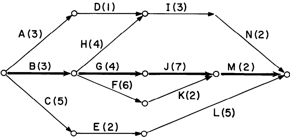
Figure 13-3 The arrow diagram for a project where manpower leveling is important.
