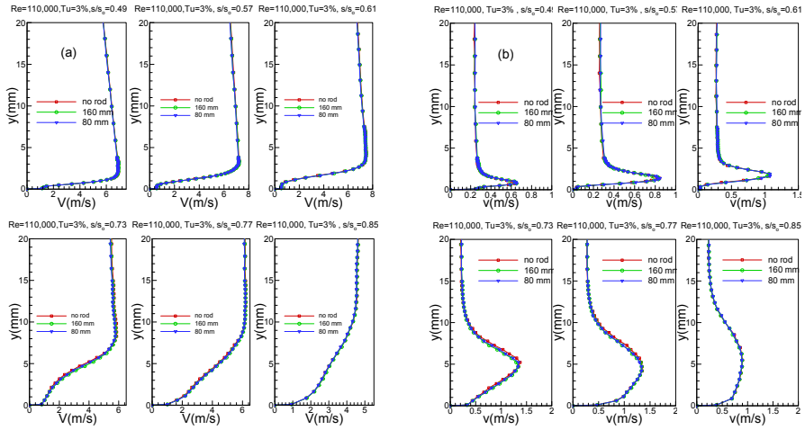
Fig. 11.39: Distribution of time-averaged velocity (a) and turbulence fluctuation rms (b) along the suction surface for steady case \Omega=0 ( S_R=\infty ) and unsteady cases \Omega=1.59 ( S_R=160 mm) and \Omega=3.18 ( S_R=80 mm) at Re=110,000 and Tu=3\% .
