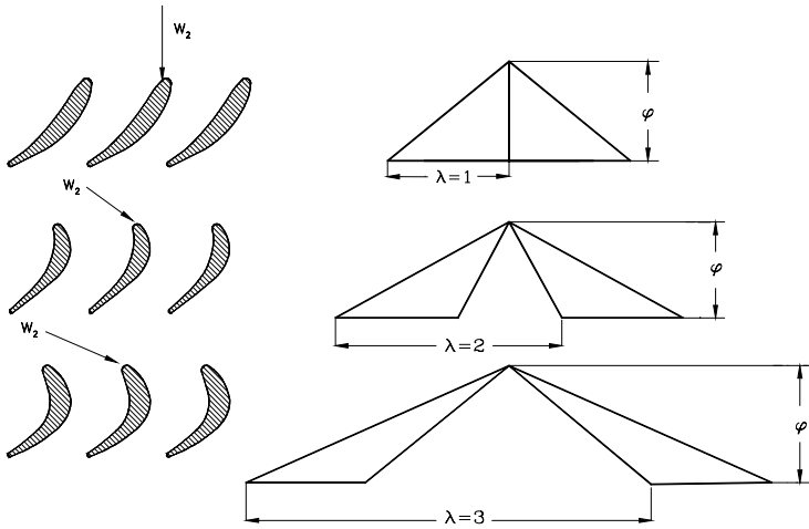
Fig. 5.26: Dimensionless stage velocity diagram to explain the effect of stage load coefficient \lambda on flow deflection and blade geometry, r = 0.5 .
