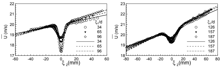
Fig. 10.19: Mean longitudinal velocity distribution in lateral direction, solid lines, Eq. (10.60), experiments from Schobeiri et al. [5].
