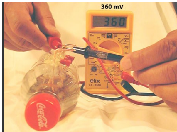
Creating electricity in a cola bottle
