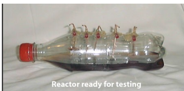
Cola bottle used as a plasma reactor
