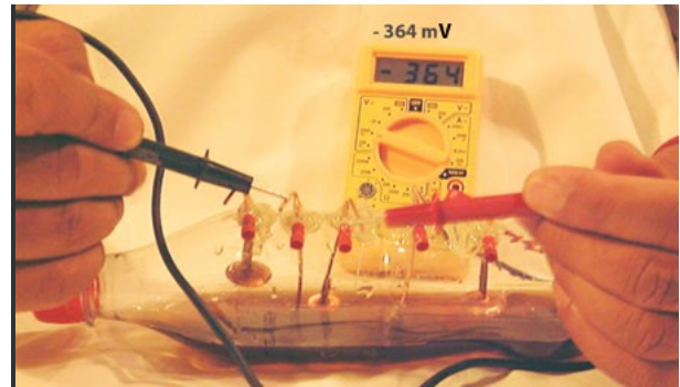
Creating voltage in a cola bottle
