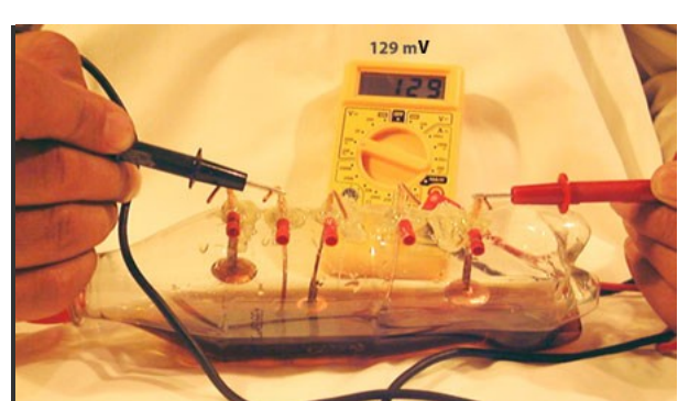
Creating current in a cola bottle
