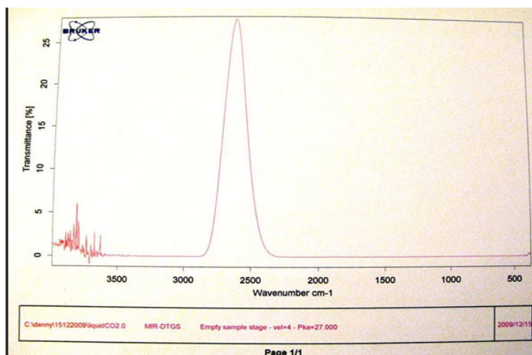
IR spectroscopy graph of the CO 2 substance
