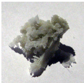
Solid CO 2 at room temperature
