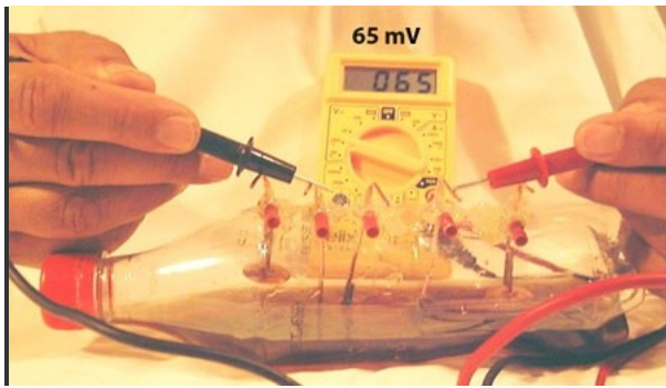
Creating voltage and current in a cola bottle
