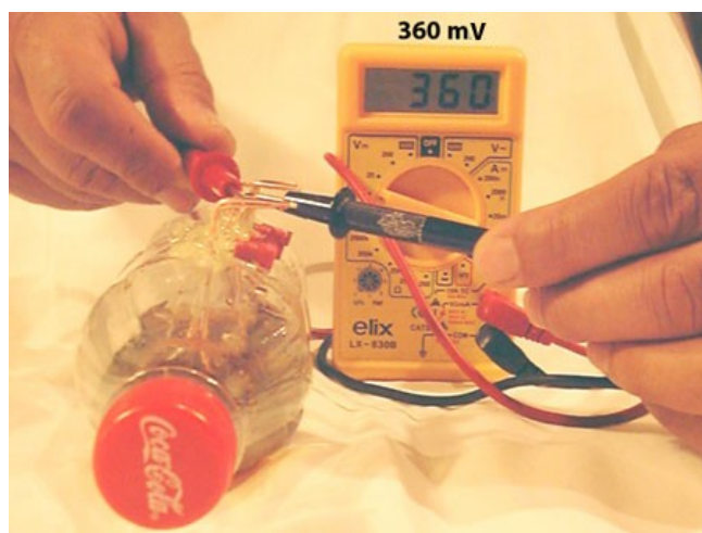
This simple cola bottle plasma reactor contains all essential conditions for a "universal" self-sustaining process.
