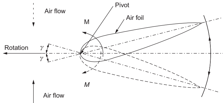
FIGURE 9.29 Air turbine using self-pitch-controlled blades for wave energy conversion. (From Kim et al., 2002, with Permission of Elsevier Science)
