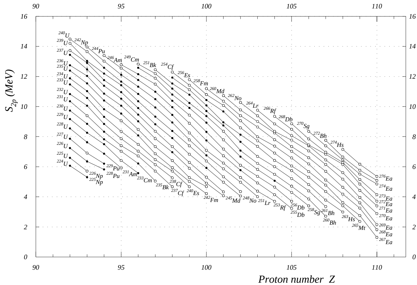
Fig. 16. Two-proton separation energies Z = 92 to 110
