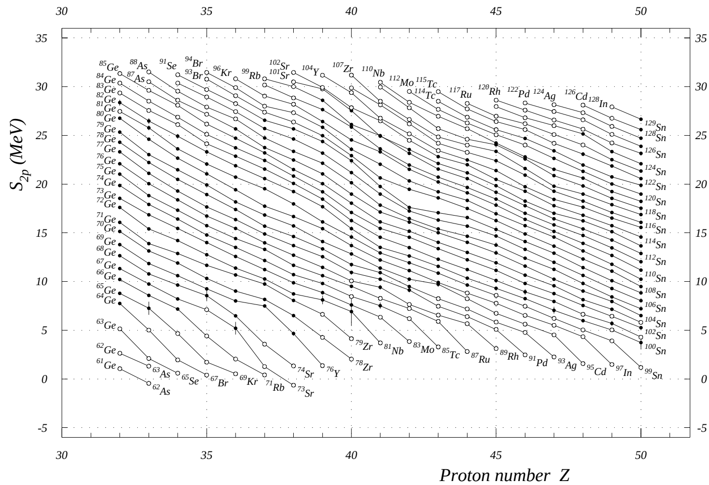
Fig. 12. Two-proton separation energies Z = 32 to 50
