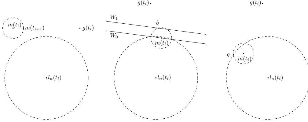
■ Figure 7 A free move. The circles with centers m(t_i) and l_n(t_i) have radii (1+\varepsilon_n)\Delta_n and r , respectively.
