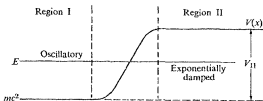
Fig. 3-4. One-dimensional potential with mc^2 > E - V_{II} > -mc^2 .
