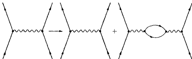
Fig. 4-27. Change in the Möller scattering amplitude.
