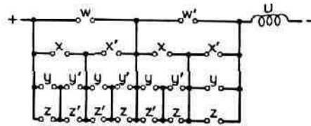
Figure 30. Series-parallel realization of selective circuit
