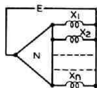
Figure 19 (left). General constant-voltage relay circuit
