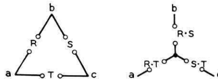
Figure 8. Delta-wye transformation
