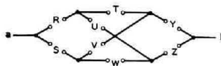
Figure 18. Nonplanar network
