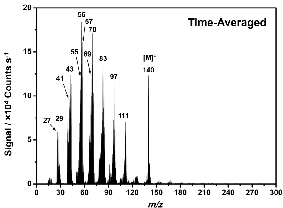
Figure 3.3: Time-averaged positive plasma ion mass spectrum of 1-decene pulsed plasma ( t_{on} = 30 \mu s , t_{off} = 10 ms , P_{on} = 15 W , and 0.1 mbar). Mass spectrometer tuning on 57 m/z mass signal.
