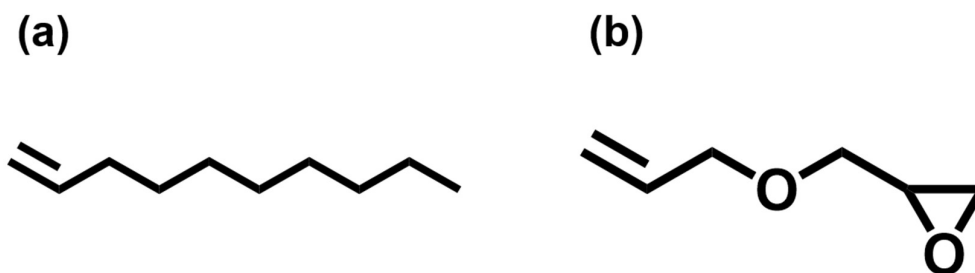
Structure 1: 1-decene (a) and allyl glycidyl ether (b) monomer structures
