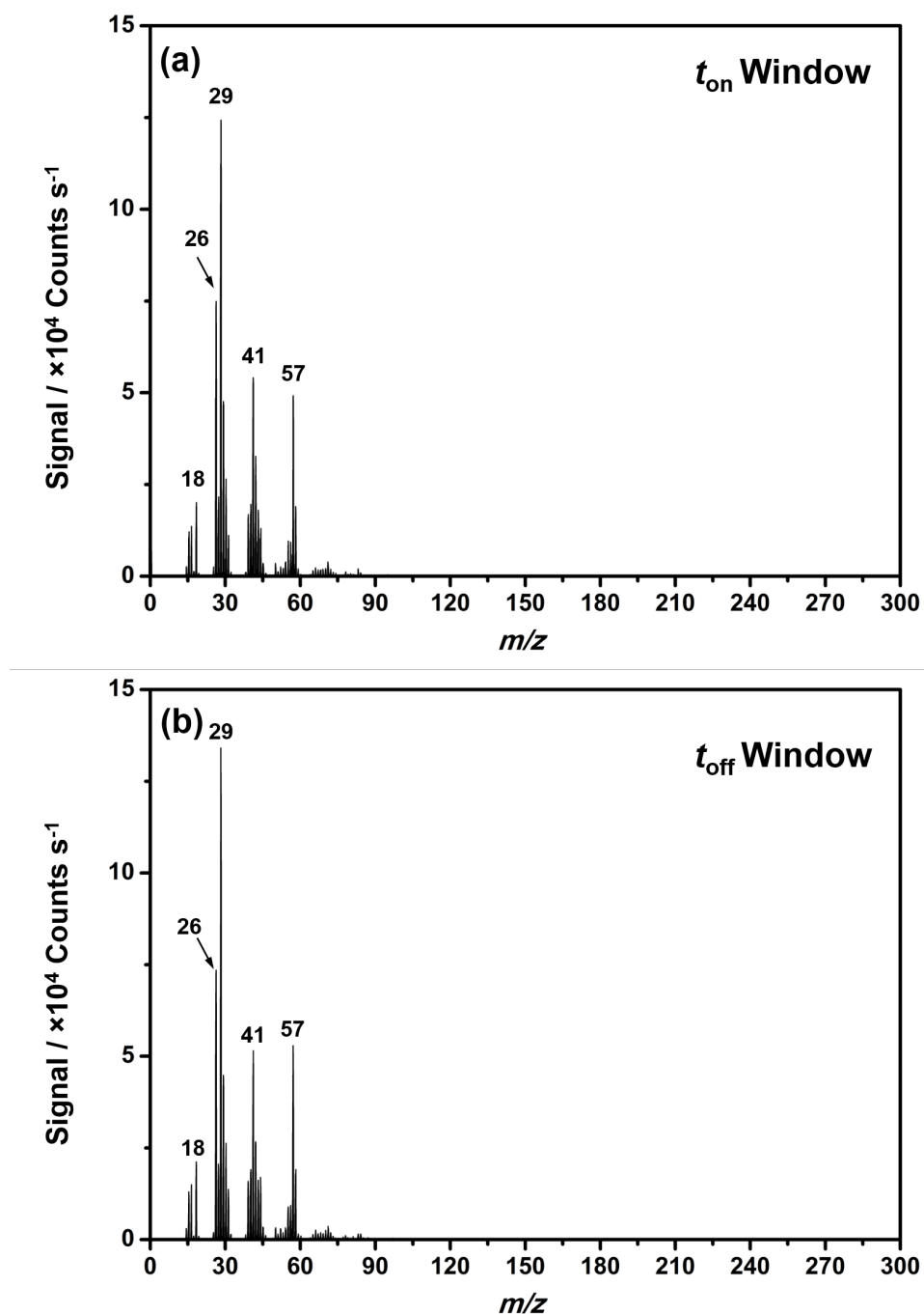
Figure 3.12: Time-resolved electron-impact ionisation mass spectra of allyl glycidyl ether pulsed plasmas (with t_{on} = 30 \mu s , t_{off} = 10 ms , P_{on} = 15 W , and 0.1 mbar ). Mass spectrometer tuning on 57 m/z mass signal.
