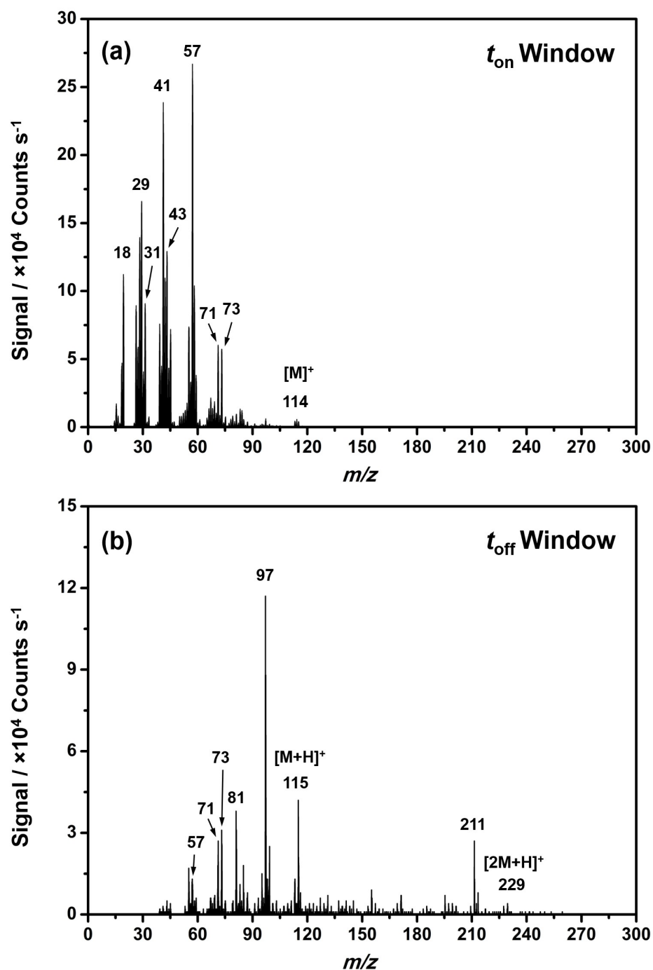
Figure 3.10: Time-resolved positive plasma ion mass spectra of allyl glycidyl ether pulsed plasma ( t_{\text{on}} = 30 \mu\text{s} , t_{\text{off}} = 10 \text{ ms} , P_{\text{on}} = 15 \text{ W} , and 0.1 \text{ mbar} ). Mass spectrometer tuning on 57 \text{ } m/z mass signal.
