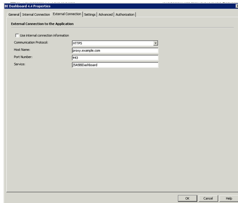
Figure 7.8 External Connection Tab for BI Dashboard Properties
