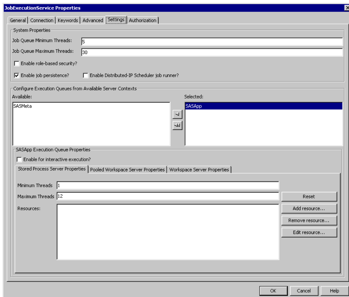
Figure 2.1 Job Execution Service Settings
