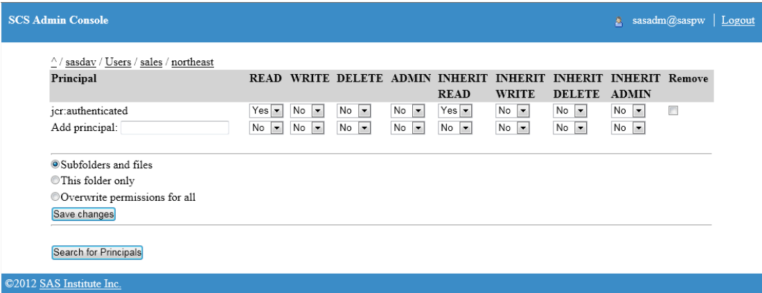
Figure 10.2 Folder Permissions in the SAS Content Server
