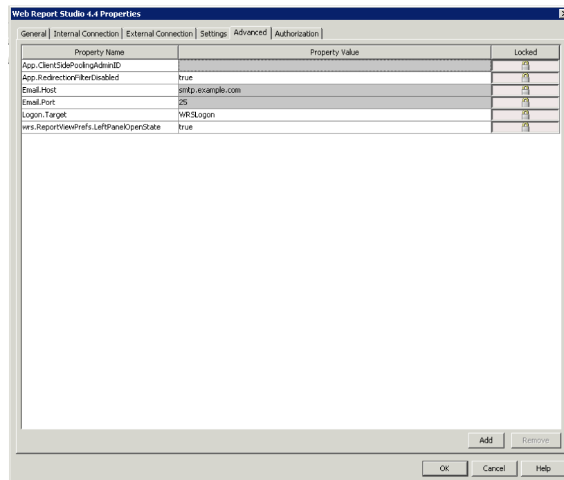
Figure 7.3 Advanced Tab for SAS Web Report Studio 4.4 Properties
