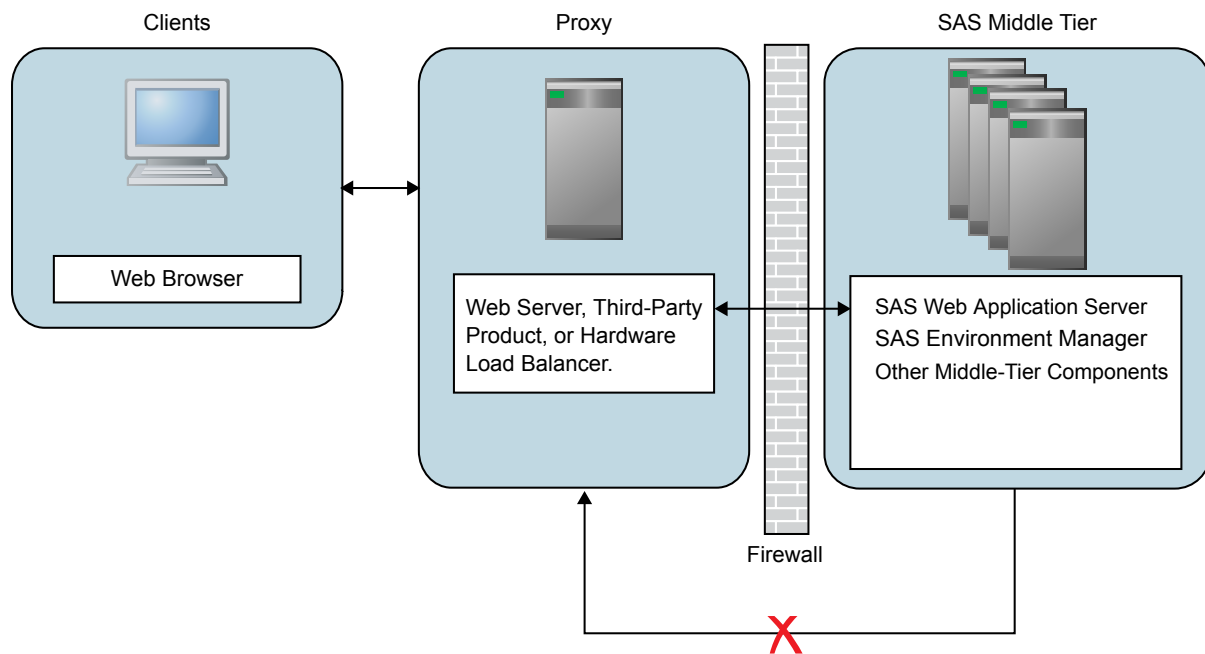
Figure 7.6 Network Topology with a Firewall
