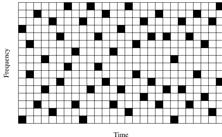
Figure 3.25 An illustration of a scheme that uses only a fixed part of the bandwidth at every time. Here, one small square denotes a single sub-carrier within one OFDM block. The time-axis indexes the different OFDM blocks; the frequency-axis indexes the different sub-carriers.
