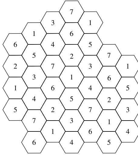
Figure 4.2 A hexagonal arrangements of cells and a possible reuse pattern of channels 1 through 7 with the condition that a channel cannot be used in one concentric ring of cells around the cell using it. The frequency reuse factor is 1/7 .
