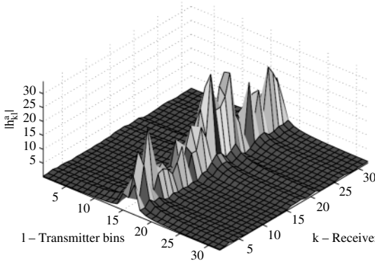
(c) 60° spread at transmitter, 60° spread at receiver
