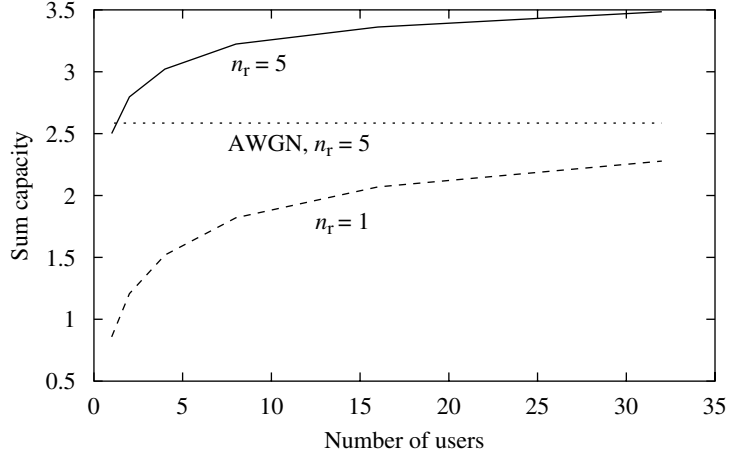
Figure 10.9 Sum capacities of the uplink Rayleigh fading channel with n_r the number of receive antennas, for n_r = 1, 5 . Here SNR = 1 (0 dB) and the Rayleigh fading channel is \mathbf{h} \sim \mathcal{CN}(0, \mathbf{I}_{n_r}) . Also plotted for comparison is the corresponding performance for the uplink AWGN channel with n_r = 5 and SNR = 5 (7 dB).
