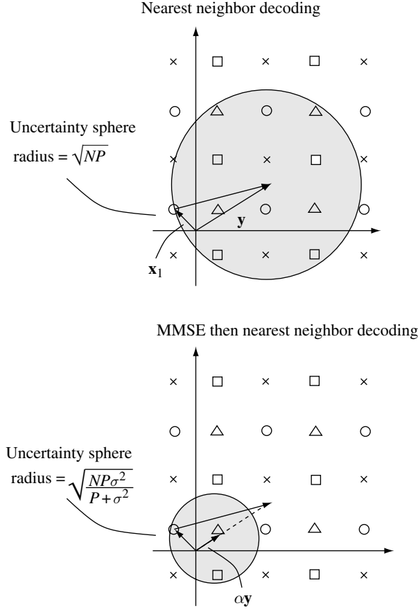
Figure 10.22 MMSE decoding yields a much smaller uncertainty sphere than does nearest neighbor decoding.
