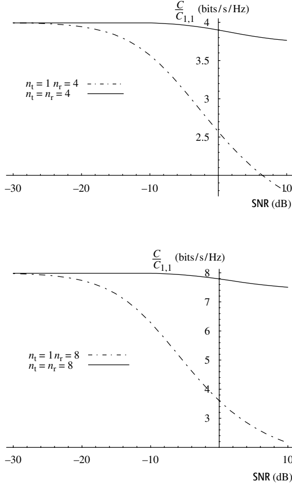
Figure 8.3 Low SNR capacities. Upper: a 1 by 4 and a 4 by 4 channel. Lower: a 1 by 8 and a 8 by 8 channel. Capacity is a fraction of the 1 by 1 channel in each case.
