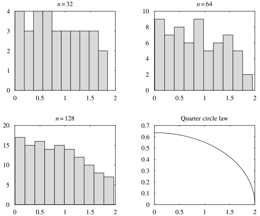
Figure 8.4 Convergence of the empirical singular value distribution of \mathbf{H}/\sqrt{n} . For each n , a single random realization of \mathbf{H}/\sqrt{n} is generated and the empirical distribution (histogram) of the singular values is plotted. We see that as n grows, the histogram converges to the quarter circle law.
