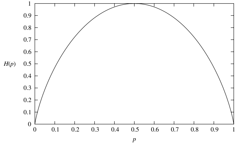
Figure B.3 The binary entropy function.
