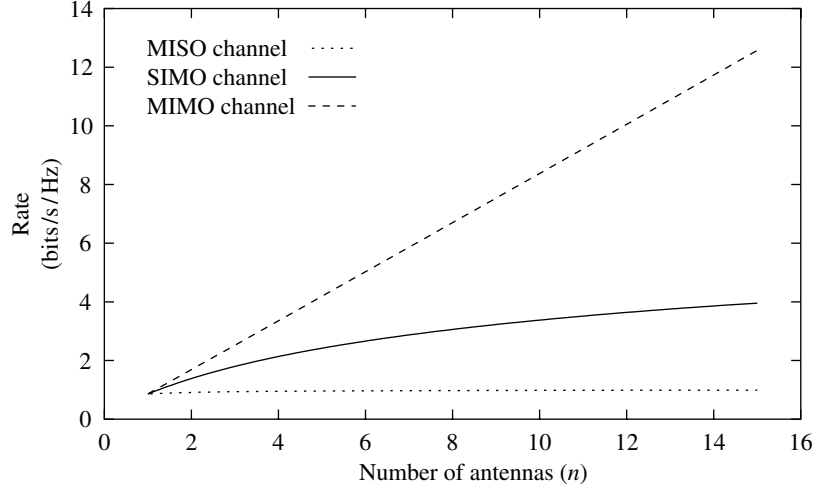
Figure 8.6 Capacities of the n by 1 MISO channel, 1 by n SIMO channel and the n by n MIMO channel as a function of n , for \text{SNR} = 0 dB
