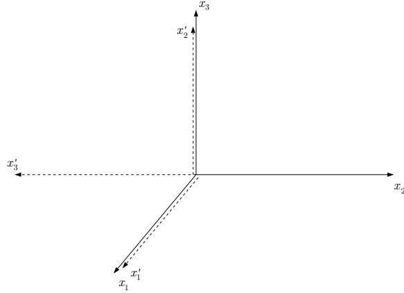
Figure 1.31: Rotation of 90^\circ about x_1 axis.
