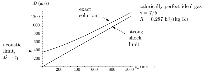
Figure 3.13: Shock speed versus piston velocity for calorically perfect ideal air.
