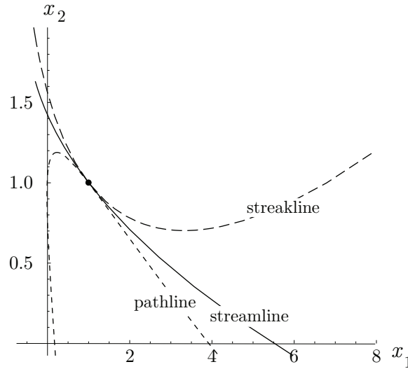
Figure 1.9: Streamline, pathlines, and streaklines for unsteady flow of example problem.
