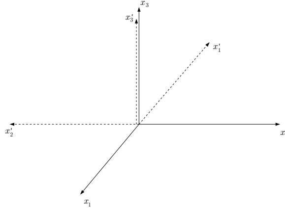
Figure 1.29: Rotation of 180^\circ about x_3 axis.
