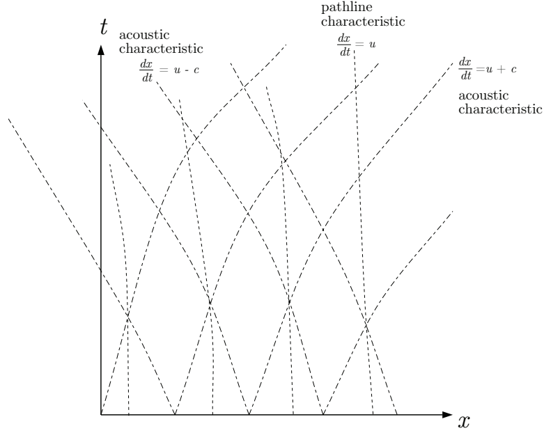
Figure 3.19: x - t diagram showing characteristics for pathlines dx/dt = u and acoustic waves dx/dt = u \pm c .
