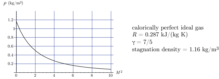
Figure 3.4: Static density versus Mach number squared.
