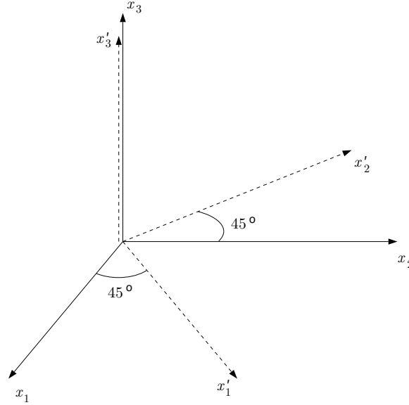
Figure 1.33: Rotation of 45^\circ about x_3 axis.
