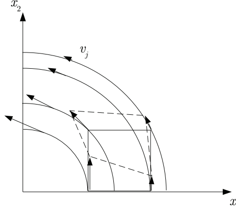
Figure 1.18: Sketch of ideal irrotational vortex.
