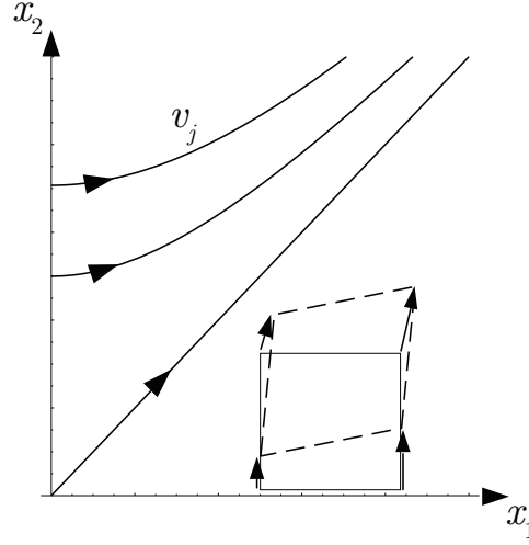
Figure 1.16: Sketch of pure shearing flow.
