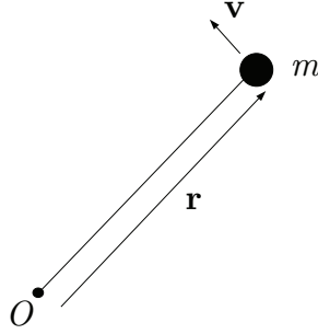
Figure 1.24: Sketch of particle of mass m velocity \mathbf{v} rotating about an axis centered at point O , with radial distance vector \mathbf{r} .
