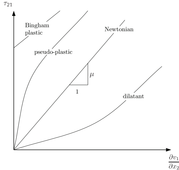
Figure 1.28: Variation of viscous stress with strain rate for typical fluids.
