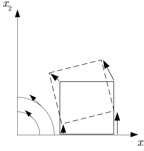
Figure 1.14: Sketch of pure rigid body rotation.
