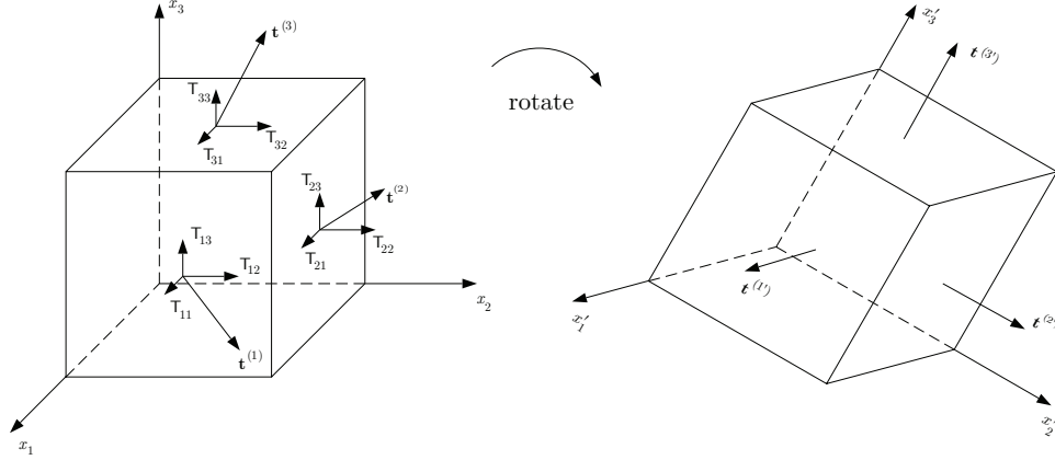
Figure 1.5: Sample Cartesian element which is rotated so that its faces have vectors which are aligned with the unit normals associated with the faces of the element.
