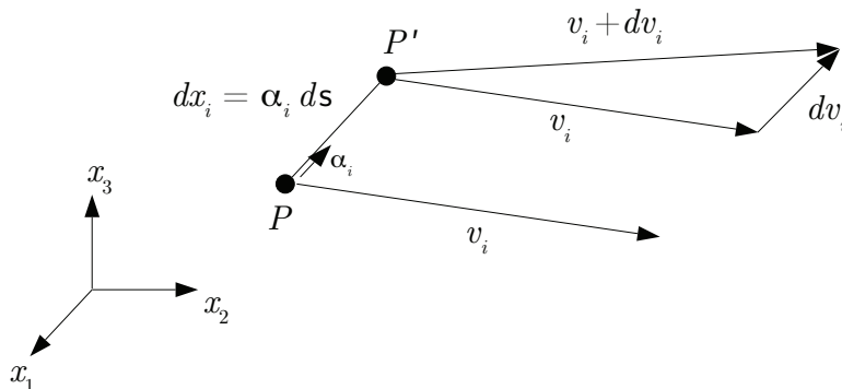
Figure 1.10: Sketch of fluid particle P in motion with velocity v_i and nearby neighbor particle P' with velocity v_i + dv_i .
