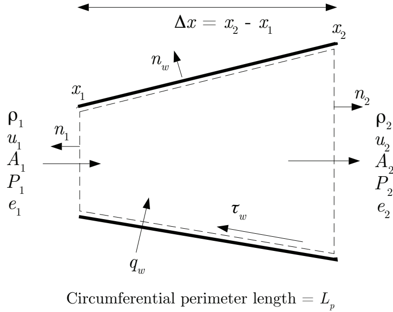
Figure 3.1: Control volume sketch for one-dimensional compressible flow with area change, heat transfer, and wall friction.
