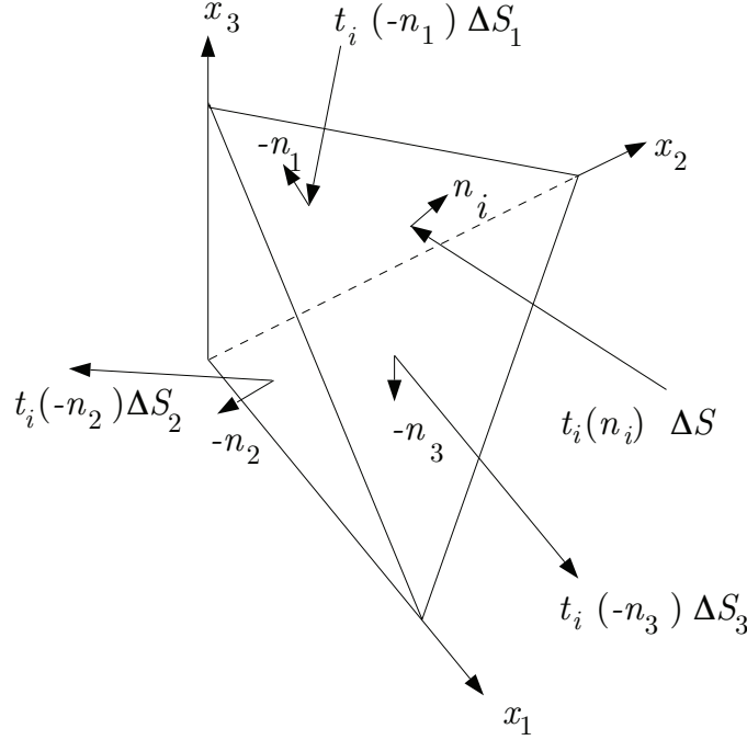
Figure 1.23: Sketch of tetrahedral element for stress analysis on an arbitrary plane.
