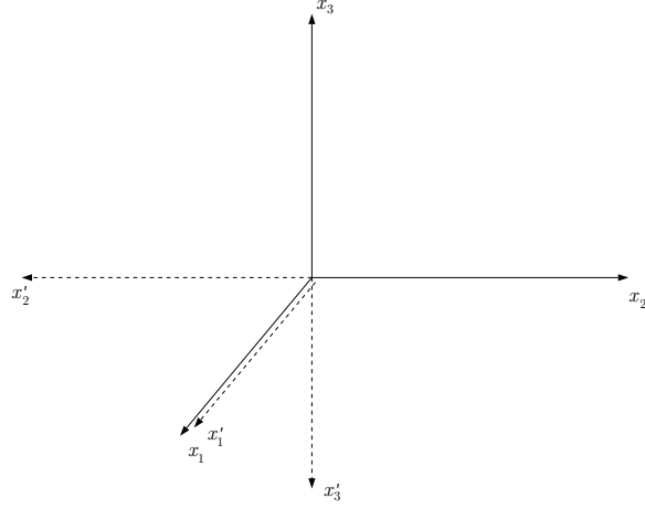
Figure 1.30: Rotation of 180^\circ about x_1 axis.
