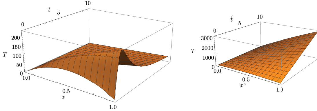
Figure 1.8: Eulerian plot T(x, t) and Lagrangian plot of T(x^o, \hat{t}) for example problem originally described in Lagrangian coordinates, with \tau = 1 , L = 1 , T_o = 300 .
