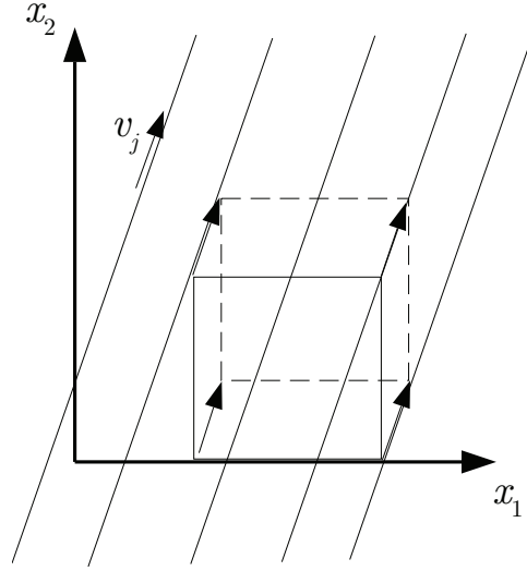
Figure 1.13: Sketch of uniform flow.
