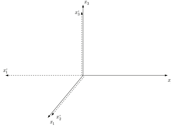
Figure 1.32: Rotation of 90^\circ about x_3 axis.
