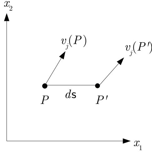
Figure 1.11: Sketch of fluid particle P in motion with velocity v_j(P) and nearby neighbor particle P' with velocity v_j(P') .
