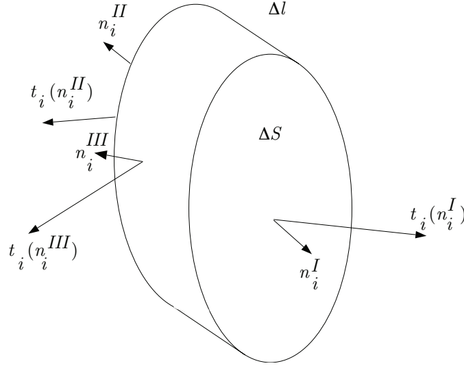
Figure 1.22: Sketch of pillbox element for stress analysis.
