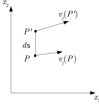
Figure 1.12: Sketch of fluid particle P in motion with velocity v_i(P) and nearby neighbor particle P' with velocity v_i(P') .
