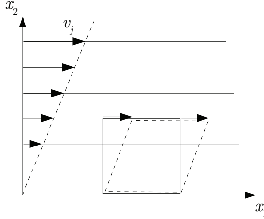
Figure 1.17: Sketch of Couette flow.
