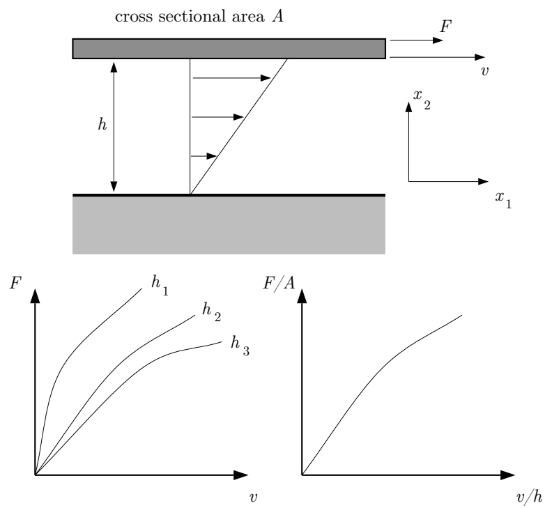
Figure 1.27: Sketch of simple Couette flow experiment with measurements of stress versus strain rate.
