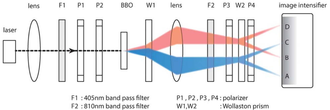
Fig. 3. Experimental equipment to verify the Bohmian trajectory. Laser (405 nm) light passed through filter F1 and polarizing plate P1 and entered the Type-II BBO crystal. Photon pairs passed through the lens after their relative angles were expanded with the Wollaston prism W1. The light was again separated into two light waves by the Wollaston prism W2 and imaged onto the image intensifier. The paths of signal and idler lights were shown by red and blue lines, respectively.
