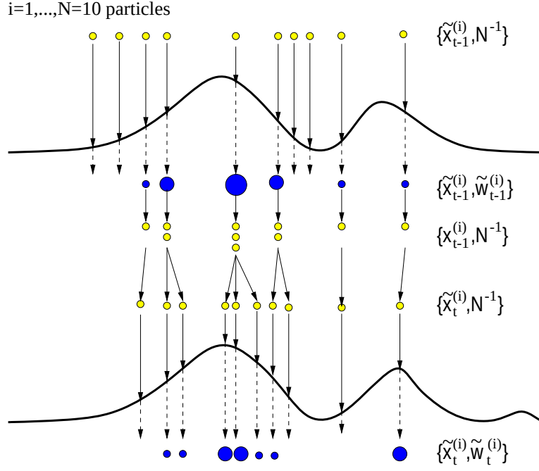
Figure 1.1. In this example, the bootstrap filter starts at time t - 1 with an unweighted measure \{\tilde{\mathbf{x}}_{t-1}^{(i)}, N^{-1}\} , which provides an approximation of p(\mathbf{x}_{t-1}|\mathbf{y}_{1:t-2}) . For each particle we compute the importance weights using the information at time t - 1 . This results in the weighted measure \{\tilde{\mathbf{x}}_{t-1}^{(i)}, \tilde{w}_{t-1}^{(i)}\} , which yields an approximation p(\mathbf{x}_{t-1}|\mathbf{y}_{1:t-1}) . Subsequently, the resampling step selects only the fittest particles to obtain the unweighted measure \{\tilde{\mathbf{x}}_{t-1}^{(i)}, N^{-1}\} , which is still an approximation of p(\mathbf{x}_{t-1}|\mathbf{y}_{1:t-1}) . Finally, the sampling (prediction) step introduces variety, resulting in the measure \{\tilde{\mathbf{x}}_t^{(i)}, N^{-1}\} , which is an approximation of p(\mathbf{x}_t|\mathbf{y}_{1:t-1}) .
