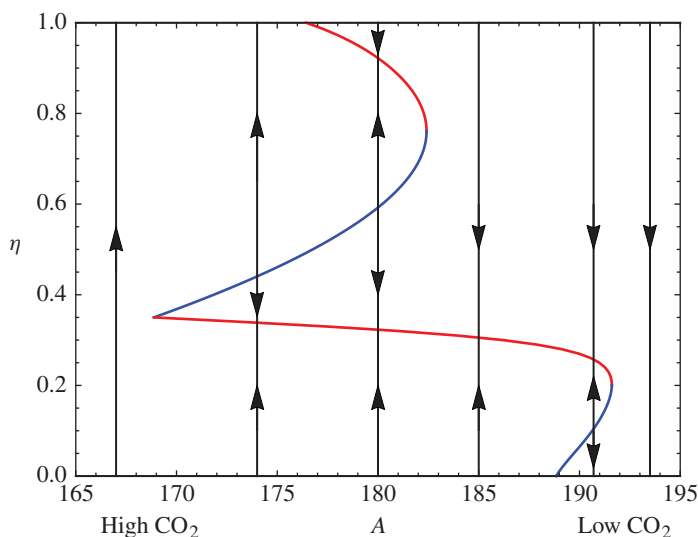
Figure 8. Dynamic bifurcation diagram for the Jormungand model. Arrows indicate the movement of the ice line as solutions to system (12) evolve, with albedo function \alpha_J(y, \eta) . Red: Stable equilibrium, blue: Unstable equilibrium.
