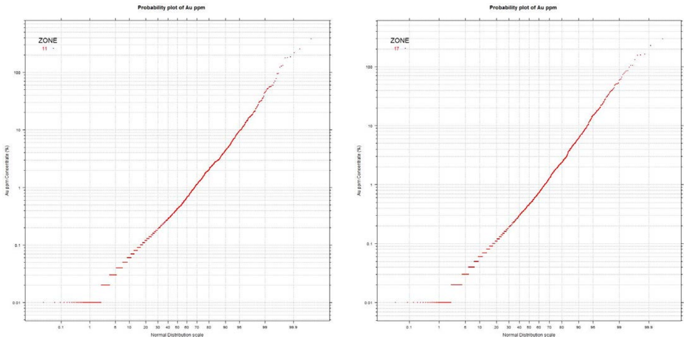
Figure 14-33 Examples of Probability plots on raw assays – Domains 1 and 7
