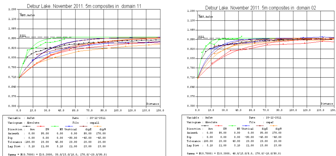
Figure 14-14 Examples of Detour Lake Correlograms of the Capped Grade of 5 metre Composites per Mineralized Domains
