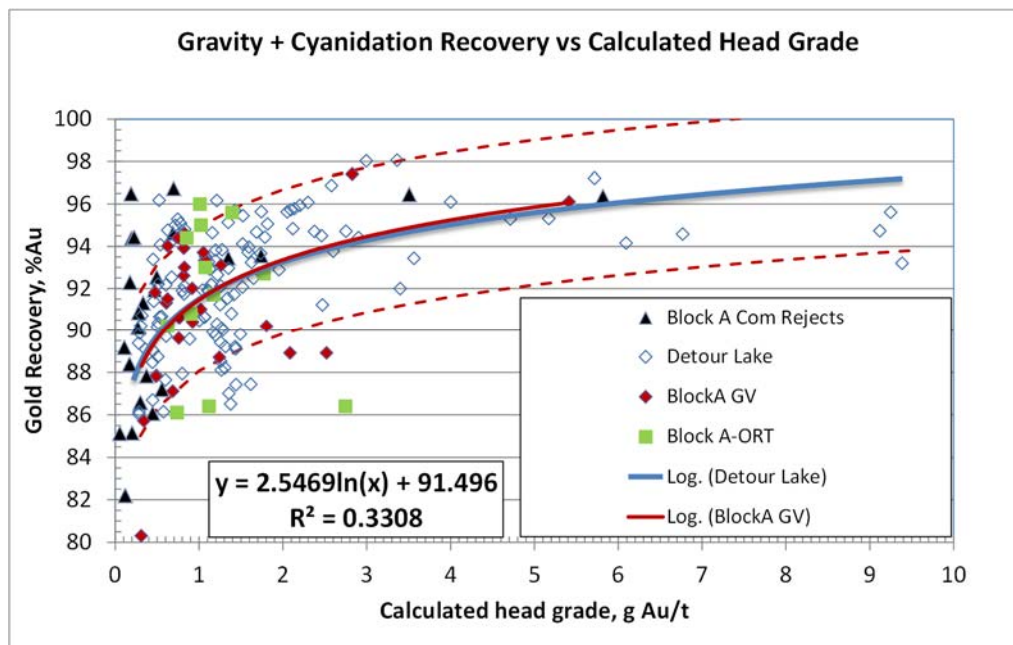
Figure 13-4 Comparison of Gravity Separation + Cyanidation Recovery Performance for Detour Lake and West Detour
