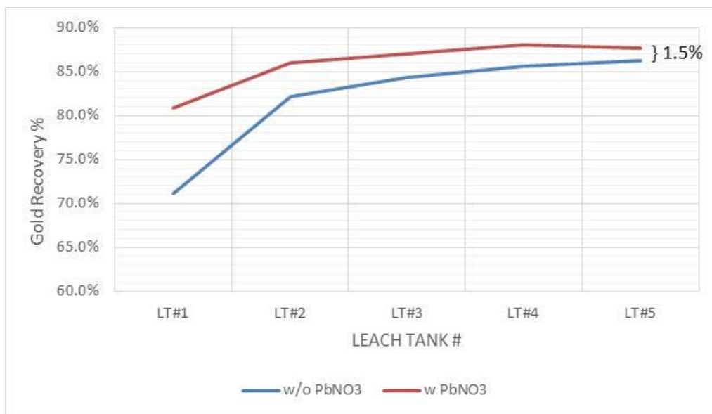
Figure 13-6 Plant Trial – Leach Kinetic Profile
