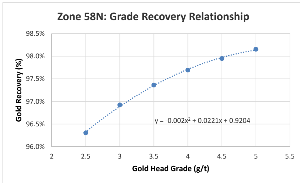
Figure 13-8 Grade Recovery Relationship
