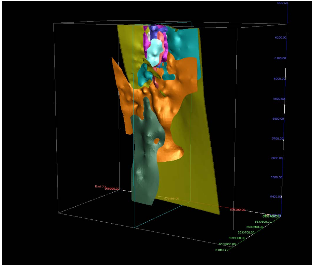
Figure 14-32 Zone 58N Deposit Isometric View of the Mineralized Domains (looking south-east)
