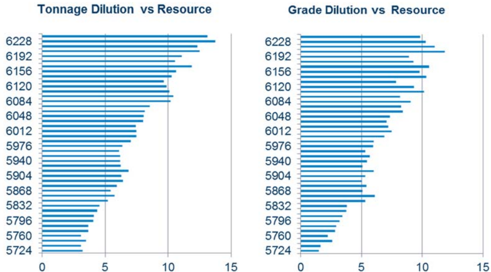
Figure 15-9 Detour Lake Pit Dilution by Bench 1
