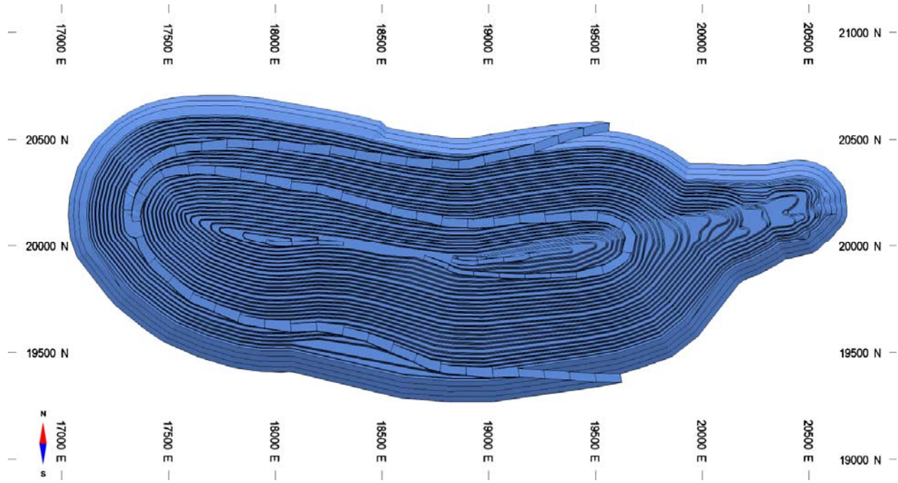
Figure 15-5 Detour Lake Ultimate Pit Design – Plan View
