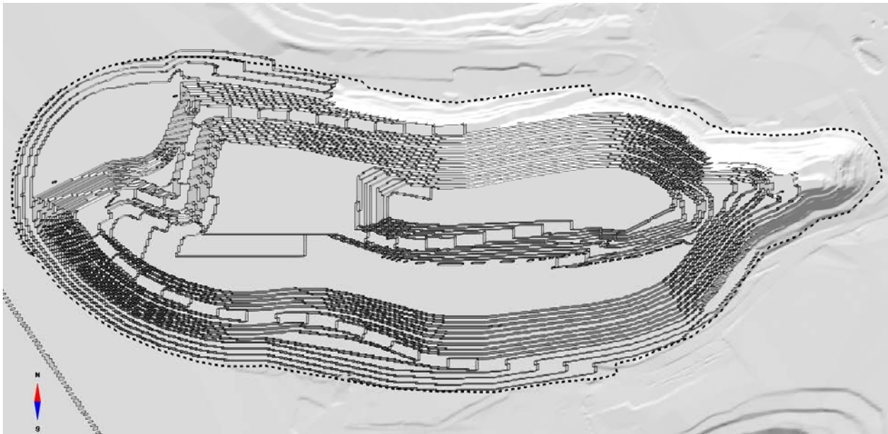
Figure 16-7 Detour Lake Pit End of Period 2028
