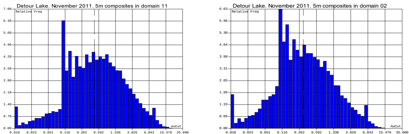
Figure 14-11 Examples of Detour Lake Histogram of 5 metre Composite Grades per Domain
