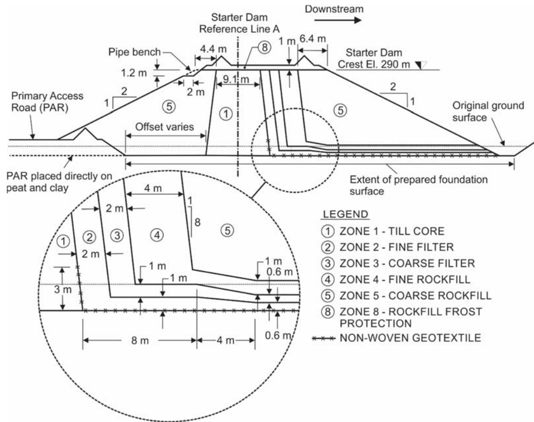
Figure 20-3 Typical Cell 2 ‘Starter Dam’ section (not to scale)
