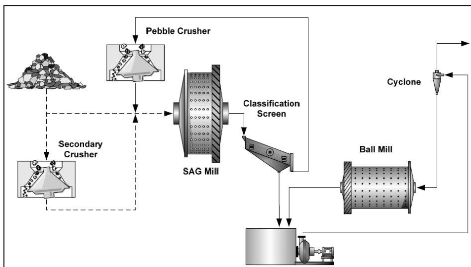
Figure 17-1 SABC Circuit
