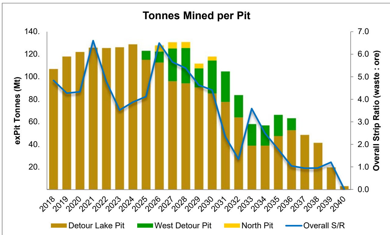
Figure 16-3 Tonnes Mined per Pit
