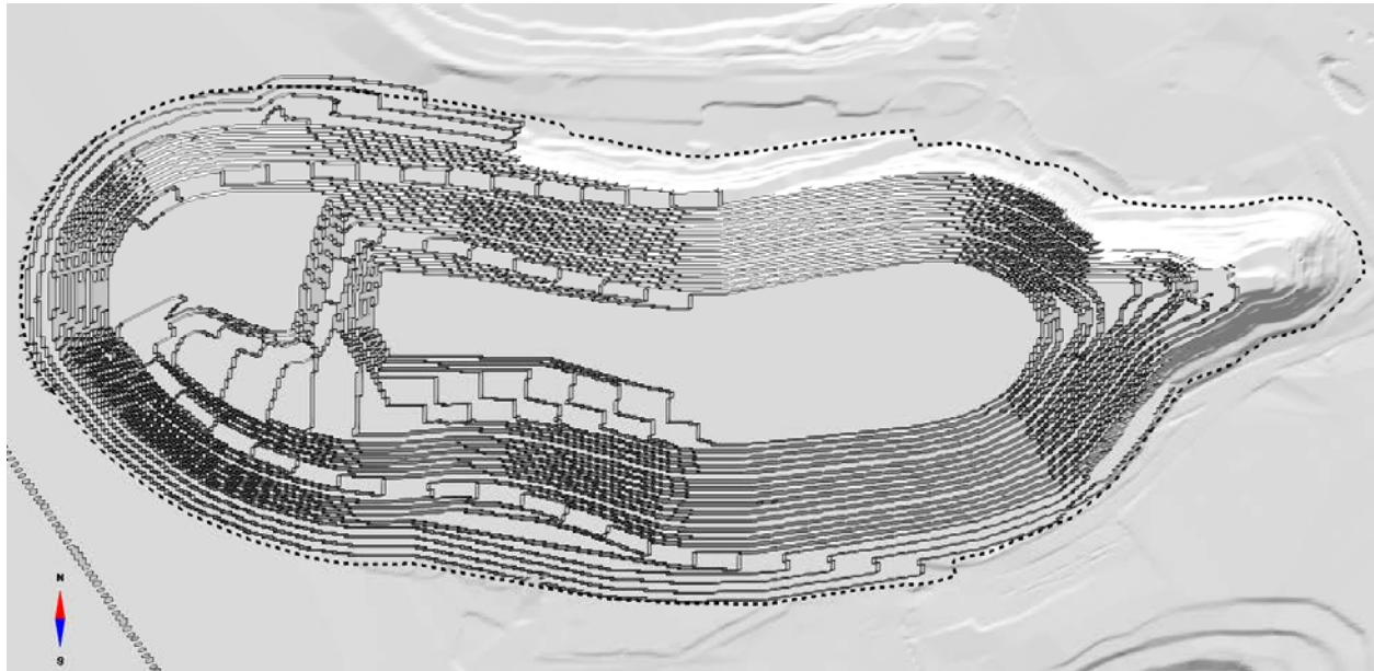
Figure 16-8 Detour Lake Pit End of Period 2031
