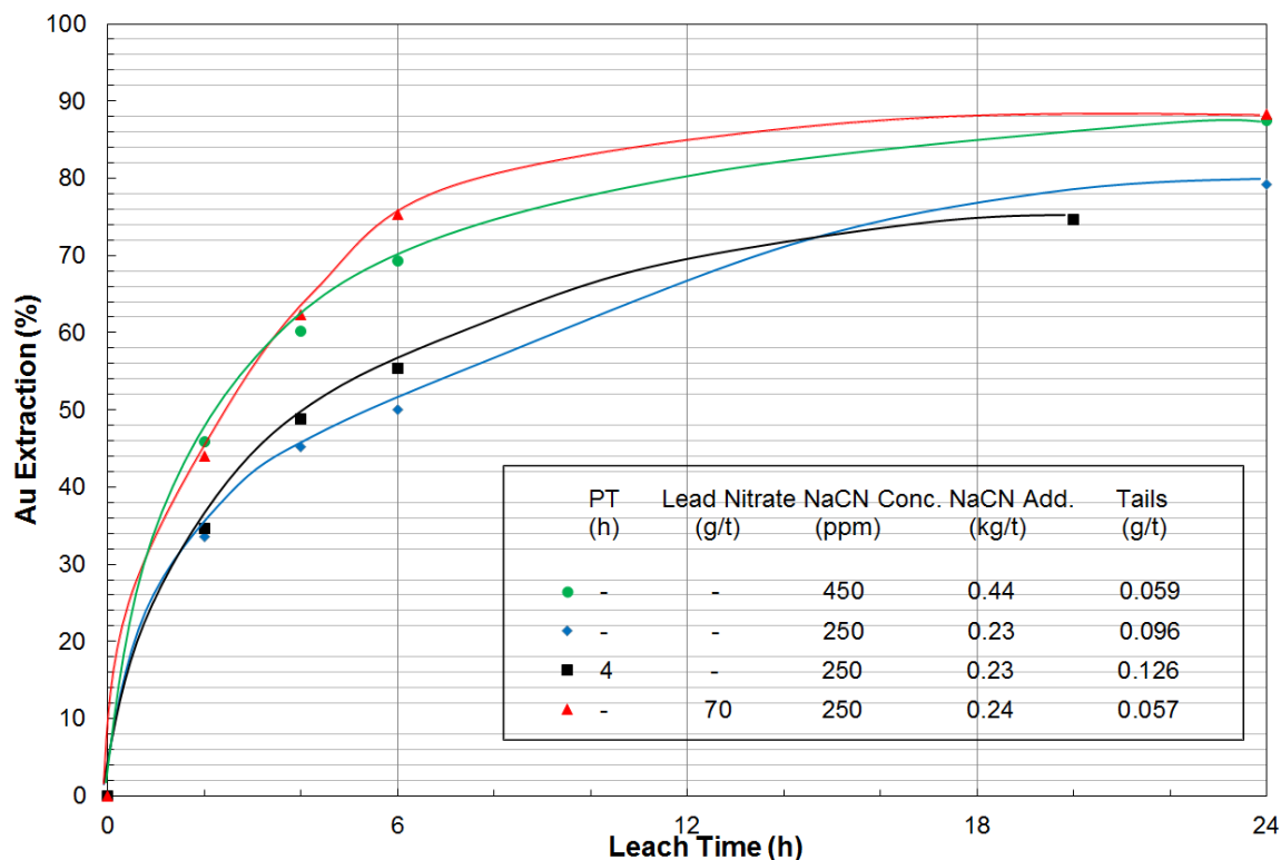
Figure 13-5 Effect of Chemical Regime on Gold Leaching Performance (recovery is post gravity recovery)
