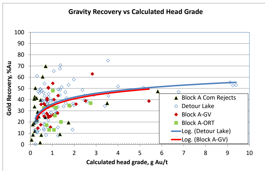
Figure 13-3 Comparison between Gravity Separation Performance for Detour Lake and West Detour GV and ORT Samples
