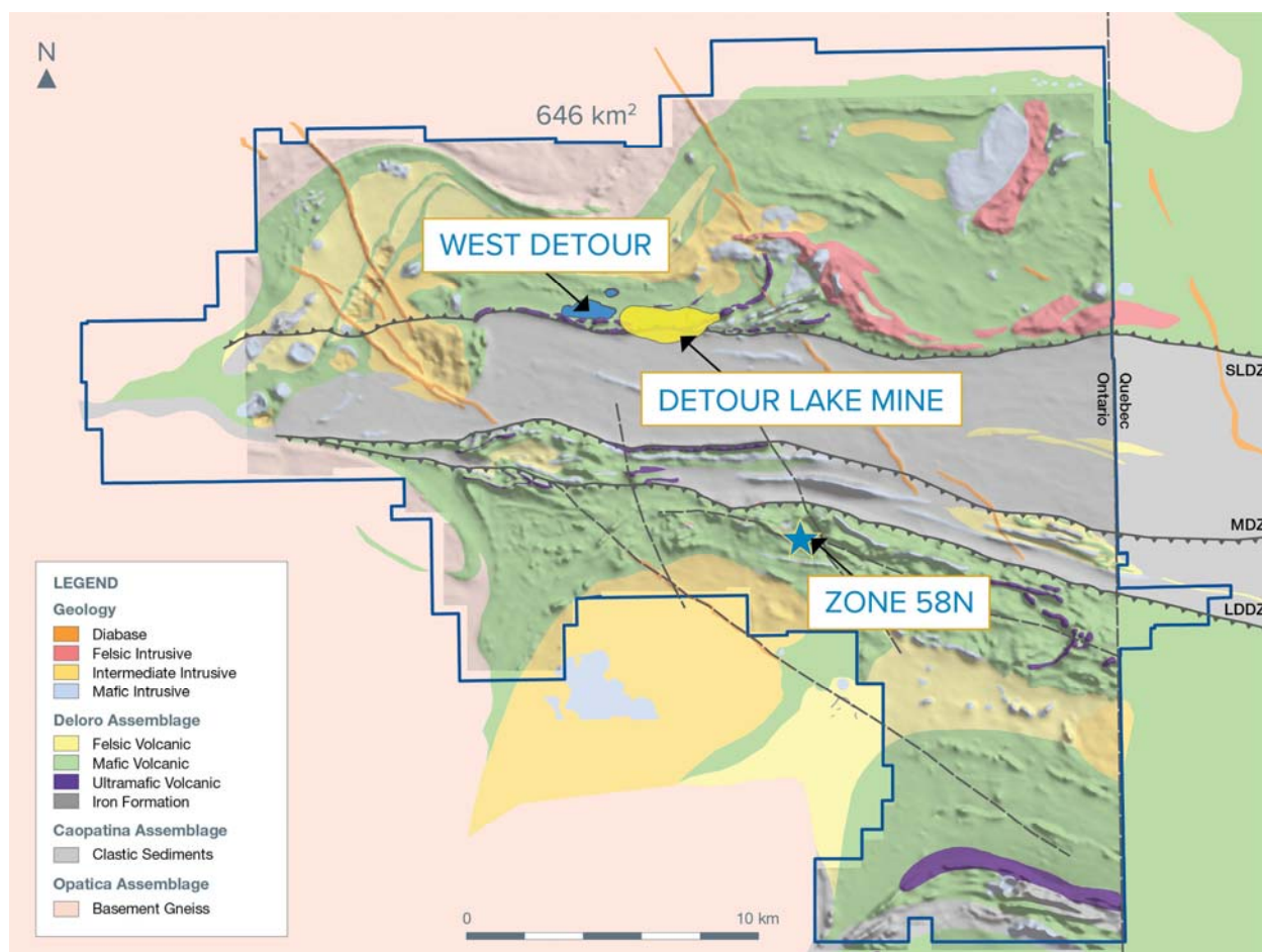
Figure 7-1 Regional Geology Map (Detour Lake Property)
