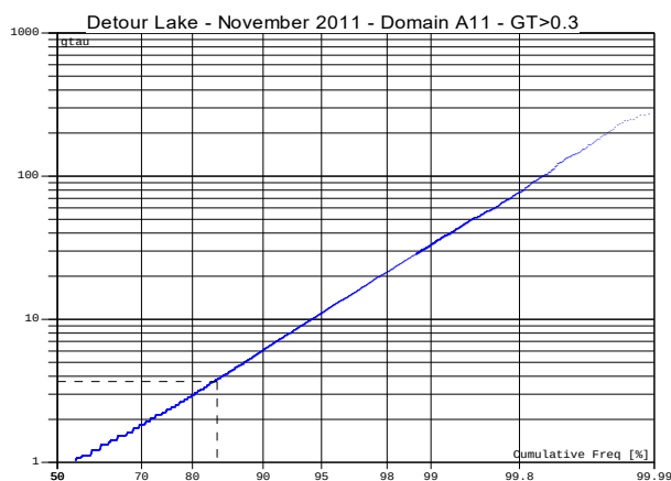
Figure 14-8 Examples of Detour Lake GT Cumulative Frequency Plots of 2011 Data in Mineralized Domains
