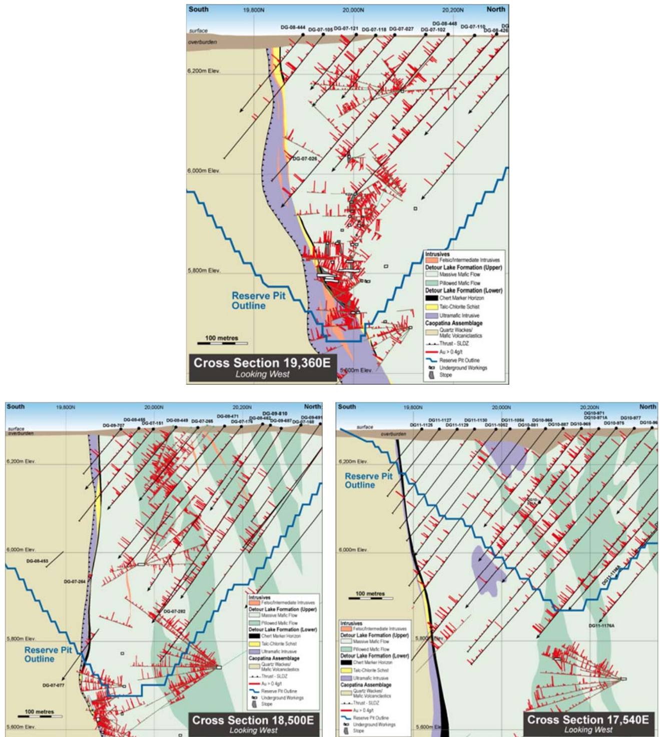
Figure 7-4 Geological Sections 19,360E (A-A'), 18,500E (B-B') and 17,540E (C-C') for Detour Lake Pit and 16,340E (D-D') for West Detour Pit
