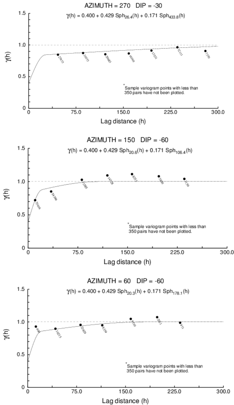
Figure 14-5 North Pit Indicator Variograms for the IK Model
