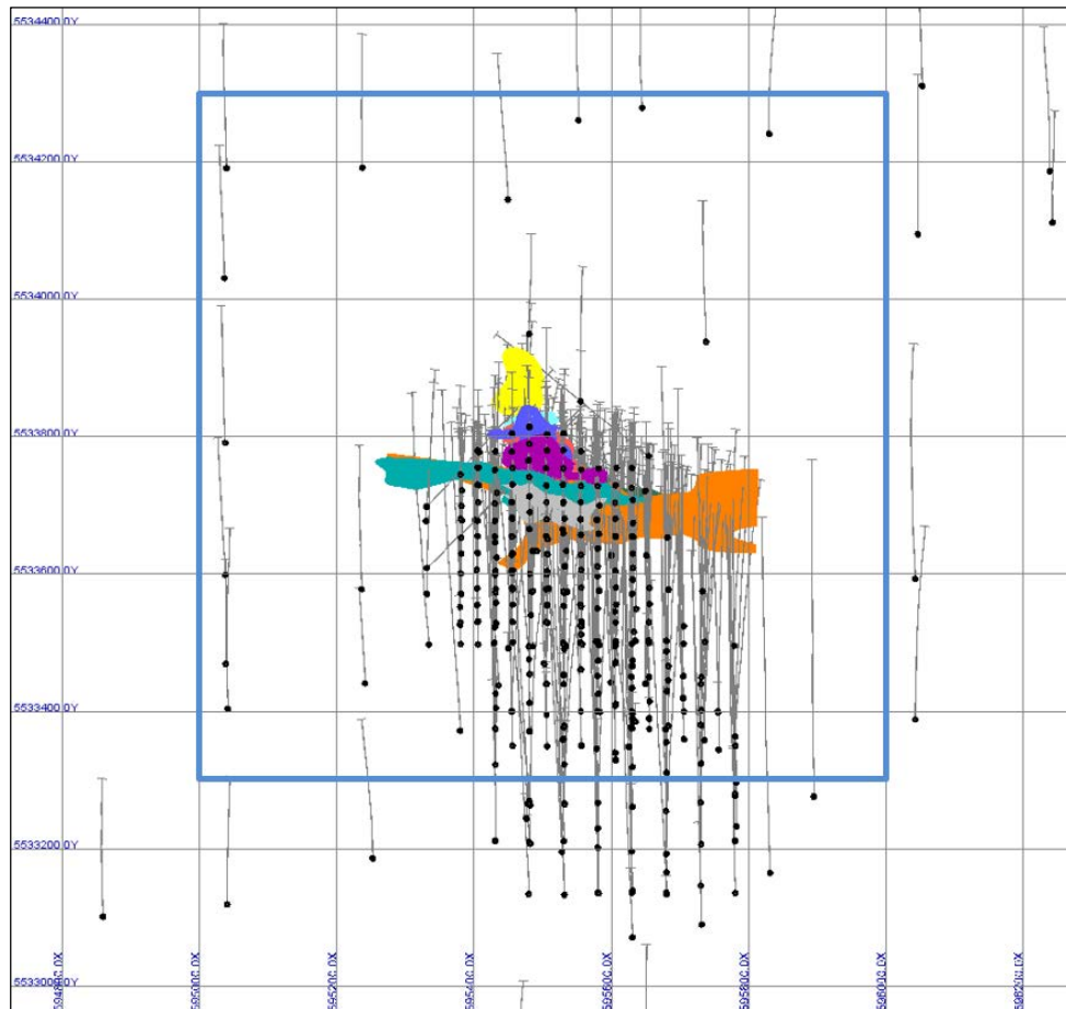
Figure 14-35 Block Model for Zone 58N - Plan View Showing Mineralized Domains and Drill Holes
