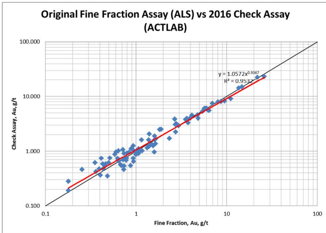
Figure 12-3 Correlation Chart of Check Assays from 2016 for Zone 58N. Black line = reference line, Red line = trend line from samples
