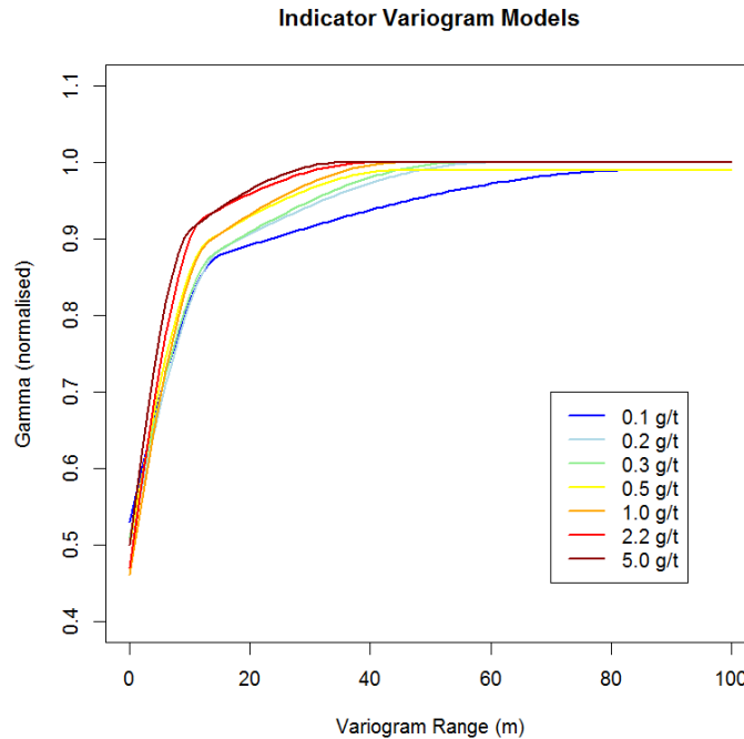
Figure 14-34 Indicator Variograms for Samples Within the 0.05 g/t Au Envelope
