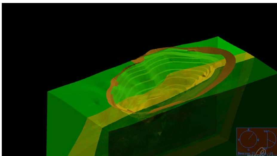
Figure 14-4 Isometric View of the North Pit Geology
