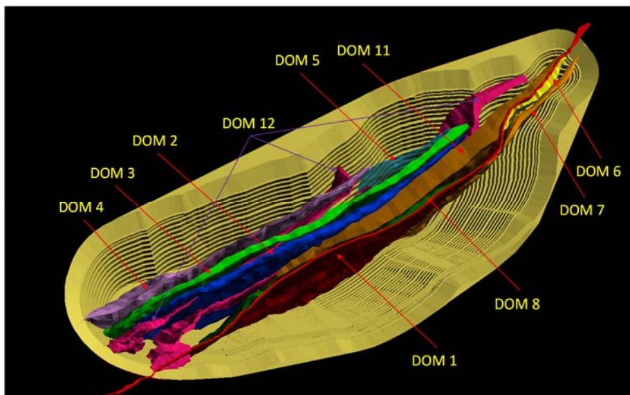
Figure 14-2 Detour Lake Isometric View of the Open Pit Showing Mineralized Domains
