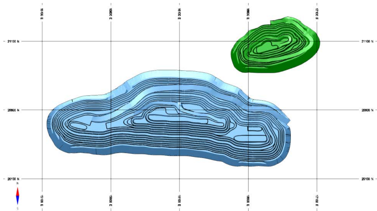
Figure 15-7 West Detour and North Pit Ultimate Pit Design – Plan View
