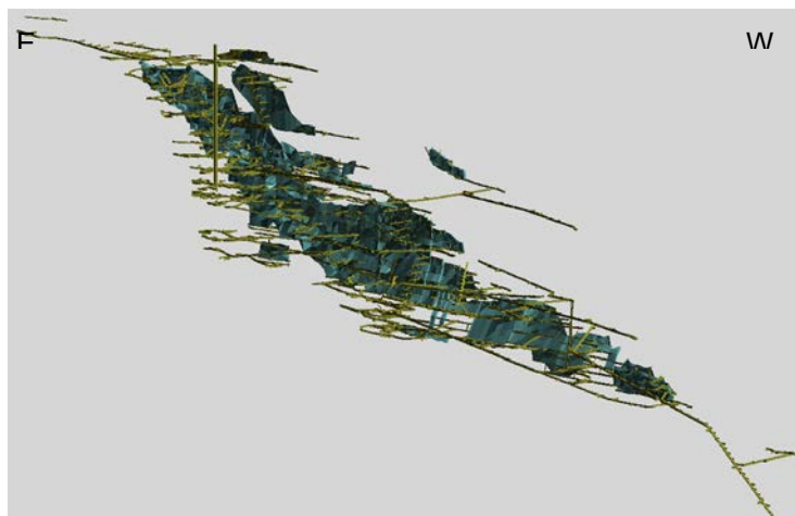
Figure 14-7 Isometric View of the Detour Lake Historical Underground Model
