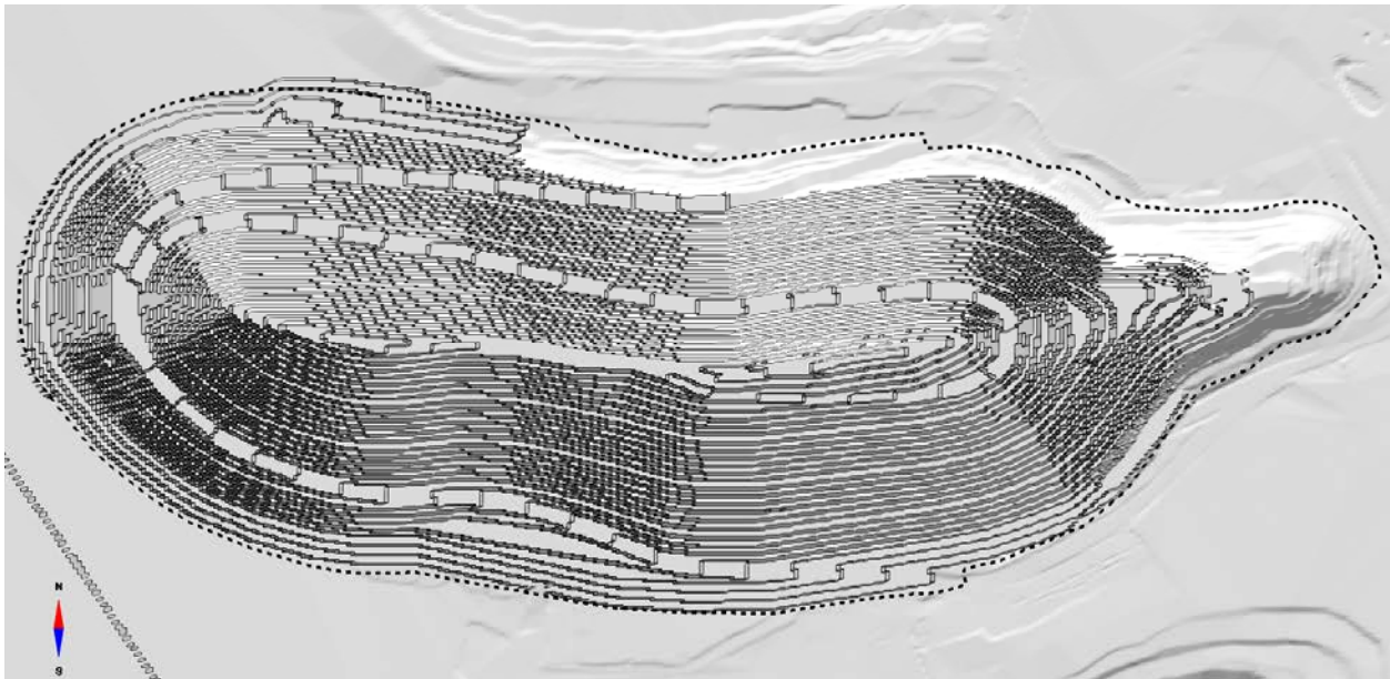
Figure 16-11 Detour Lake Pit End of Period 2040
