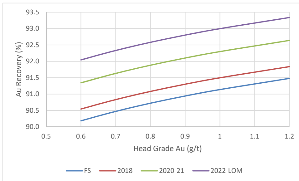
Figure 13-7 Updated Recovery Relationships (grade recovery curve)
