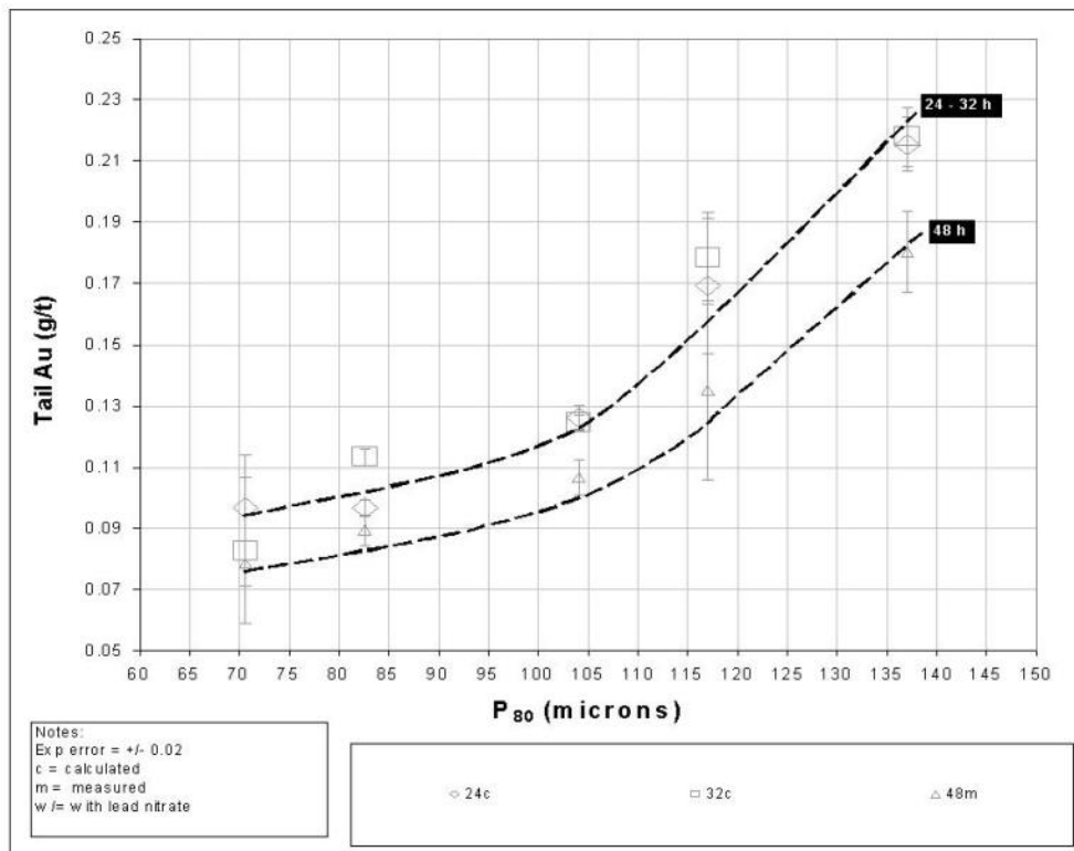
Figure 13-1 Gold in Tails (g/t) vs. P_{80}
