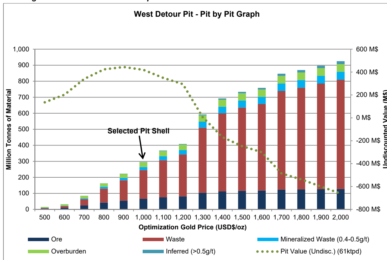
Figure 15-2 West Detour Pit Optimization Results 1
