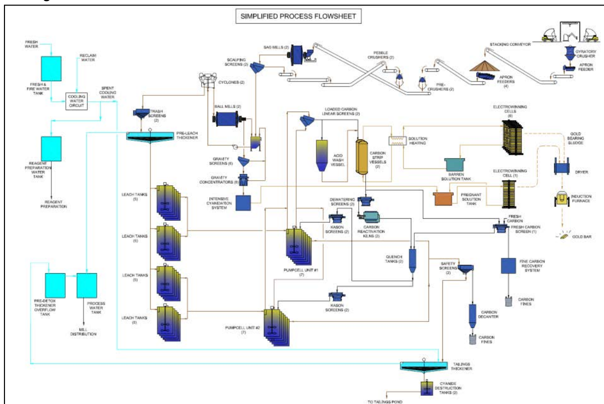
Figure 17-2 Detour Lake Process Flowsheet 1
