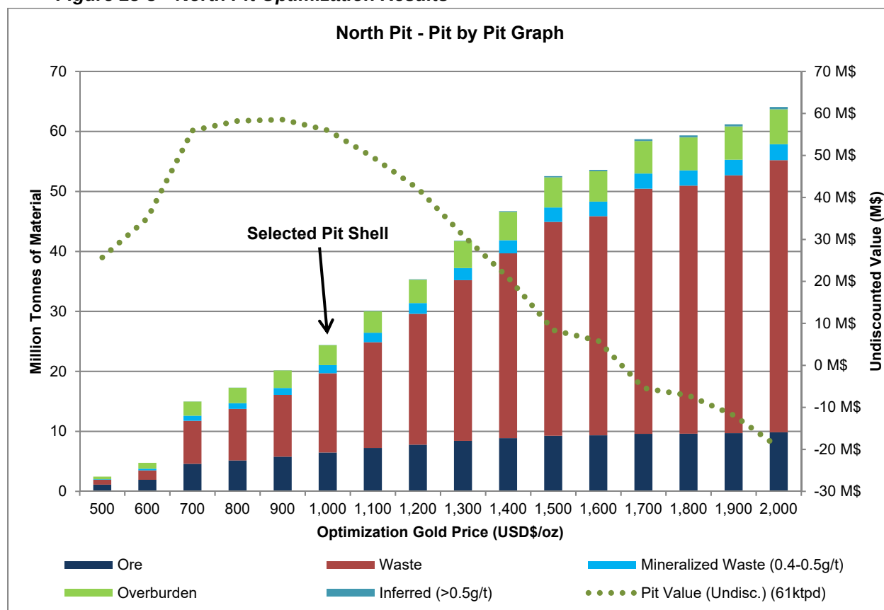
Figure 15-3 North Pit Optimization Results 1
