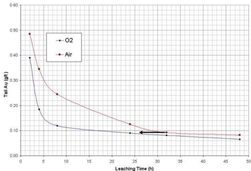
Figure 13-2 Oxygen versus Air – Gold Leaching Kinetic Comparison
