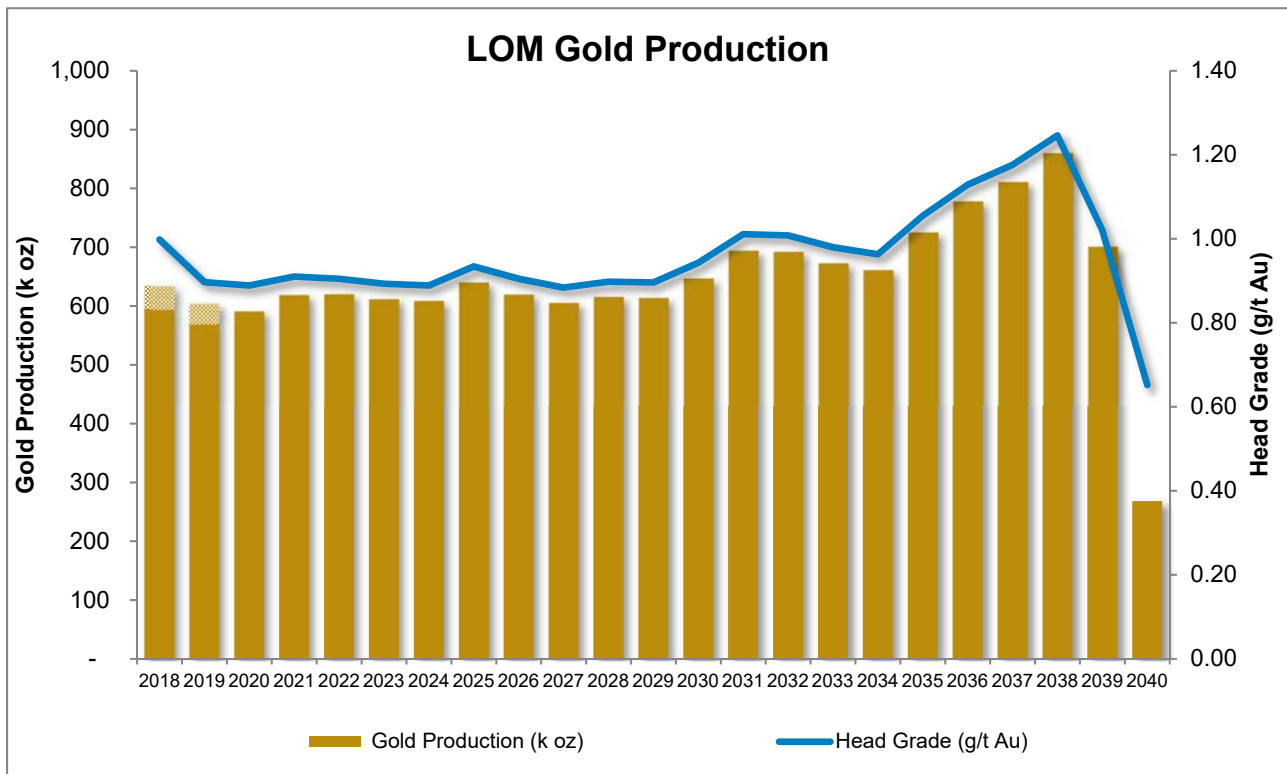
Figure 16-2 LOM Gold Production Profile
