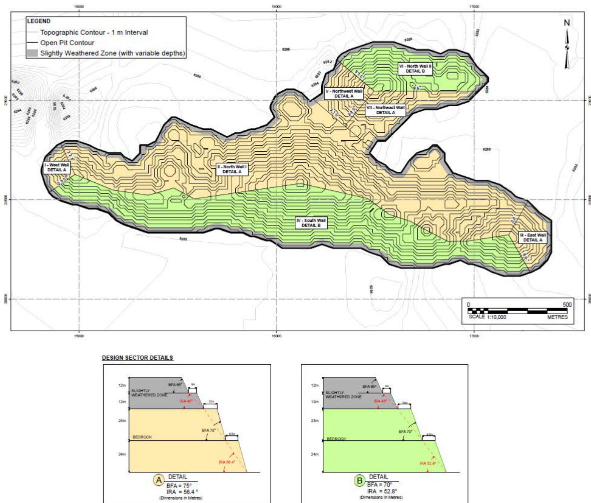
Figure 15-6 West Detour and North Pits - Pit Slope Recommendations (previous Block A pit below)
