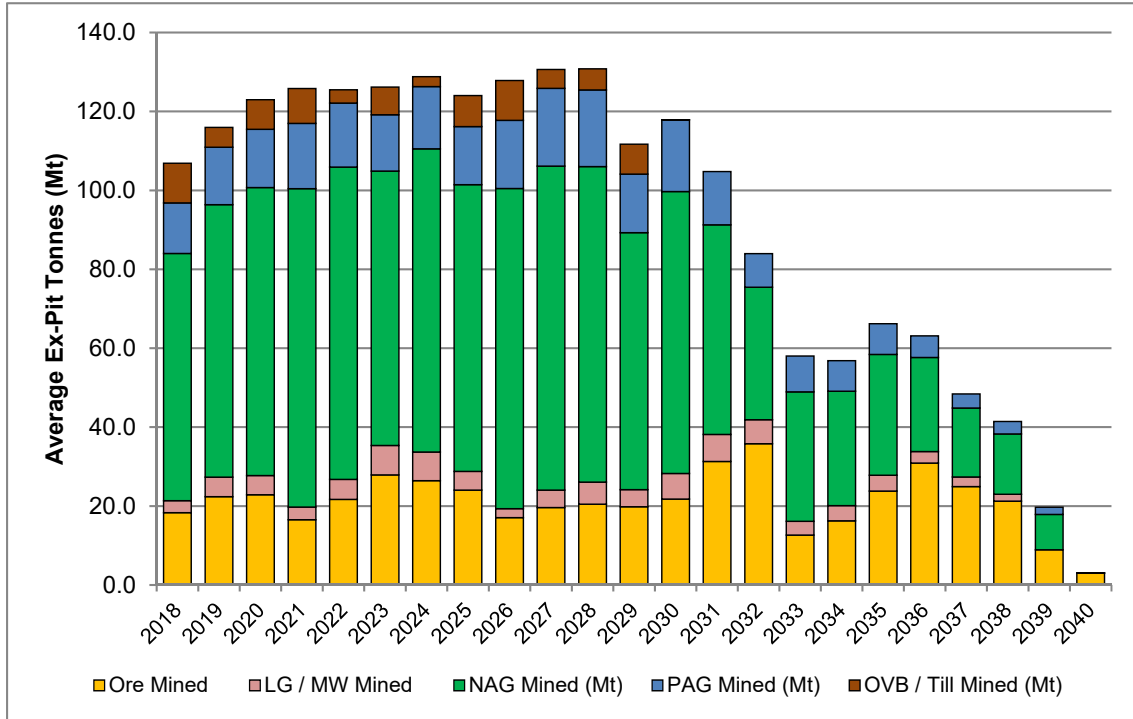
Figure 16-1 Annual Material Movement Breakdown
