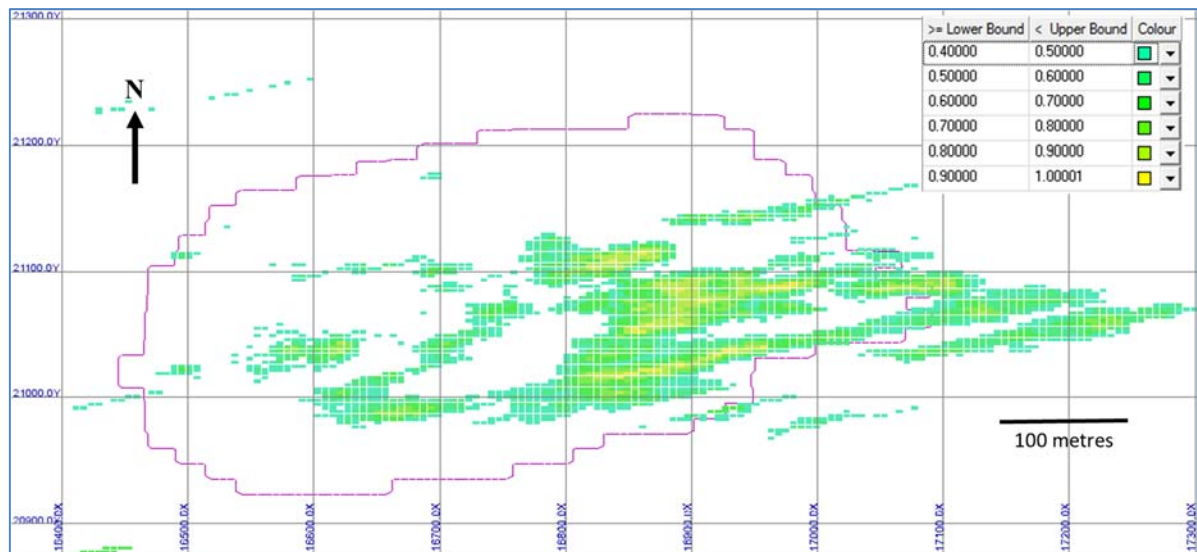
Figure 14-6 North Pit Plan View (6250EL) of Probabilities Greater than or Equal to 0.4 and Trace of Constraining Shell
