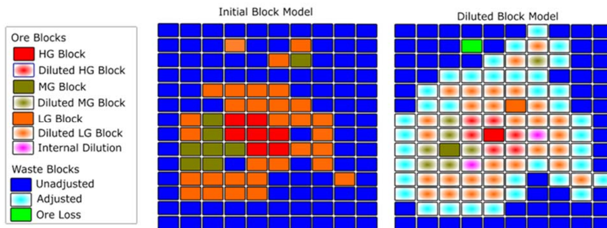
Figure 15-8 Illustration of Dilution Methodology
