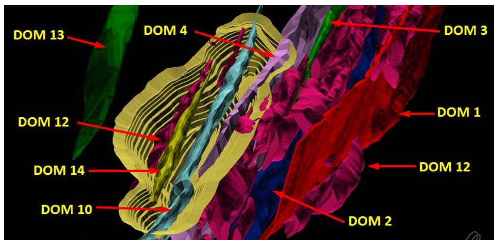
Figure 14-3 West Detour Isometric View of the Open Pit Showing Mineralized Domains
