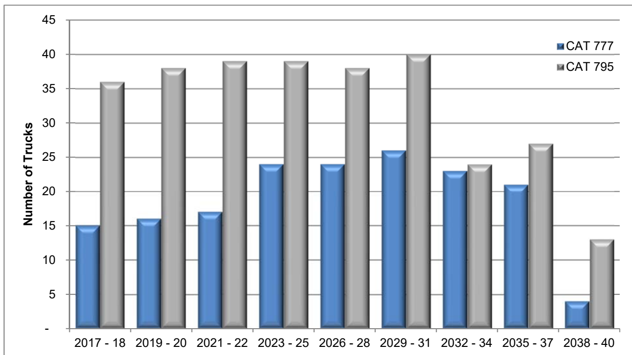
Figure 16-20 Maximum Truck Fleet Requirements per Period
