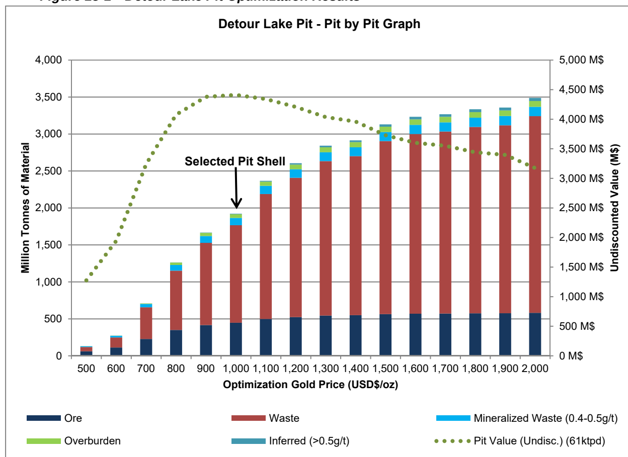
Figure 15-1 Detour Lake Pit Optimization Results 1
