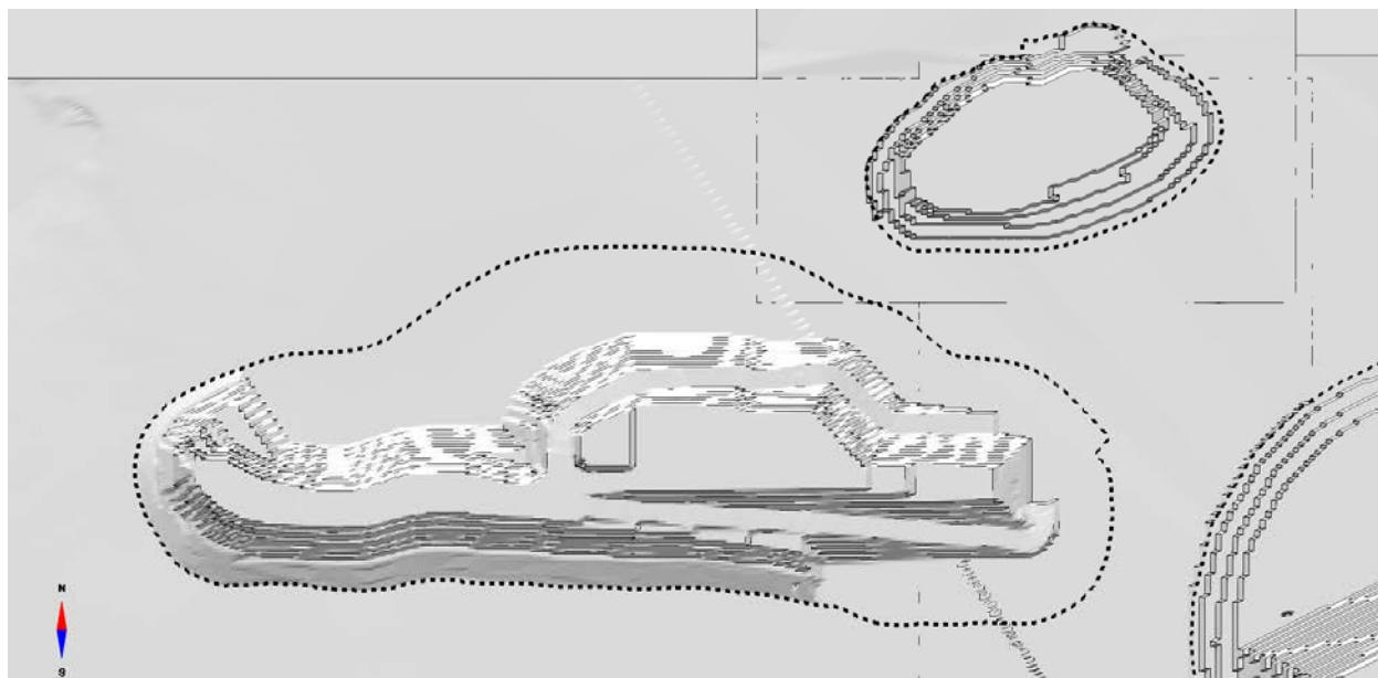
Figure 16-13 West Detour and North Pit End of Period 2028
