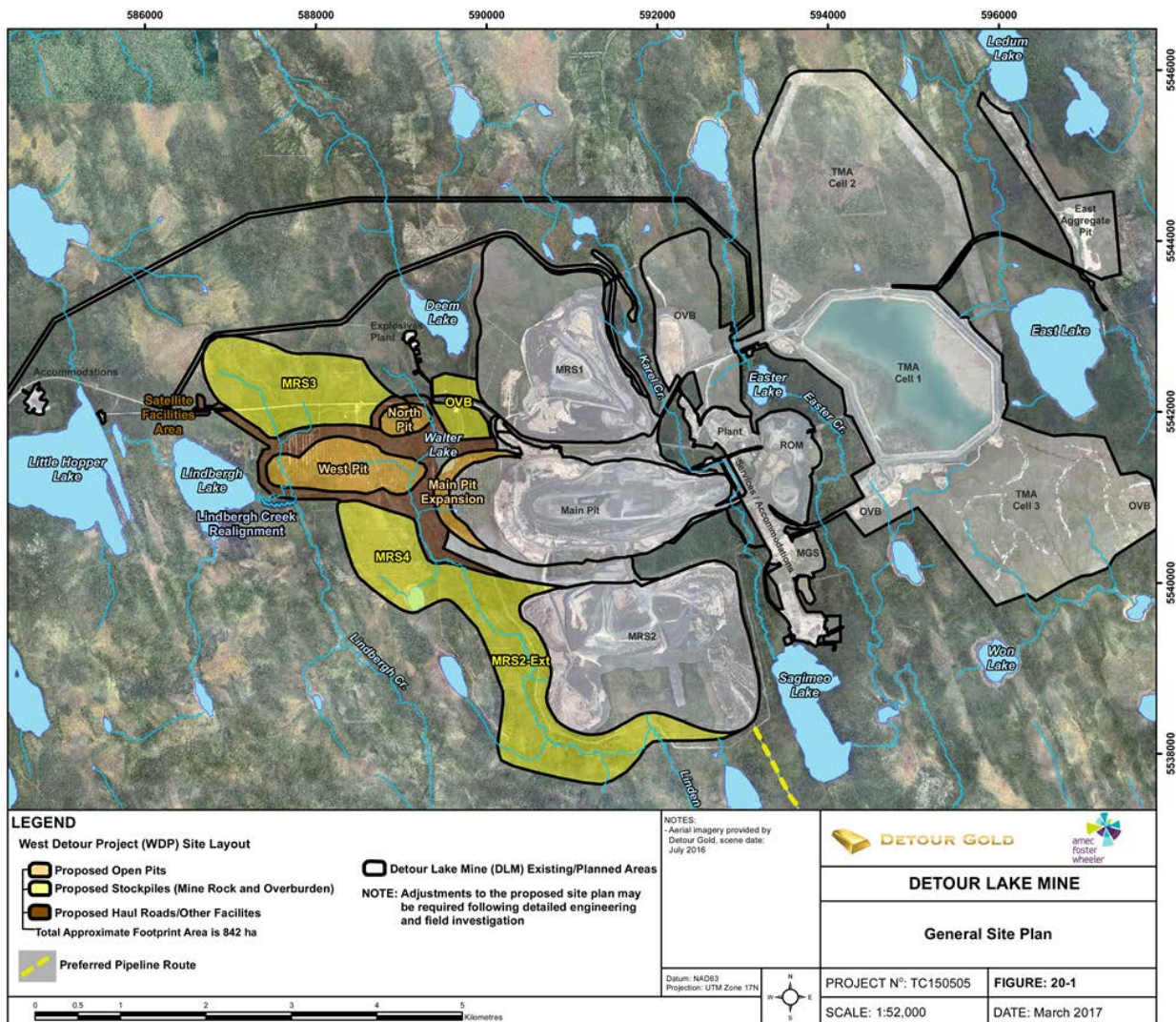
Figure 16-18 Site and Waste Rock Stockpile Layout
