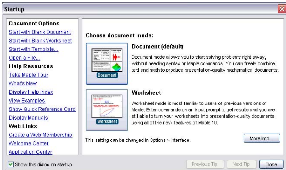
Figure 2.1: Startup Dialog
