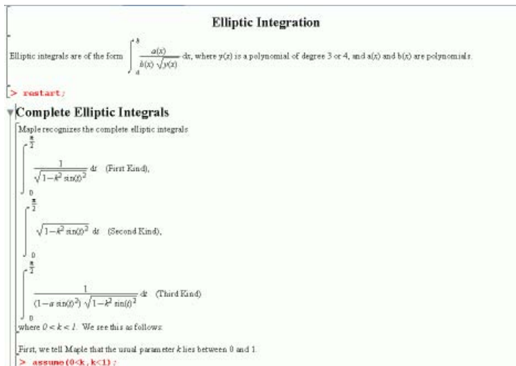
Figure 2.20: Example Worksheet
