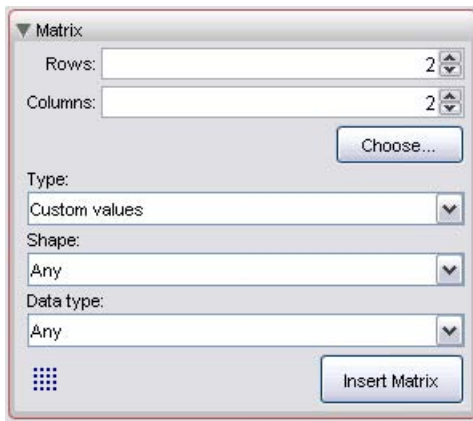
Figure 2.14: Matrix Palette
