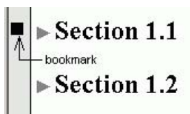
Figure 2.24: Bookmarks
