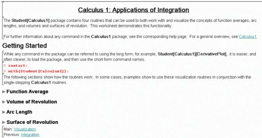
Figure 3.4: Example Worksheet
