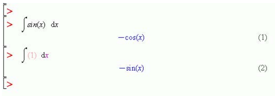
Figure 2.22: Equation Label
