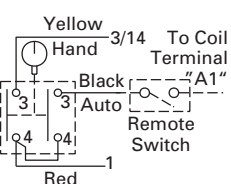
Figure C 3-Position Selector Switch Figure F START/STOP with Pilot Light
