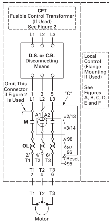
Figure 1 Front View Diagram
