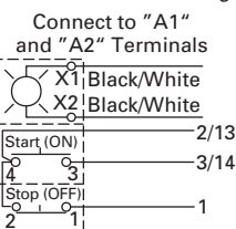
Figure C 3-Position Selector Switch Figure F START/STOP with Pilot Light
