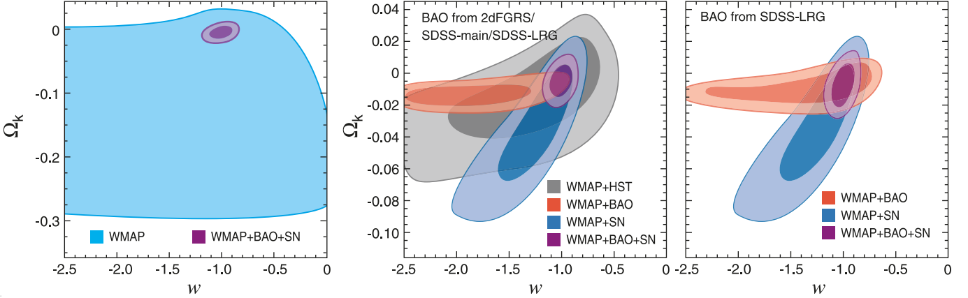
FIG. 12.— Joint two-dimensional marginalized constraint on the time-independent (constant) dark energy equation of state, w , and the curvature parameter, \Omega_k (§ 5.3). Note that we have imposed a prior on w , w > -2.5 . The contours show the 68% and 95% CL. (Left) The WMAP-only constraint (light blue; 95% CL) compared with WMAP+BAO+SN (purple; 68% and 95% CL). This figure shows how powerful the extra distance information from BAO and SN is for constraining \Omega_k and w simultaneously. (Middle) A blow-up of the left panel, showing WMAP+HST (gray), WMAP+BAO (red), WMAP+SN (dark blue), and WMAP+BAO+SN (purple). This figure shows that we need both BAO and SN to constrain \Omega_k and w simultaneously: WMAP+BAO fixes \Omega_k , and WMAP+SN fixes w . (Right) The same as the middle panel, but with the BAO prior re-weighted by a weaker BAO prior from the SDSS LRG sample (Eisenstein et al. 2005). The BAO data used in the other panels combine the SDSS main and LRG, as well as the 2dFGRS data (Percival et al. 2007). The constraints from these are similar, and thus our results are not sensitive to the exact form of the BAO data sets. Note that neither BAO nor SN alone is able to constrain w or \Omega_k : they need the WMAP data for lifting the degeneracy. Note also that BAO+SN is unable to lift the degeneracy either, as BAO needs the sound horizon size measured by the WMAP data.
