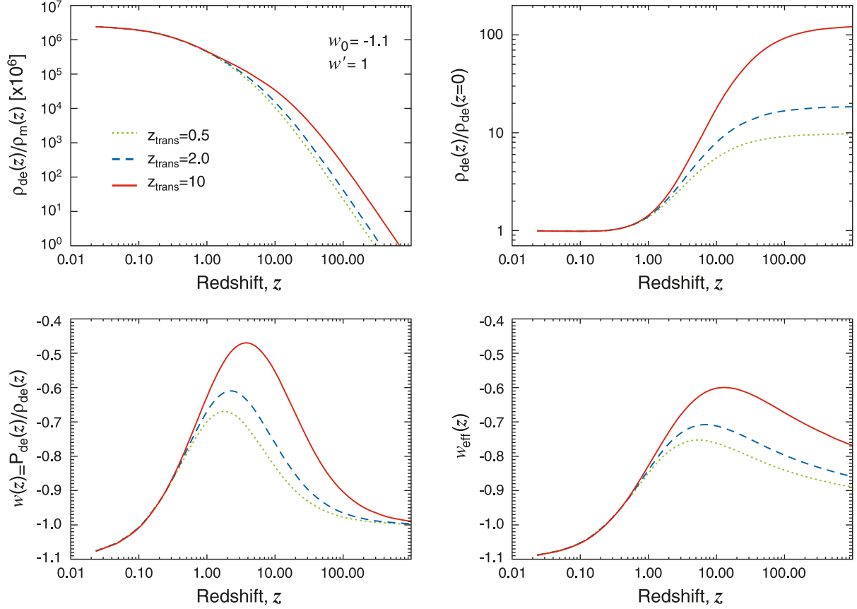
FIG. C1.— Evolution of dark energy for w_0 = -1.1 and w' = 1 , and various transition redshifts, z_{\text{trans}} = 0.5, 2 , and 10 , above which w(z) approaches to -1 . (Top Left) Evolution of the dark energy to matter density ratio as a function of z . Note that the vertical axis has been multiplied by 10^6 . (Top Right) Evolution of the dark energy density relative to the dark energy density at present. The dark energy density was nearly constant at high redshifts above z_{\text{trans}} ; thus, these models can describe the “thawing models,” (Caldwell & Linder 2005) in which dark energy was nearly constant at early times, and had become dynamical at lower redshifts. (Bottom Left) Evolution of the equation of state, w(z) = P_{\text{de}}(z)/\rho_{\text{de}}(z) . By construction of the model, w(z) approaches to -1 beyond z_{\text{trans}} . (Bottom Right) Evolution of the effective equation of state, w_{\text{eff}}(z) , which determines the evolution of dark energy density as \rho_{\text{de}}(z) = \rho_{\text{de}}(0)(1+z)^{3[1+w_{\text{eff}}(z)]} , where
