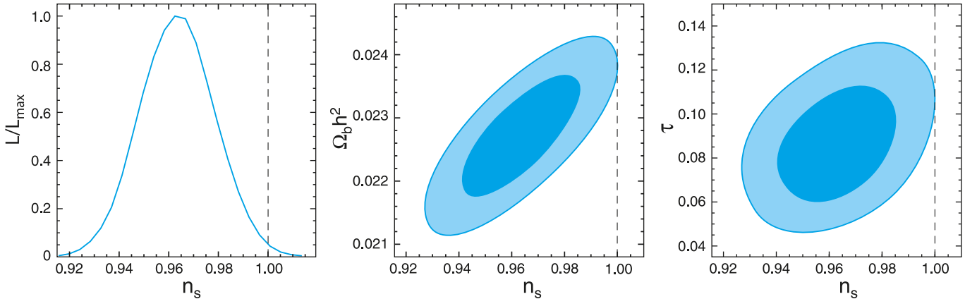
FIG. 1.— Constraint on the primordial tilt, n_s (§ 3.1.2). No running index or gravitational waves are included in the analysis. (Left) One-dimensional marginalized constraint on n_s from the WMAP-only analysis. (Middle) Two-dimensional joint marginalized constraint (68% and 95% CL), showing a strong correlation between n_s and \Omega_b h^2 . (Right) A mild correlation with \tau . None of these correlations are reduced significantly by including BAO or SN data, as these data sets are not sensitive to \Omega_b h^2 or \tau ; however, the situation changes when the gravitational wave contribution is included (see Fig. 3).
