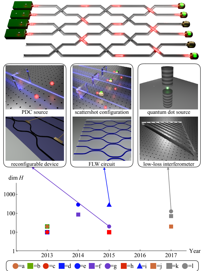
Figure 6. Increase of the Hilbert-space dimensionality \dim H in BOSONSAMPLING experimental implementations with single photons. Top inset: scheme of an integrated photonic device for BOSONSAMPLING, where a no-collision state is injected in the first optical modes and measured at the output after a Haar-random unitary evolution. Legend - PDC: parametric down-conversion, FLW: femtosecond laser writing. Recently the implementation of a lossy BOSONSAMPLING experiment has been reported [595]. Bottom legend: references to the related literature. a: [567]. b: [240]. c: [569]. d: [568]. e: [582]. f: [516]. g: [122]. h: [575]. i: [581]. j: [583]. k: [149]. l: [584]
