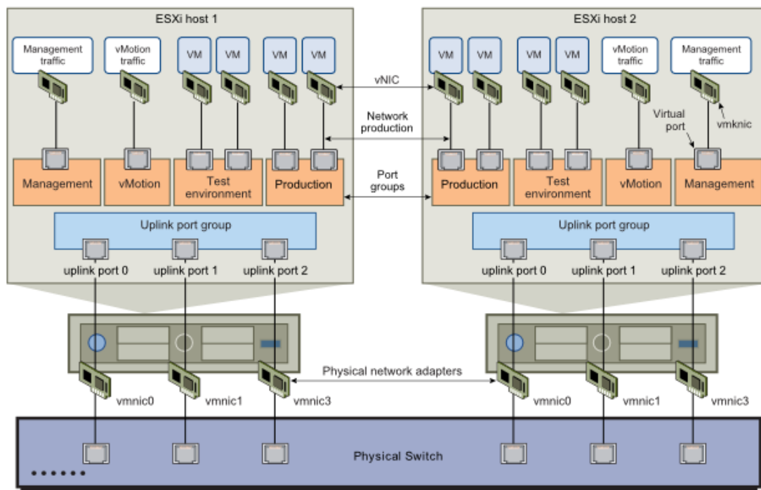
Figure 8. Standard Switch
