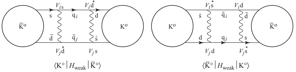
Figure E.1 Quark diagrams illustrating how the weak interaction with W bosons generates mixing. q_i , and q_j are any of the (2/3)e charged quarks u , c or t . The mixing matrix elements are proportional to the products of the four KM factors in the diagrams.
