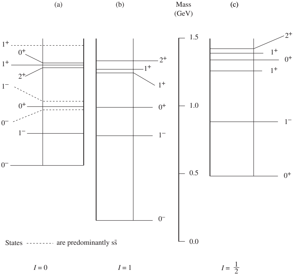
Figure 1.4 States of the quark–antiquark system u\bar{u} , u\bar{d} , d\bar{u} , d\bar{d} form isotopic triplets ( I = 1 ) : u\bar{d} , (u\bar{u} - d\bar{d})/\sqrt{2} , d\bar{u} ; and also isotopic singlets ( I = 0 ) : (u\bar{u} + d\bar{d})/\sqrt{2} . Figure 1.4(a) is an energy-level diagram of the lowest energy isosinglets, including states --- which are interpreted as s\bar{s} states. Figure 1.4(b) is an energy-level diagram of the lowest energy isotriplets. Figure 1.4(c) is an energy-level diagram of the lowest energy K mesons. The K mesons are quark–antiquark systems u\bar{s} and d\bar{s} ; they are isotopic doublets, as are their antiparticle states s\bar{u} and s\bar{d} . Their higher energies relative to the states in Fig. 1.4(b) are largely due to the higher mass of the s over the u and d quarks. The large relative displacement of the 0^+ state is a feature with, as yet, no clear interpretation.
