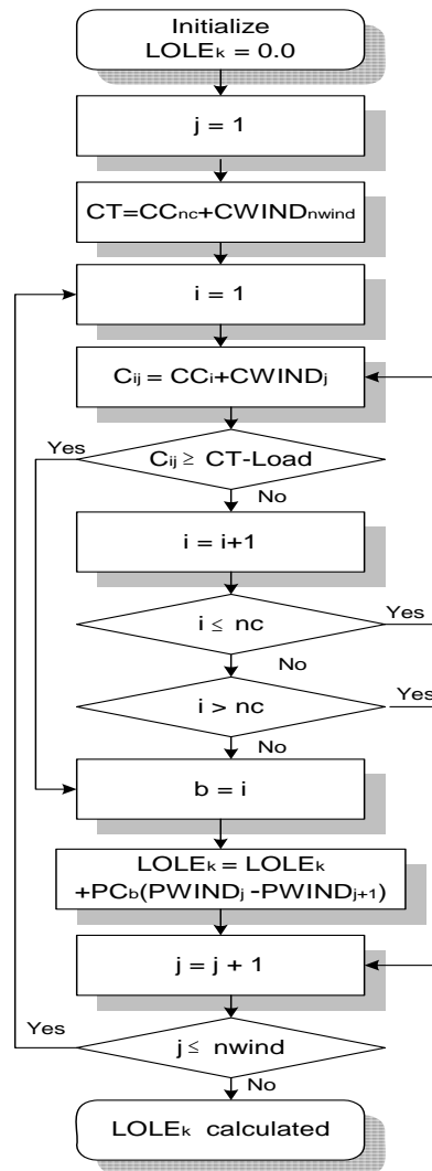
Figure 3. Flow chart for evaluating the LOLE of the system for the k^{\text{th}} hour
