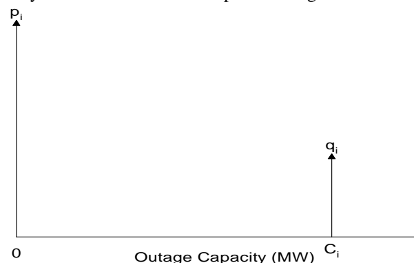
Figure 2. Forced outage capacity probability density function
