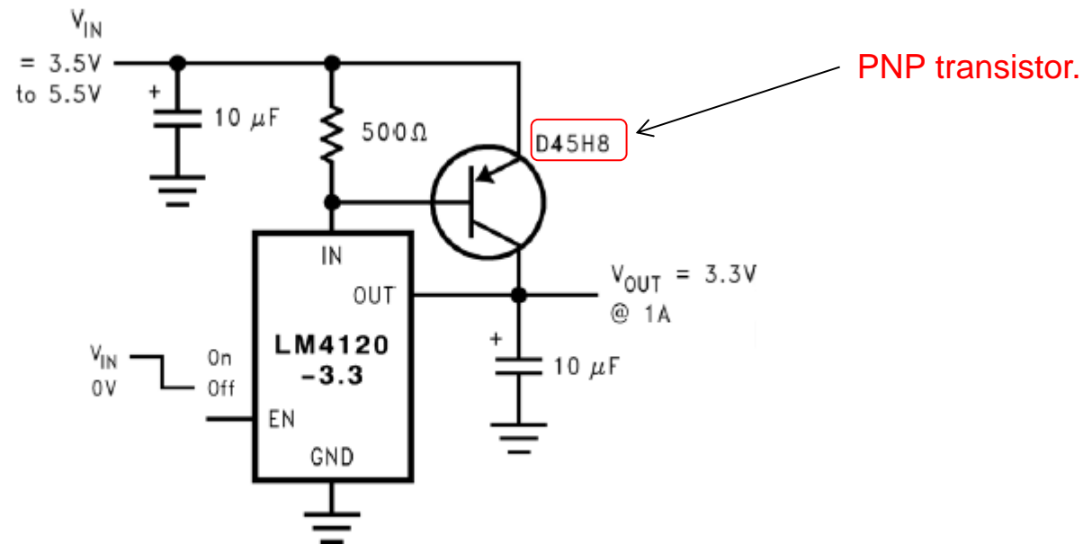
Figure 20. Precision High-Current Low-Dropout Regulator Circuit
