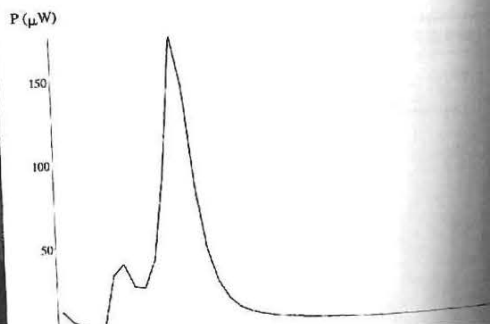
Figure 6.3 Internal hygrostat and heat output due to crystallization of an amorphous phase measured by isothermal microcalorimetry.
