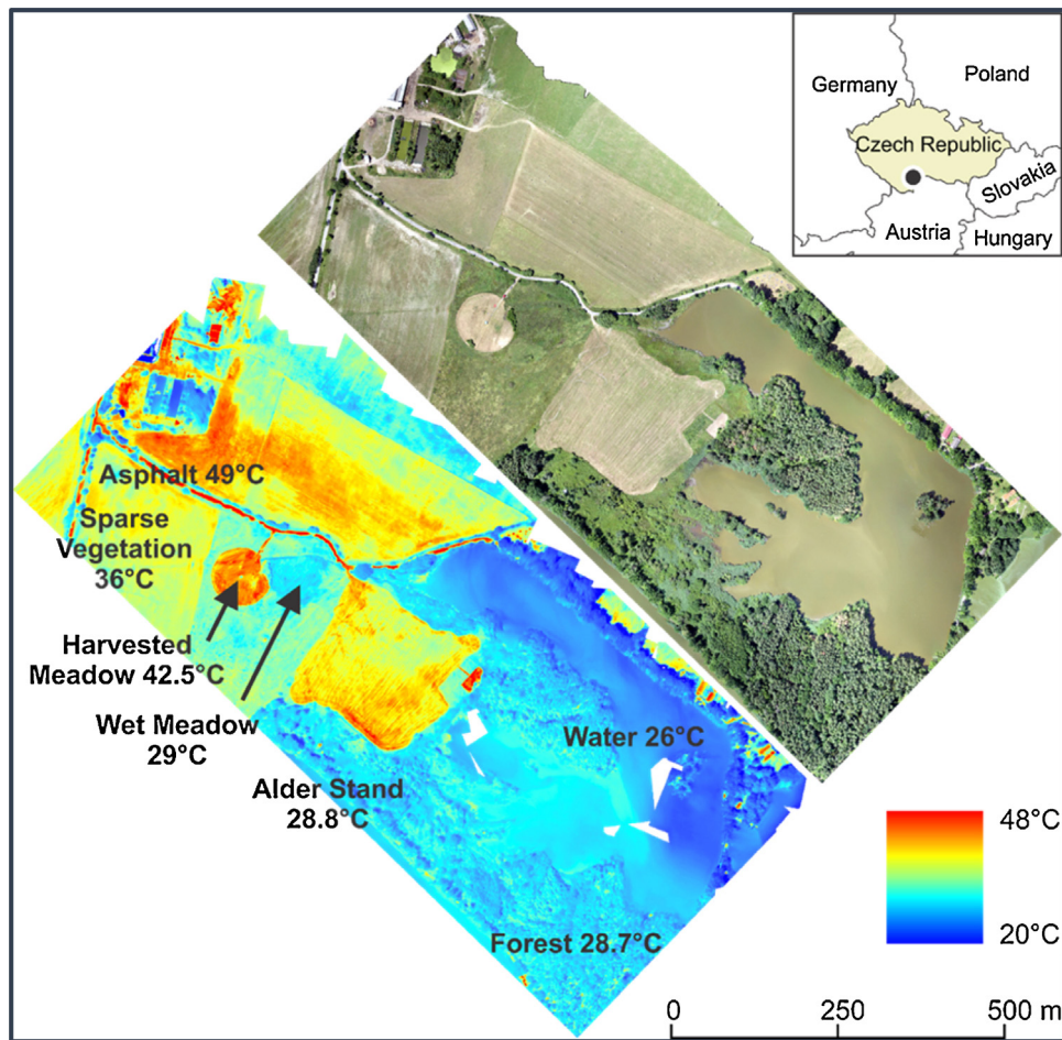
Fig. 2. Surface temperature distribution in a mixed landscape with forest. Source: adapted from (Hesslerová et al. 2013).
