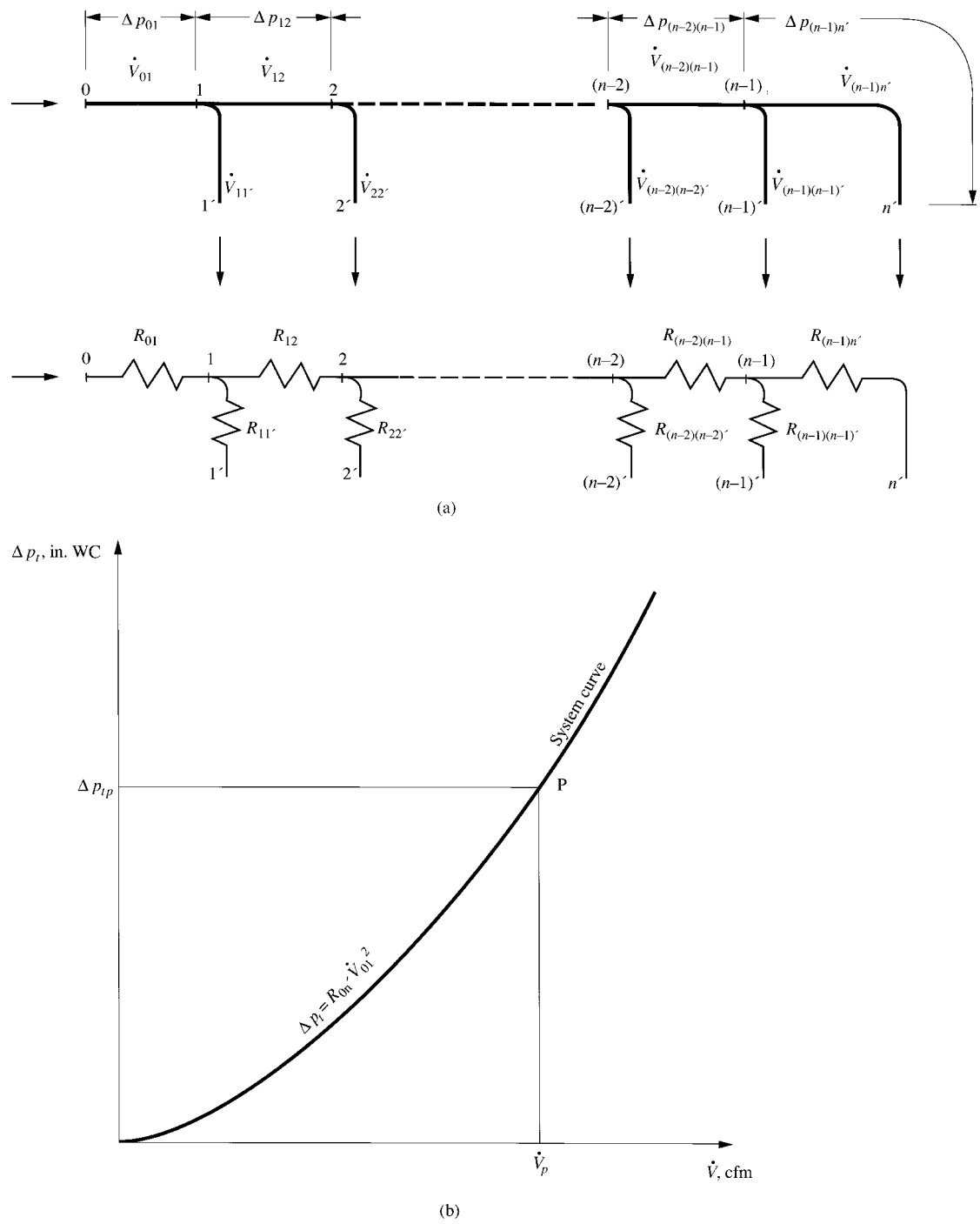
FIGURE 17.19 Flow characteristics of a supply duct system: (a) schematic diagram; (b) system curve.
