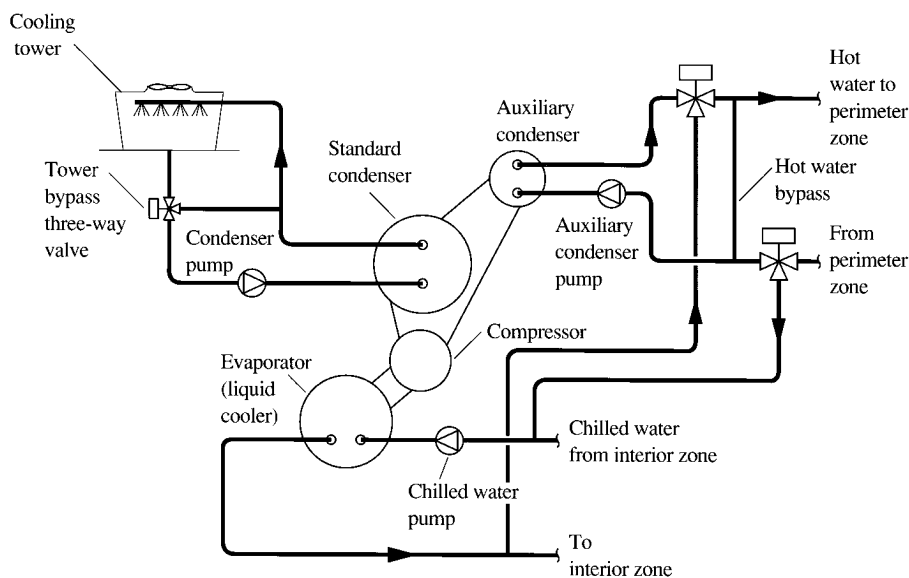
FIGURE 13.6 Heat recovery system using an auxiliary condenser.
