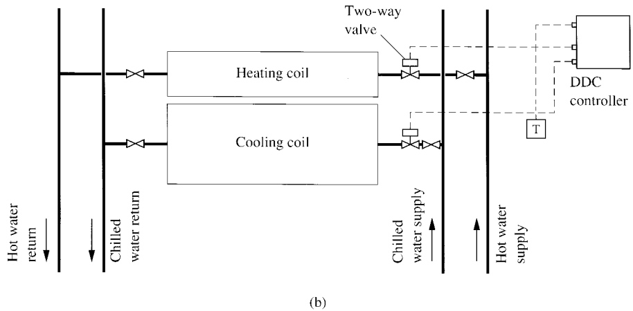
FIGURE 28.3 Four-pipe fan-coil unit system: (a) common coil; (b) separate coil.
