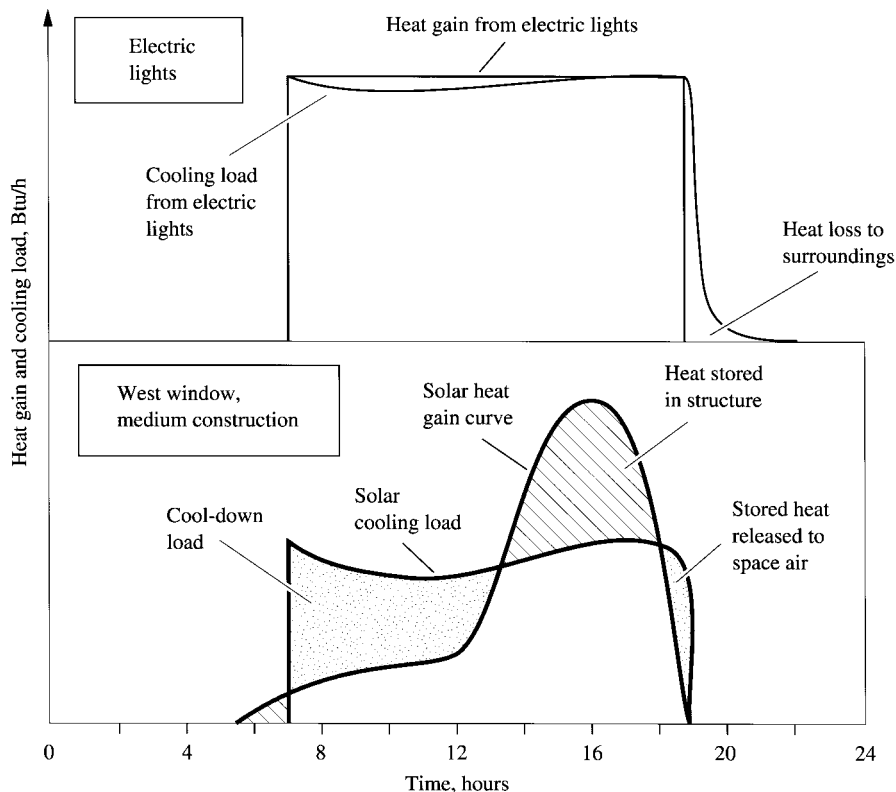
FIGURE 6.2 Solar heat gain and heat gain from electric lights and the corresponding space cooling loads for a night shutdown air system.
