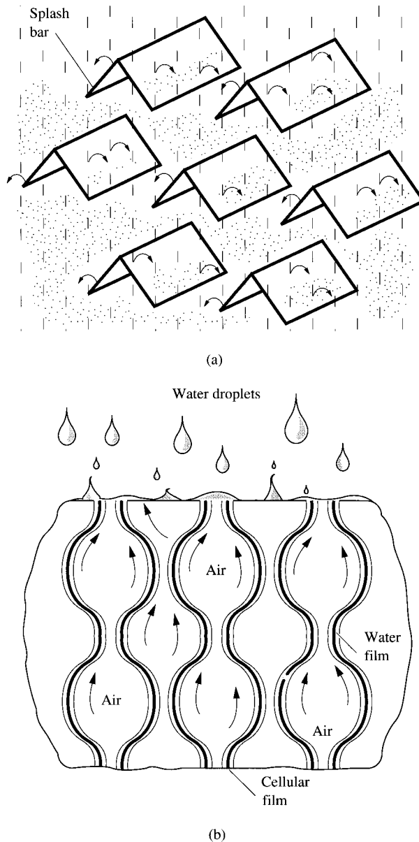
FIGURE 10.15 Two types of fill for cooling towers: (a) splash bars; (b) PVC cellular film.
