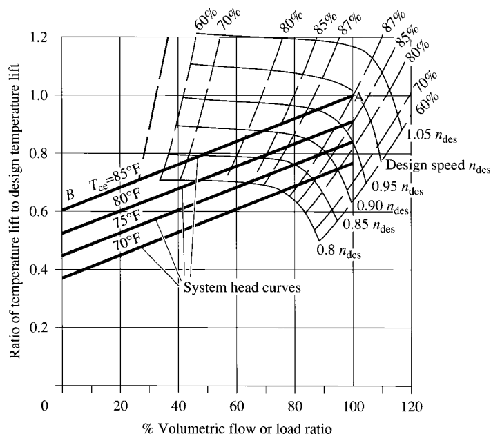
FIGURE 25.2 Compressor map of a centrifugal chiller at various load ratios R_{load} and T_{ce} .
