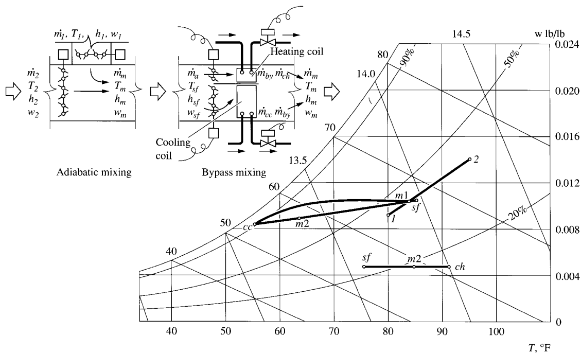
FIGURE 20.21 Adiabatic mixing and bypass mixing processes.
