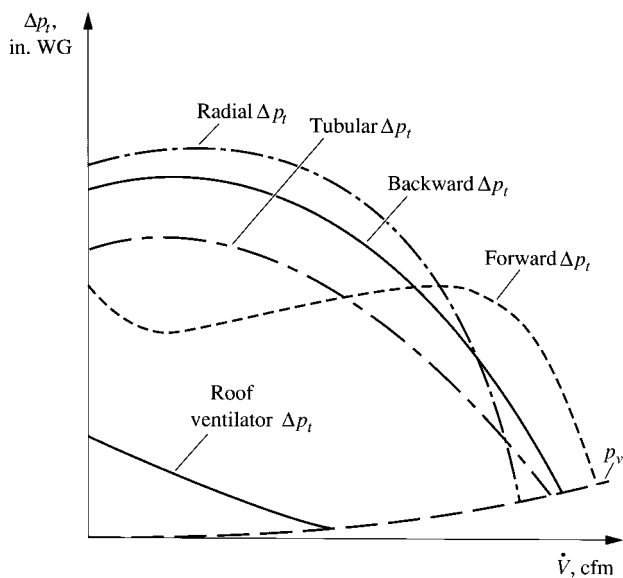
FIGURE 15.8 Pressure-volume \Delta p_t - \dot{V} performance curves for centrifugal fans with same impeller diameter.
