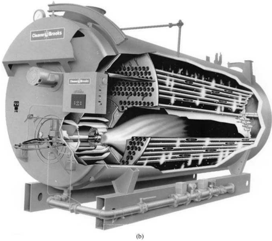
FIGURE 8.3 Scotch marine packaged boiler. (a) Schematic diagram; (b) a cutaway photograph of a typical product. (Source: Cleaver-Brooks. Reprinted with permission.)
