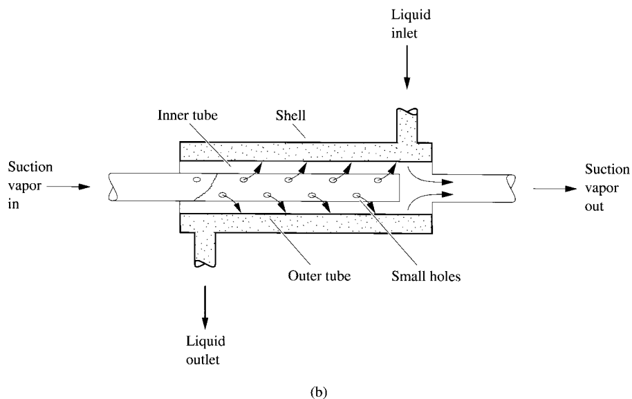
FIGURE 11.6 Liquid suction heat exchanger: (a) schematic diagram; (b) heat exchanger.
