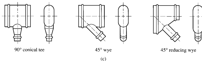
FIGURE 17.12 Round and flat oval tees and wyes: (a) round tees, wyes, and cross; (b) diverging tees and wyes with elbows; (c) flat oval tees and wyes.
