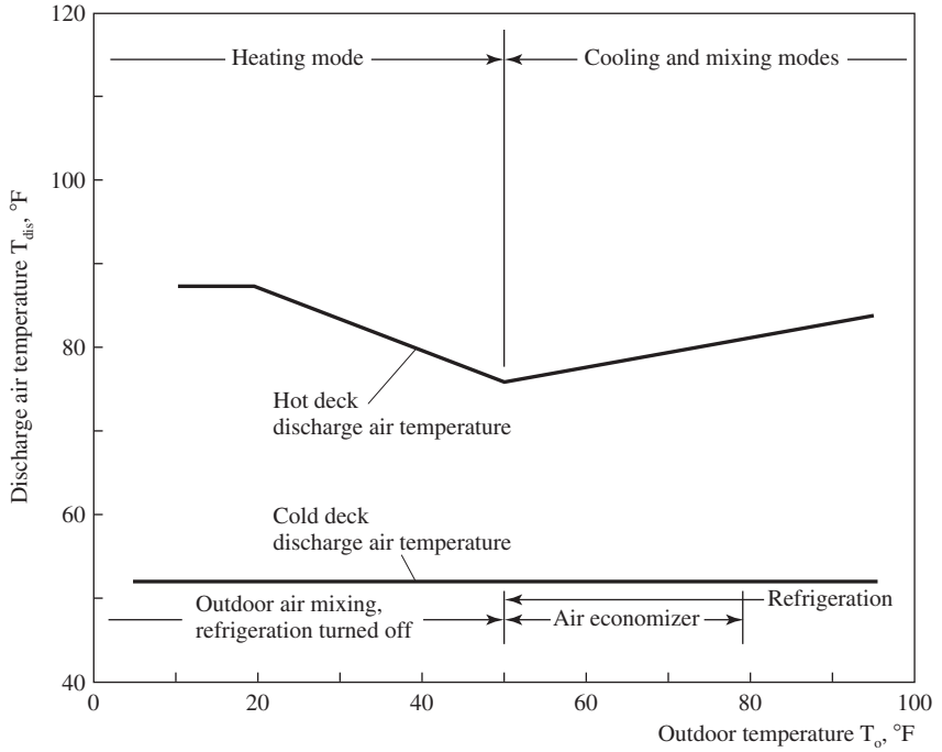
FIGURE 21.11 Warm and cold deck discharge air temperature in a dual-fan dual-duct VAV system.
