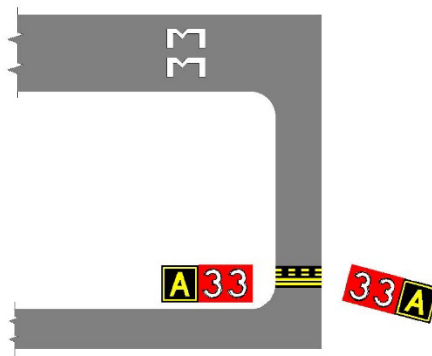
(b) Example of a Holding Position Sign on the Left Side of the Taxiway that Would be Difficult for the Pilot to See Due to Holding Position. Note the Addition of a Canted Sign on the Right Side of Taxiway to Improve Visibility
