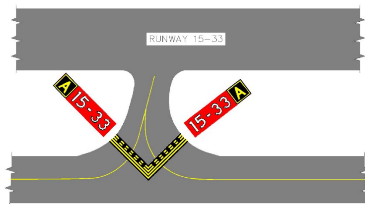
(c) Example Where Painted Holding Position Markings do not Extend Straight Across the Taxiway
