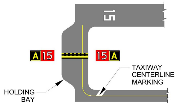
(a) Example of Holding Position Markings Extending Across Holding Bay
