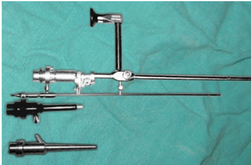
Fig. 8.7: Instrumentation (wave guides, hand piece, coupler) used for laser surgery
