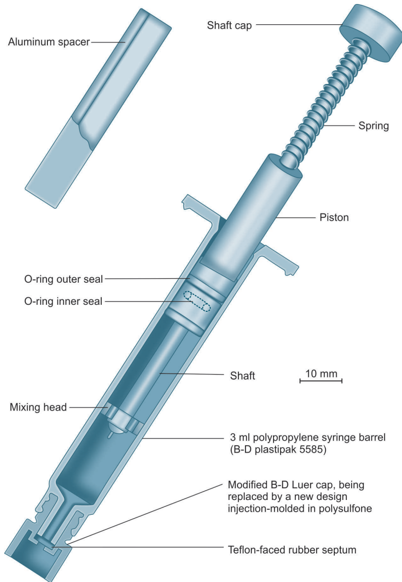
Fig. 17.6: The mixer-dispenser syringe (Advanced Medical Grade Silicones BV, The Netherlands) allows the catalyst to be injected with the silicone and mixed. A spacer converts it into an injection syringe, which is connected to the coaxial catheter and placed in the fluid flow actuator. (Reproduced by permission of Siegler AM, Lindemann HJ (Eds). Hysteroscopy: Principles and Practice . Philadelphia: JB Lippincott, 1984)
