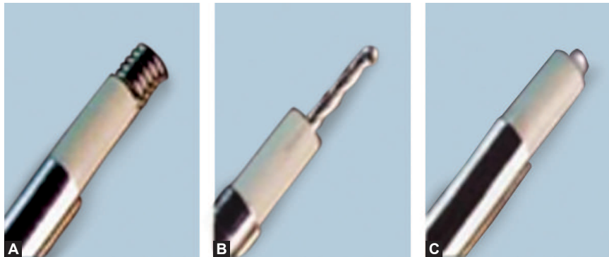
Figs 5.2A to C: Spring, twizzle and ball electrodes from left to right
