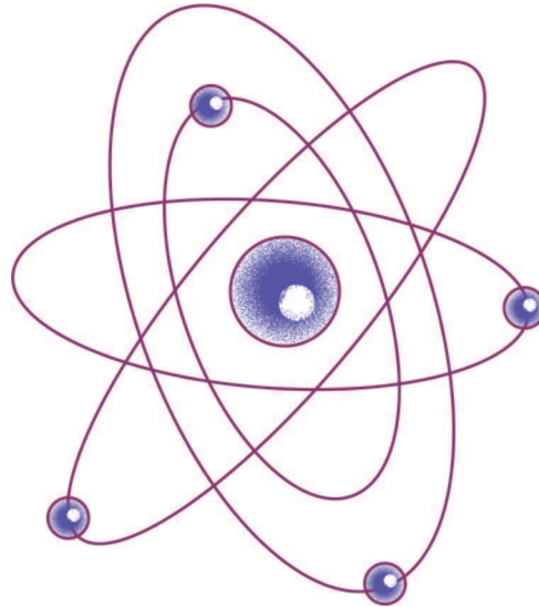
Fig. 8.1: Illustration of an atom with a nucleus and orbiting electrons
