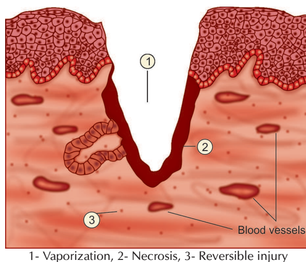
Fig. 8.11: A CO 2 laser beam produces a spot or crater in which three zones of tissue injury may be identified
