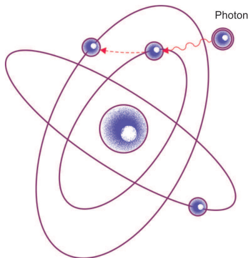
Fig. 8.2: Stimulated absorption occurs as a photon impacts on an electron, driving it into a higher orbit
