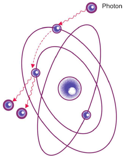
Fig. 8.4: The natural “slow” decay process may be stimulated by collision processes, resulting in many photons travelling at the same frequency as the inducing photons
