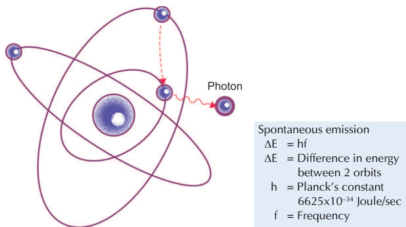
Fig. 8.3: Slow, natural decay causes an electron to drop into a lower orbit, resulting in a photon being emitted at a predicted frequency equal to the difference in energy between the two orbits
