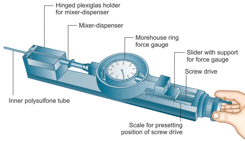
Fig. 17.5: Fluid flow actuator system (Advanced Medical Grade Silicones BV, The Netherlands) used to drive the activated and hardening silicone out of the syringe and down the coaxial catheter and into the fallopian tubes. (Reproduced by permission of Siegler AM, Lindemann JH (Eds). Hysteroscopy: Principles and Practice . Philadelphia: JB Lippincott, 1984)
