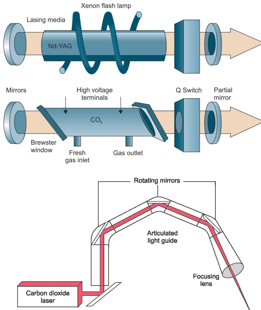
Fig. 8.9: Laser system components
