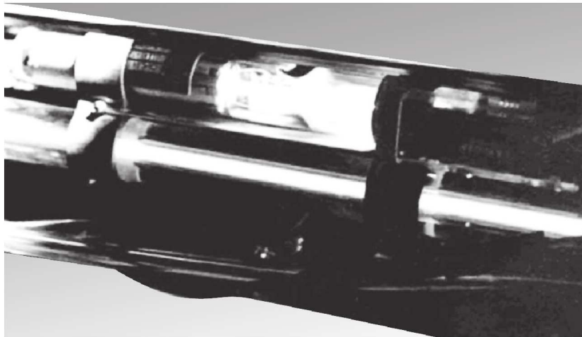
Fig. 8.6: Actual view of a CO 2 laser tube (below) and coincident helium-neon laser (above), which provides visible aiming target
