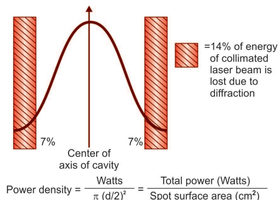
Fig. 8.10: An example of the distribution of a laser beam, whose intensity is greatest in the center of the axis. On either end of the bell-shaped curve, 7 percent of the energy is lost because of diffraction. The power density (intensity) is equivalent to laser power packed into a given spot. The smaller the spot, the greater the power density
