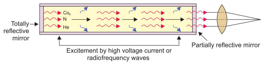
Fig. 8.5: Schematic diagram of a CO 2 laser tube. Photons reflect between the two mirrors (in phase) and eventually exit as the laser beam by way of the partially reflective mirror
