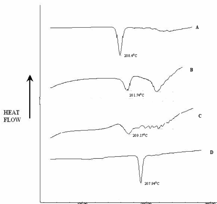
Figure 2: D.T.A of amlodipine besylate and with excipients A) Pure drug, B) Drug with SSG, C) Drug with MCC and D) Drug with camphor
