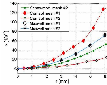
Fig. 10. Angular acceleration \alpha of the point and screw model depending on the wires radial position at cylinder bottom (voltage source: U_0 = 1.5 V).
