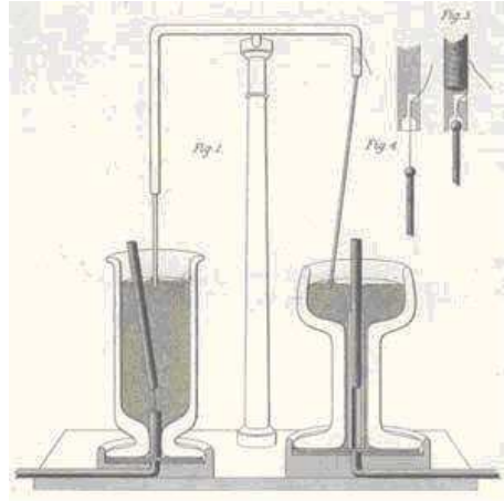
Fig. 1. The first electric motor - Michael Faraday, 1821 (from [1]).
