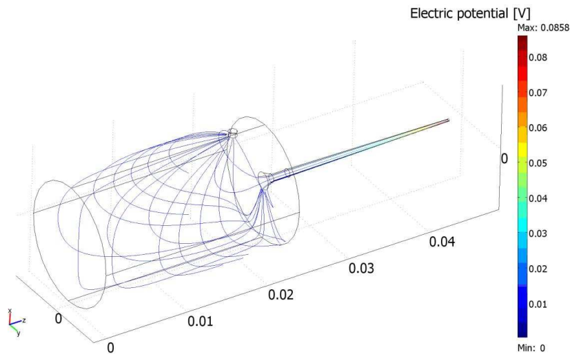
Fig. 21. FEM solution of the SPICE model for the total current density (streamlines), and the distribution of electric potential on the screw (colored scaling).
