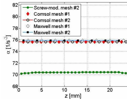
Fig. 13. Angular acceleration \alpha of the point and screw model depending on the wires axial position along the z -axis at the cylinder surface ( z = 0 mm corresponds to the bottom, z = 24 mm to the top of the cylinder; current source: I_0 = 10 A).
