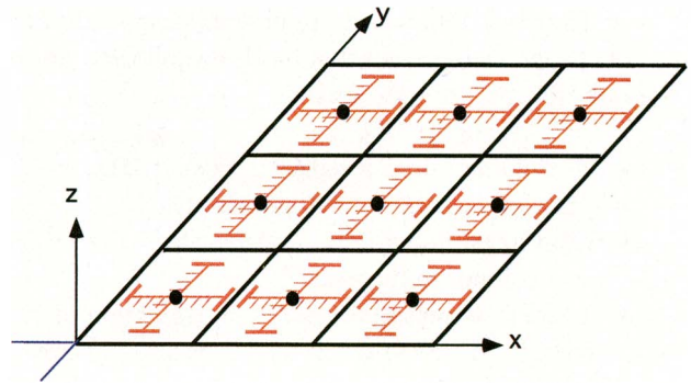
FIG. 17. An evolved version of the original superparameterization concept depicted in Fig. 16. Two CSRs are embedded in each GCM grid box. They are oriented at right angles to each other. They have periodic boundary conditions, as before. At the point where the two high-resolution grids overlap, the CSR is three-dimensional. Elsewhere, it is two-dimensional.
