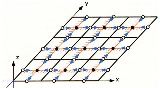
FIG. 18. Here the two orthogonal high-resolution grids are extended to the walls of the GCM grid cells. The periodic boundary conditions are replaced by a direct coupling of the CSRs in neighboring GCM cells, as depicted by the blue arrows. The open circles represent points at which the large-scale winds are predicted. At a CSR grid point that is not at the intersection of the two high-resolution grids, we can do a quasi-three-dimensional calculation by interpolation between the neighboring orthogonal high-resolution grids.
