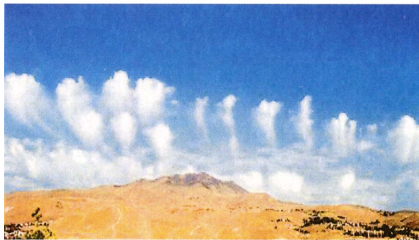
FIG. 7. Precipitation falling from elevated cumuli. When there are multiple cloud layers, such precipitation can fall through either clear or cloudy air. Such microphysical overlap influences the precipitation rate and other processes.
