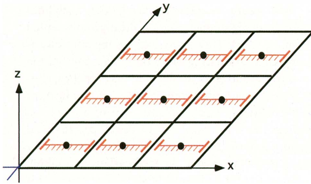
FIG. 16. The black squares represent an array of GCM grid boxes, and the red lines represent embedded two-dimensional CSRs. The CSR domains do not extend to the edges of the GCM grid boxes. The lateral boundary conditions on the CSRs are periodic. At the black dots, the GCM and the domain average of the CSR interact.
