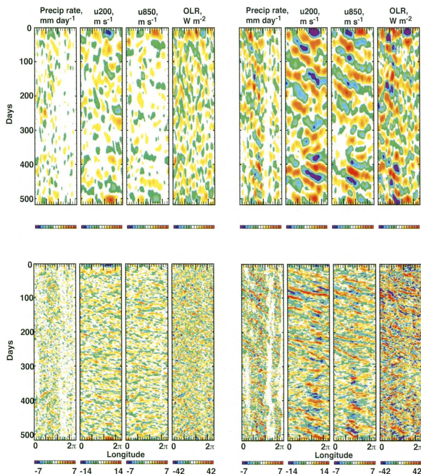
FIG. 12. Hövmöller diagrams for the precipitation rate, 200-mb zonal wind, 850-mb zonal wind, and OLR in a control run with the T21 CAM, and in an experiment with the same model modified to use the superparameterization. In the top two panels, the results are filtered to show variability with periods in the range 20–100 days. The bottom two panels show variability in the 2–20-days range.
