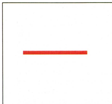
FIG. 11. Grabowski embedded a 2D CSRМ inside each grid cell of a global model. Here the black box represents a GCM grid cell. The red bar represents the 2D CSRМ. In this example, the CSRМ is oriented east–west (i.e., left–right in the sketch). Grabowski and Smolarkiewicz (1999) and Grabowski (2001) experimented with a north–south orientation as well. As would be expected, the results obtained depend to some extent on the orientation chosen. See Grabowski’s papers for further discussion.
