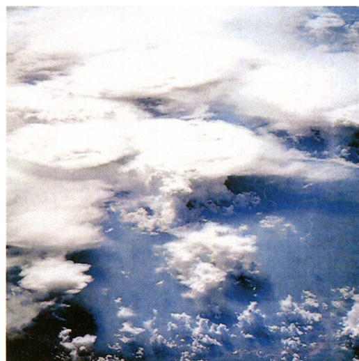
FIG. 4. Cumulus convection generates stratiform cloudiness through detraining of ice and liquid. A major portion of all stratiform cloudiness is produced through such detraining.
