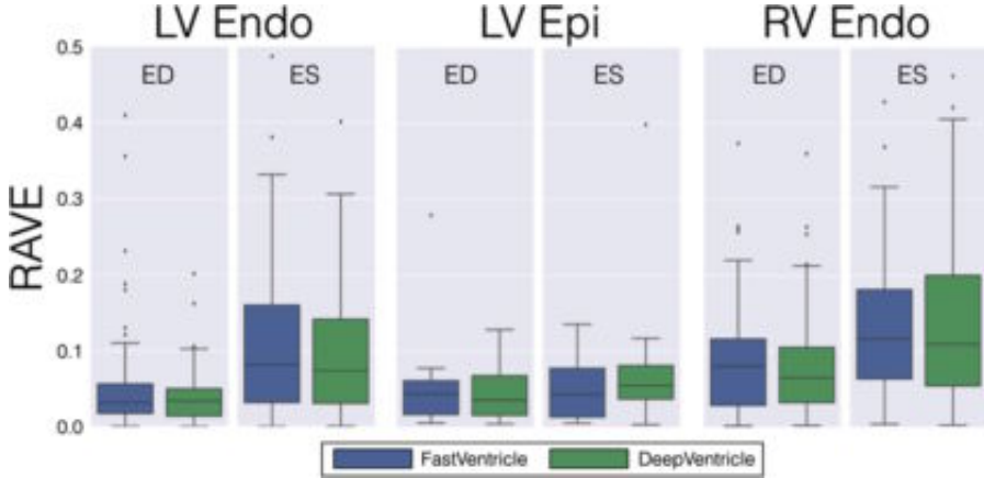
Fig. 2. Boxplots comparing the relative absolute volume error (RAVE) between FastVentricle and DeepVentricle for each of LV endo, LV epi, and RV endo at ED (left panels) and ES (right panels). The line at the center of each box denotes the median RAVE, the ends of the box show 25% (Q1) and 75% (Q3) of the distribution. Whiskers are placed at the first value within 1.5 interquartile ranges past the first and third quartiles.
