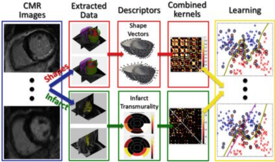
Fig. 1. The proposed pipeline to go from CMR images to classification models. CMR images are semi-automatically segmented to extract the infarct and shape information. From the created models, the relevant data is obtained: shape descriptors and infarct location and volume. Finally, different combinations of kernels are constructed and the best combination is used in the MKL algorithm to perform classification.
