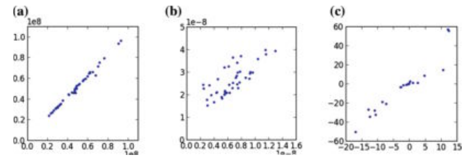
Fig. 2. (a): (MP - P_{ve})/CO as a function of R , (b): SV/(MP - DP) as a function of C , (c): \Delta\sigma (%) as a function of \Delta SV (%)
