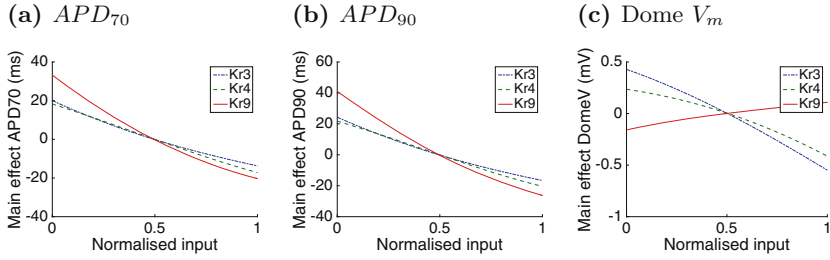
Fig. 4. Main effects of inputs Kr3 , Kr4 , and Kr9 on (a) APD_{70} , (b) APD_{90} , and (c) dome V_m . Each input is plotted on a normalised scale corresponding to the range in Table 1.
