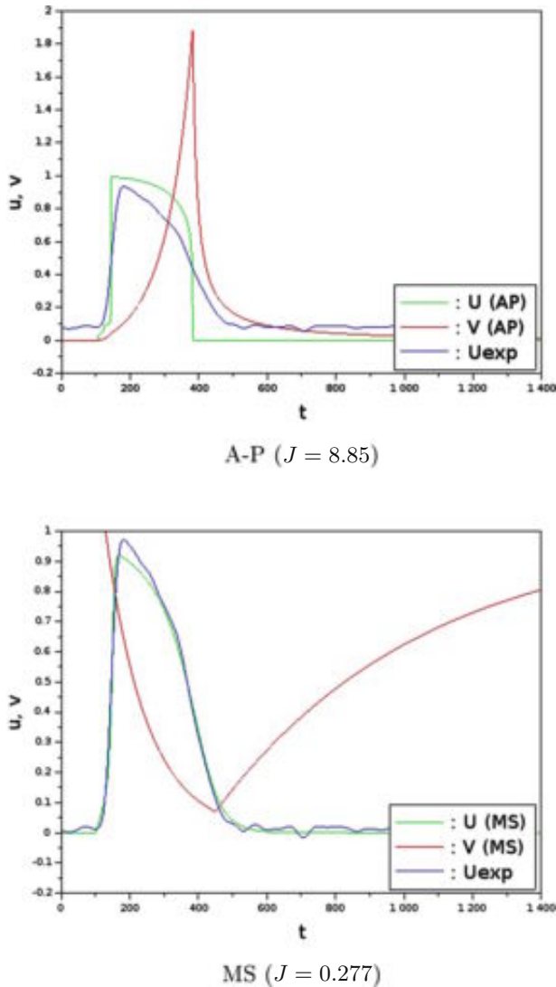
Fig. 1. A-P and MS models fitted to AP recorded by optical fluorescence
