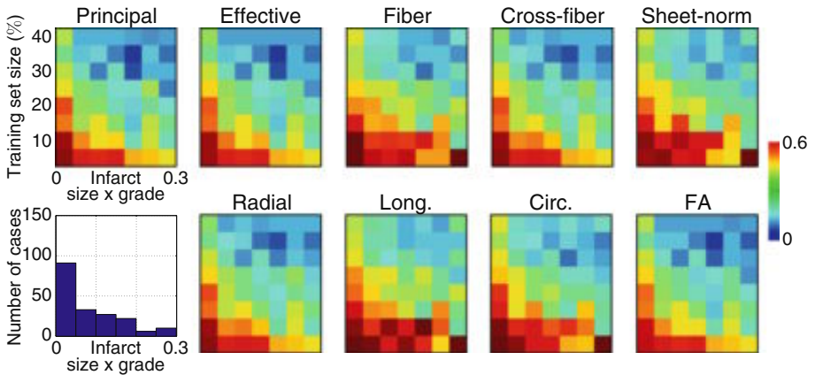
Fig. 3. Performance of the strain-based parameters (median over the tested cases). The color bar depicts the distance to an ideal localization. Horizontal axis: a normalized combination of the degree of severity and the size of the infarct. Vertical axis: the percentage of the population used as the training set. The histogram shows the number of cases that correspond to the infarct size-severity measure on the horizontal axis. (Color figure online)
