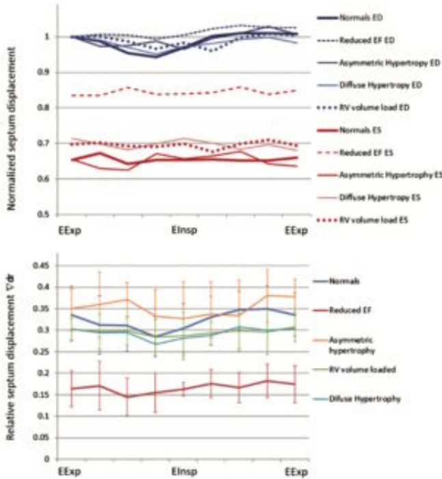
Fig. 6. d_{ES,r} (red) and d_{ED,r} (blue), normalized by d_{ED,r} (Top), and \nabla d_r (Bottom) for the respiratory cycle from end-expiration (EExp) to end-inspiration (EInsp) and back to EExp. For the normal, reduced EF, asymmetric hypertrophy, diffuse hypertrophy, and volume loaded RV subgroups. Note the greater variation in the normal subjects. (Color figure online)
