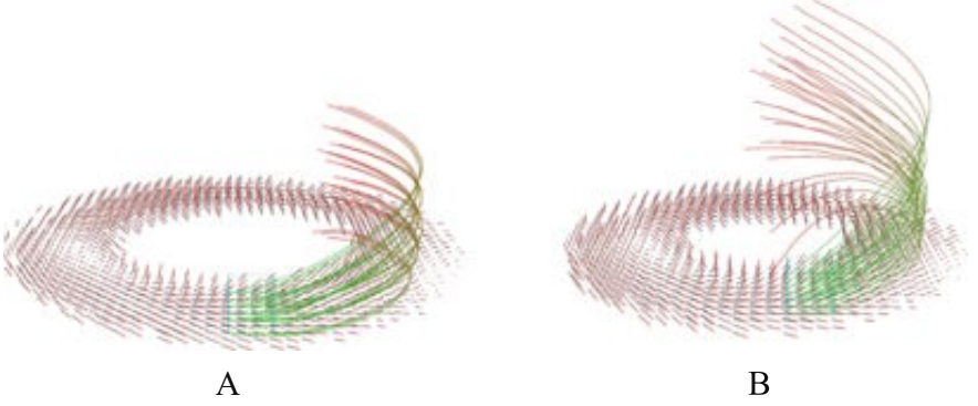
Fig. 2. An illustration of the simulated motion of canine heart wall fibers in the left ventricle at two time points in the systolic phase: 50 ms (A) and 350 ms (B). The fiber orientations are shown in red and partial tractography provides a visualization of fibers in a local neighborhood. In this simulation the total transmural applied rotation ( \theta ) from 0 ms to 400 ms is 20^\circ . (Color figure online)
