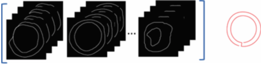
Fig. 2. Left: clusters in the shape pool; right: mean shape.
