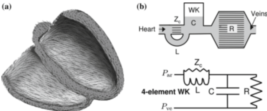
Fig. 1. (a): 3D heart geometry with myocardial fibres directions, (b): Schema and rheological model and of the Windkessel model (figure from [7])
