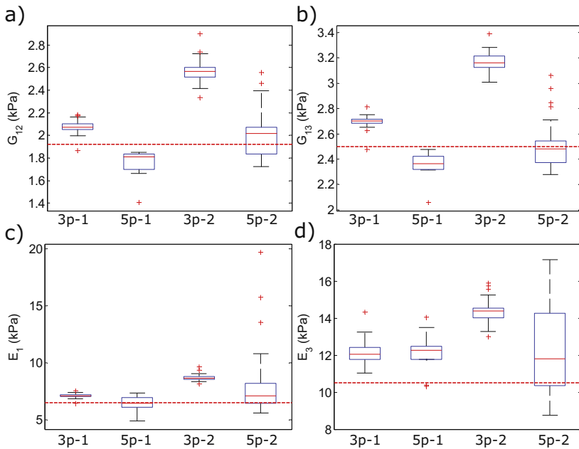
Fig. 2. Resulting estimated (a) transverse shear modulus ( G_{12} ), (b) fibre shear modulus ( G_{13} ), (c) transverse Young's modulus ( E_1 ) and (d) fibre Young's modulus ( E_3 ) for converged Monte-Carlo simulations from the five-parameter (5p) and three-parameter (3p) estimation methods for both loading cases (-1 and -2). Reference parameters are shown by red dotted lines. (Color figure online)
