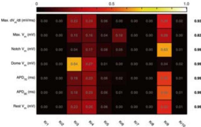
Fig. 3. Sensitivity indices for each combination of input and output. The column to the right is the sum of sensitivity indices for each output. Inputs Kr3 and Kr4 scale the magnitude and voltage dependence of gate activation (Eq. 3), and input Kr9 scales the voltage dependence of steady state activation (Eq. 6).
