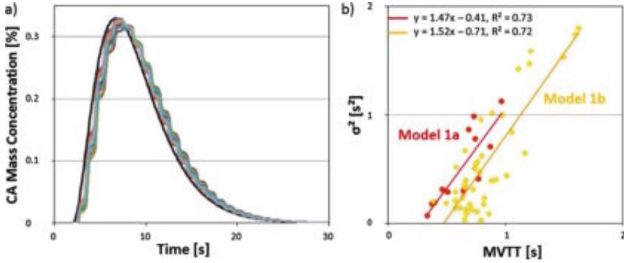
Fig. 3. Results for dispersion, MVTT and \sigma^2 . (a) shows AIF_{disp} at all outlets of model Fig. 1(a), with the applied inlet concentration time curve AIF_{LV} (black). (b) depicts \sigma^2 as a function of MVTT for both models. The results at the outlets of model Fig. 1(a) are shown in red, with a linear fit (red line, standard errors for slope and intercept: \pm 0.28 , \pm 0.19 , resp.). Analogously the results for model Fig. 1(b) are depicted in yellow (standard errors \pm 0.15 , \pm 0.13 ). Error margins of the graphs overlap, however, they do not yield information on vessel generation dependence of dispersion. (Color figure online)
