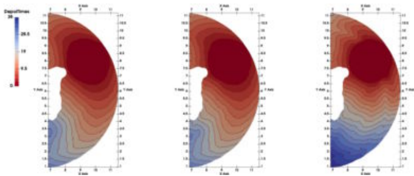
Fig. 6. Depolarization isochrones. From left to right: reference case, parallel plates and perpendicular plates, \sigma_d = 0.02 \text{ Sm}^{-1} . Time between consecutive isochrones is 2 ms.
