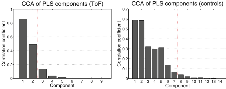
Fig. 2. Canonical correlations for PLS for the Tetralogy of Fallot group (left) and the control group (right). The red line indicates the minimum number of components needed for each group to obtain statistically significant combinations of the modes. Fewer components were required in the more heterogeneous pathological group (i.e. the ToF group) than relatively homogeneous control group. (Color figure online)
