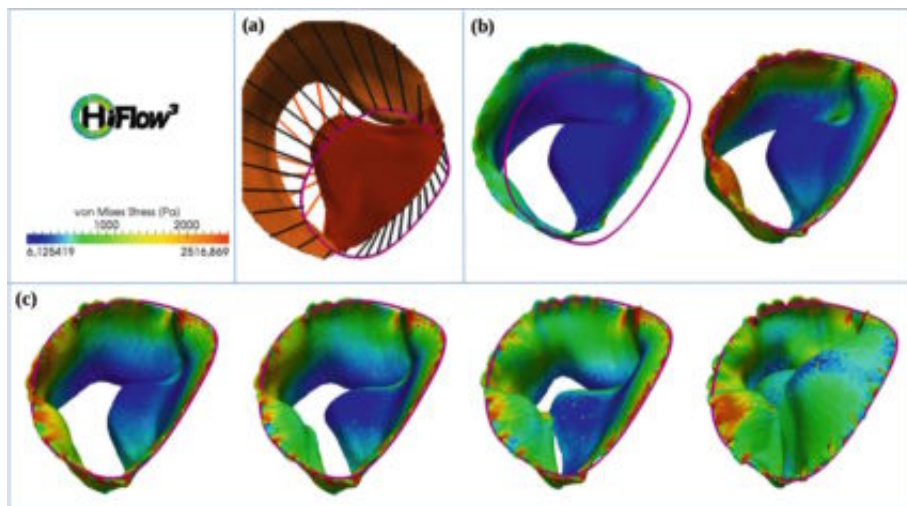
Fig. 3. Visualization of MVR surgery simulation results that were obtained from the cognition-guided, patient-specific MVR surgery assistance system prototype, showing by the example of one test patient (a) the patient- and ring-specific biomechanical model of the MVR ring implantation process, that constitutes the basis for the subsequent simulation, (b) the virtual annuloplasty ring implantation process itself, and (c) the MV closing behavior during a post-surgical cardiac cycle. In addition to the actual deformation behavior, the colors encode the arising von Mises stress distribution. (Color figure online)
