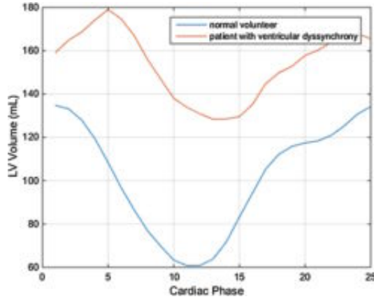
Fig. 9. LV volume change along time within a full cardiac cycle for a normal volunteer and a patient with heart dyssynchrony.
