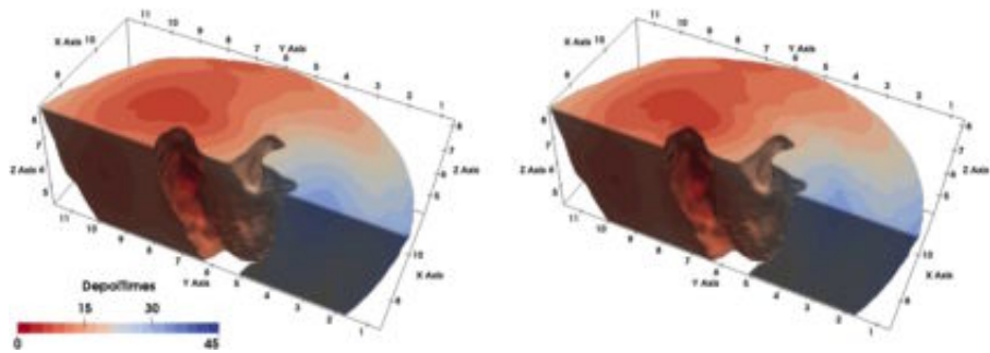
Fig. 5. Depolarization isochrones. From left to right, reference case and parallel plates, \sigma_d = 0.02 \text{ Sm}^{-1} . Time between consecutive isochrones is 2.5 ms.
