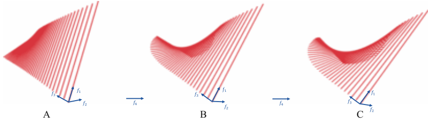
Fig. 1. The application of a specific set of 4D connection parameters c_{ijk} to a frame field attached to a fiber direction. See text for a discussion.
