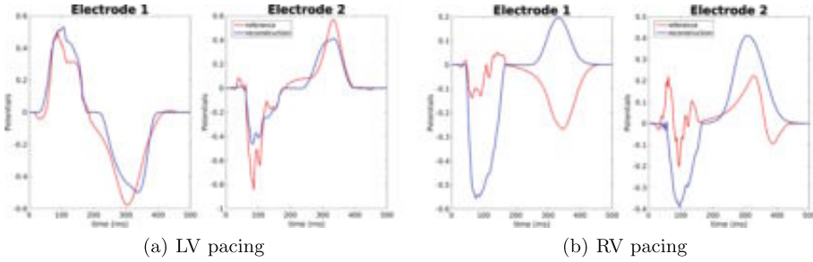
Fig. 8. Reconstructed potentials for in silico data. Electrode 1: close to the heart, Electrode 2: right hip. Red line: reference BSPM; blue line: reconstructed BSPM. (Color figure online)
