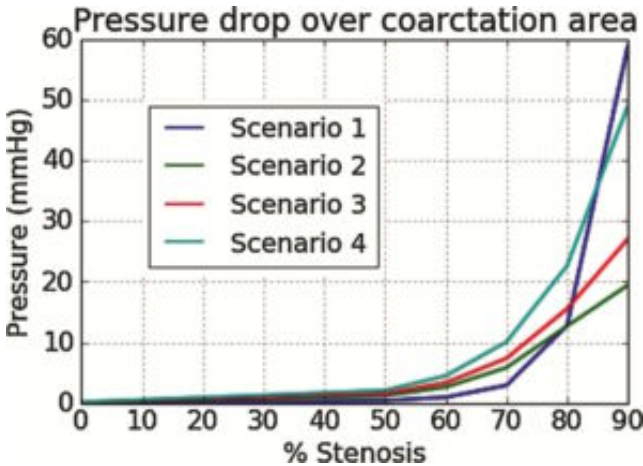
Fig. 5. Maximum pressure drop over area of coarctation, against percentage of stenosis. Dark blue: coarctation of distal aortic isthmus; Green: hypoplasia of aortic isthmus, Red: hypoplasia of aortic isthmus and descending arch; Light blue: hypoplasia of aortic isthmus, descending arch and ascending arch. (Color figure online)
