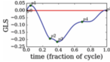
Fig. 1. Synthetic GLS curve model.
