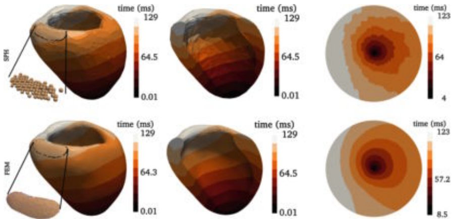
Fig. 3. Left: Contour color map of depolarization times for the left ventricle model. Middle: a longitudinal cross section of the ventricle. Right: projected endocardium onto a disk for both SPH and FEM simulations.
