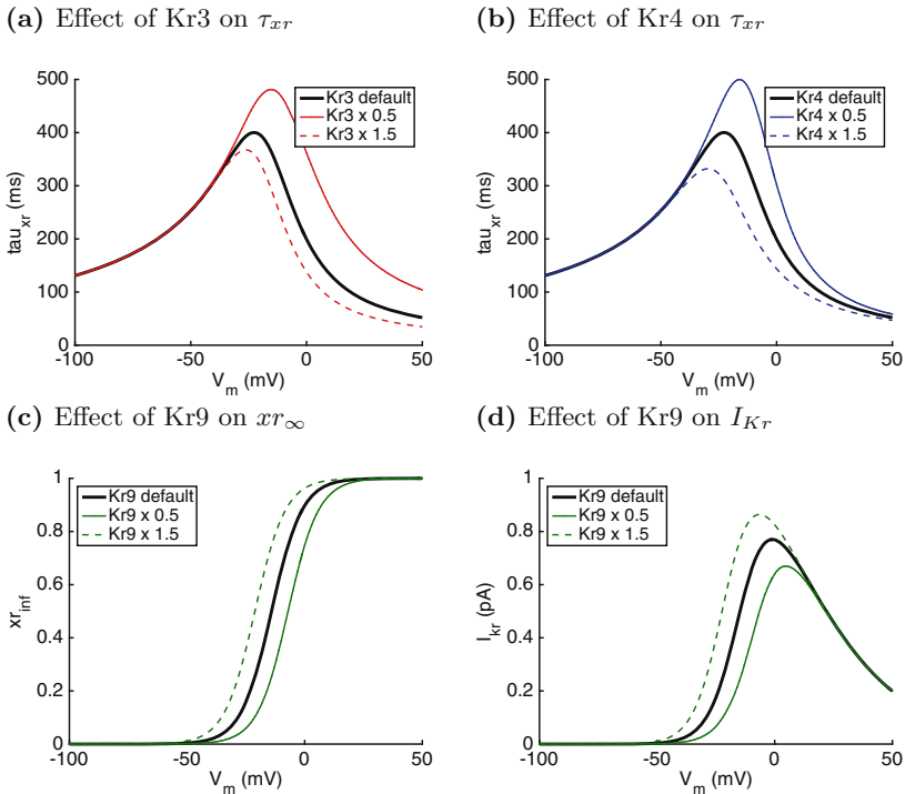
Fig. 5. Effect of multiplying inputs (a) Kr3 and (b) Kr4 by 0.5 and 1.5 on voltage dependence of \tau_{xr} , and effect of multiplying Kr9 by 0.5 and 1.5 on (c) xr_{\infty} , and (d) I_{Kr} calculated using steady state values of x_r , xr_{\infty} . Bold lines show baseline model output.
