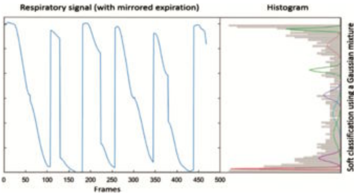
Fig. 3. Left – respiratory signal with mirrored expiration phases. Right – histogram of respiratory signal with overlaid GMM soft classification. Observe the different class sizes.
