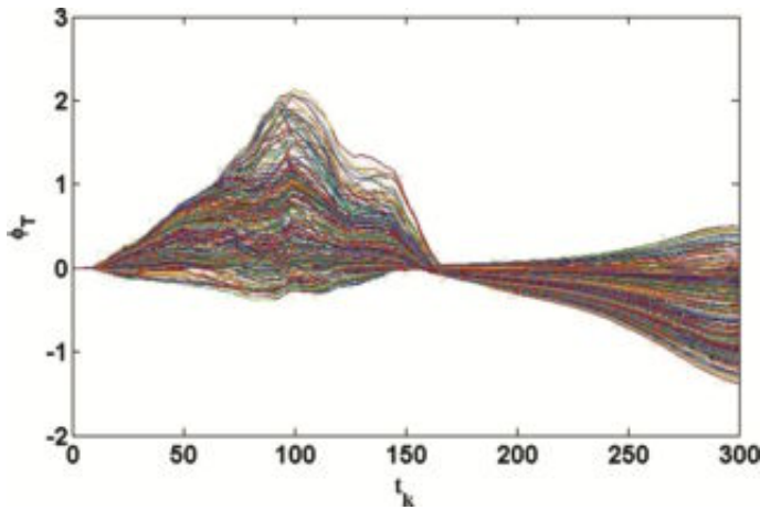
Fig. 1. In-silico body-surface potentials, \Phi_T for t_k = 1, \dots, 300 ms (corresponding to the first beat) of the single spiral wave used for the DPC plot example of Fig. 2.
