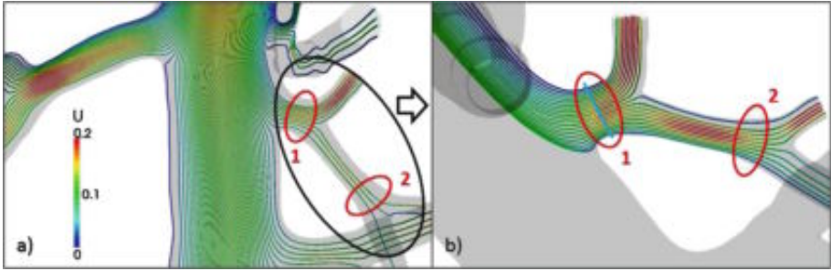
Fig. 6. Streamlines in branches 2 and 3 at 0.65s of one cardiac cycle (cf. Fig. 2), same timestep as Fig. 5(a). (a) Seed of the plotted streamlines is a horizontal 2D line source in the image plane ahead of the two branches at the upper end of the depicted model section. The sector encircled in black is represented enlarged in (b). The velocity scale (units ms^{-1} ) in (a) applies for both graphics. (b) The 2D line source used as seed is indicated in blue. The two branches and subsequent daughter vessels are “fed” from different cross sectional areals of the main branch. CA flow and velocities in the main branch thus strongly influence CA concentration time curves in branching vessels. (Color figure online)
