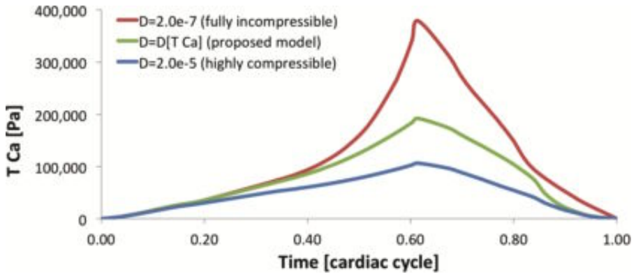
Fig. 5. Active contraction T_{Ca} inversely determined with the observed PV loop ( D = 2/K ). Active contraction increases up to a maximum at peak-systole, and relaxes over diastole. Incompressible myocardium requires substantially higher active contractions to achieve similar cavity volumes.
