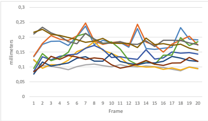
Fig. 5. The 2D curve distance measure ( cd , see Eq. 6), for the ten cases. The values are plotted for the 20 successive frames of the selected sub-sequence.
