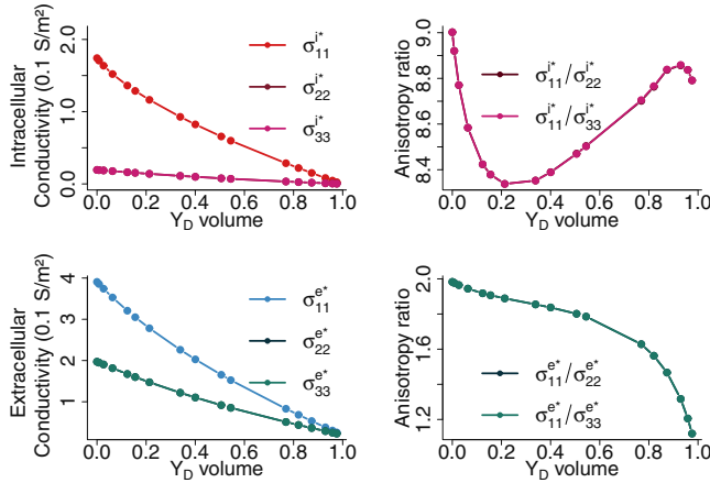
Fig. 3. Effective conductivities and anisotropy ratios for inclusions in the shape of cubes (see Fig. 2 at the bottom right), ranging in volume fraction from 0 to 98%, with fibers aligned with the x-axis.
