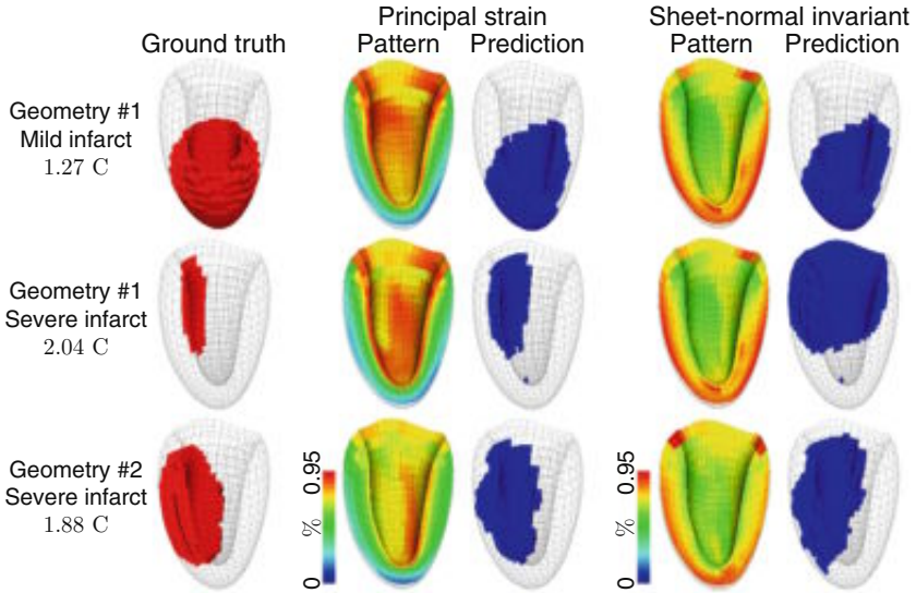
Fig. 2. Infarct localization for some pathological cases based on principal strain and sheet-normal invariant; amongst the best and the worst parameters, respectively.
