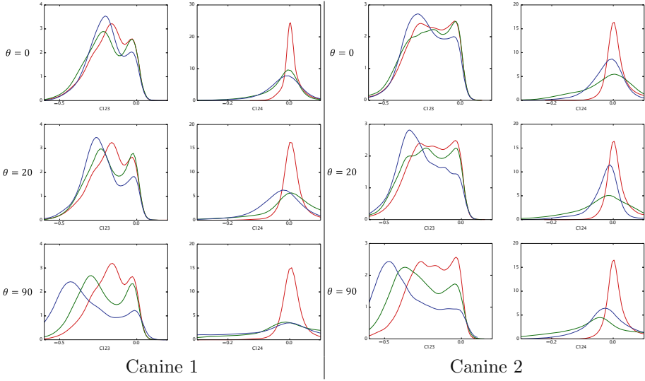
Fig. 3. We focus on c_{123} and c_{124} and show the effect of different choices for the total applied additional transmural rotation ( \theta ): 0^\circ (top), 20^\circ (middle) and 90^\circ (bottom) for two canine data sets. The red, green and blue curves show histograms corresponding to the 50 ms, 200 ms and 350 ms time samples in the systolic phase from 0 ms to 400 ms (Color figure online)
