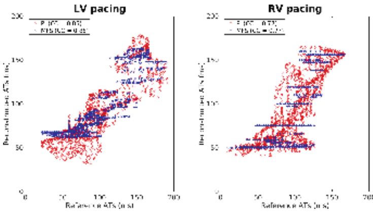
Fig. 3. Scatter plot of the ATs for in silico data. For each point, the x coordinate is the reference AT and the y coordinate is the corresponding reconstructed AT (PI in red, MFS in blue). (Color figure online)
