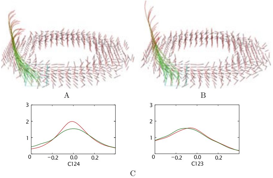
Fig. 4. In vivo heart wall fibers in a human left ventricle at two time points in the systolic phase: (A) 150 ms, (B) 220 ms. (C) Histograms of the Cartan connection parameters c_{124}, c_{123} , obtained via fits to (A) (red) and (B) (green). (Color figure online)
