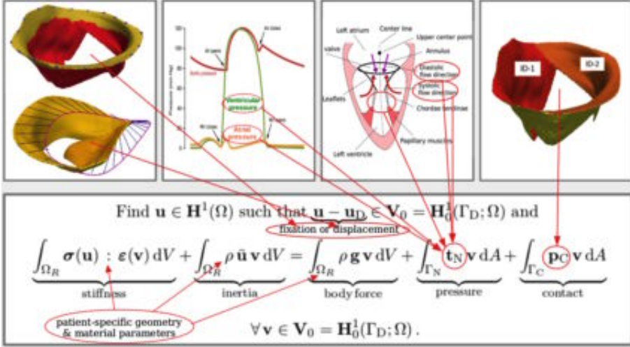
Fig. 1. Illustration of the specifications of the variational formulation of contact in elasticity for describing the MV behavior and MVR annuloplasty surgery.
