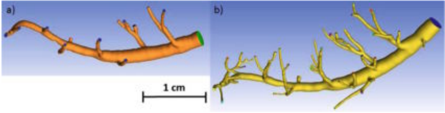
Fig. 1. Models to study vessel dependence of CA bolus dispersion, starting at first diagonal artery (vessel generation 3) branching off from LAD (inlet diameter \sim 2\text{mm} ). Model (a) includes generations 3–5 and (b) generations 3–7.
