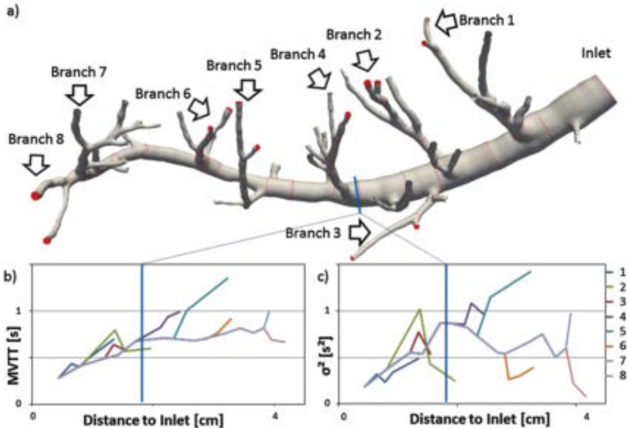
Fig. 4. Position of cross sectional planes and analysis of MVTT and \sigma^2 dependence on distance from model inlet. The vessel branches numbered in (a) are analyzed in more detail. (b) and (c) show the evolution of MVTT and \sigma^2 in the course of the numbered branches at discrete positions (red cross sections marked in (a)). The straight lines connecting the values solely serve to enhance visual presentation and do not hold any physical meaning. Close to the inlet both quantities increase. Travelling further along the considered vessels the behaviour varies strongly comprising dispersion as well as narrowing effects. Until the region marked in blue in the middle of the vascular model both quantities describe the expected monotonously increasing behavior. (Color figure online)
