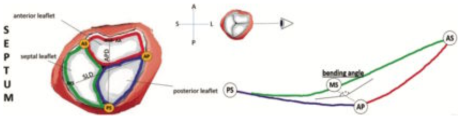
Fig. 3. Schematic of the tricuspid valve (left) and diagram of the annular bending angle measurement as viewed from the AP to MS (right). (A – anterior, P – posterior, S – septal, L – lateral, AP – anteroposterior commissure, AS – anteroseptal commissure, PS – posteroseptal commissure, MS – mid-septum, mid-AA – mid-anterior annulus, SLD – septal-lateral diameter, APD – anteroposterior diameter)
