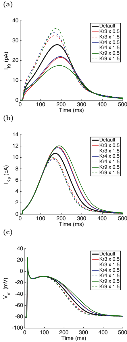
Fig. 6. Effect of multiplying inputs Kr3 , Kr4 , and Kr9 by 0.5 and 1.5 on the time course of (a) I_{Kr} , (b) I_{Ks} , and (c) V_m . Each plot shows the final action potential of a 40 beat sequence with a cycle length of 1000 ms, and the bold lines show model output for baseline parameter settings.
