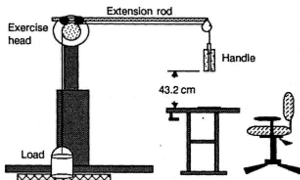
FIGURE 1. Experiment workstation.
