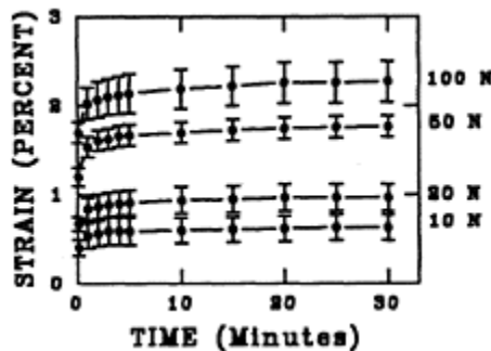
Figure 1 Results of Static Creep Test
