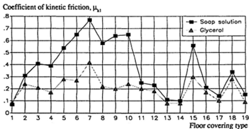
Figure 1. Coefficient of kinetic friction ( \mu_{kl} ) of 19 flooring types (mean value of 13 footwear types). A slip is unlikely to occur during normal walking when \mu_{kl} is at least 0.20.
