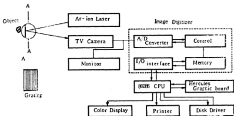
Fig.1 Data acquisition system
