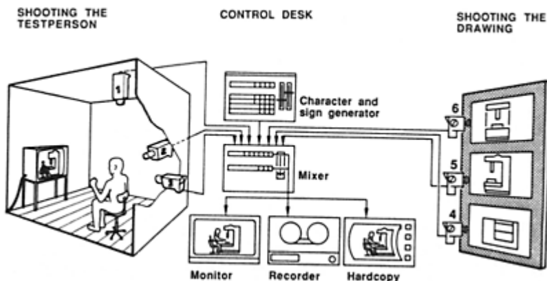
Fig. 2: Configuration of the videosomatography laboratory
