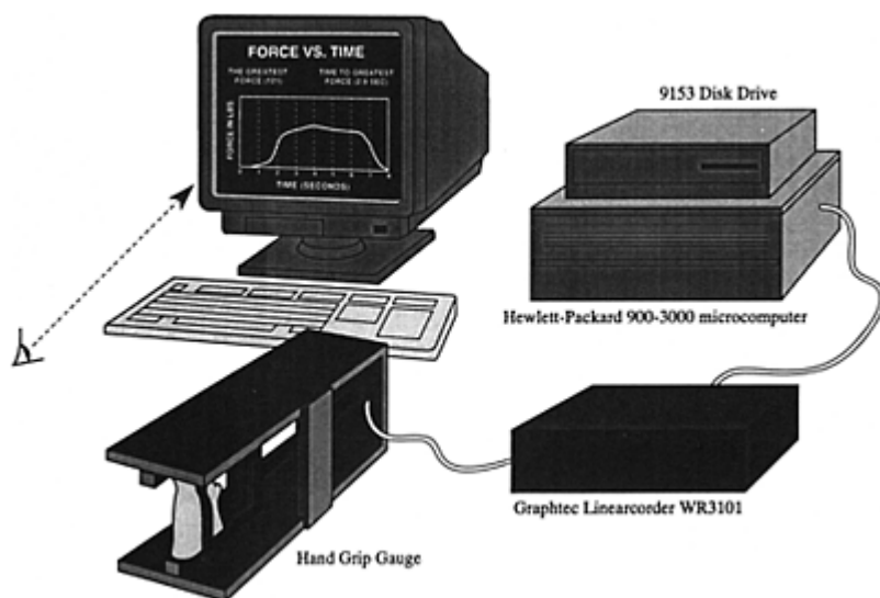
Figure 1. Experimental Configuration
