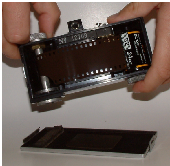
Fig 5-1: Loading the camera
