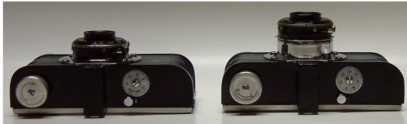
Fig 5-2: The Neck and Shutter in the storage position (left), and in the extended position (right)
