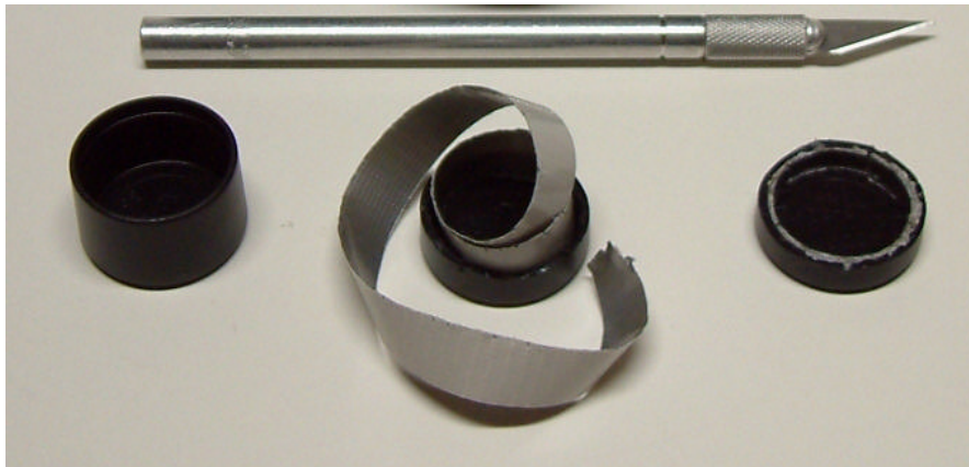
Fig. 6-4: A Lens Cap in various stages of production.
