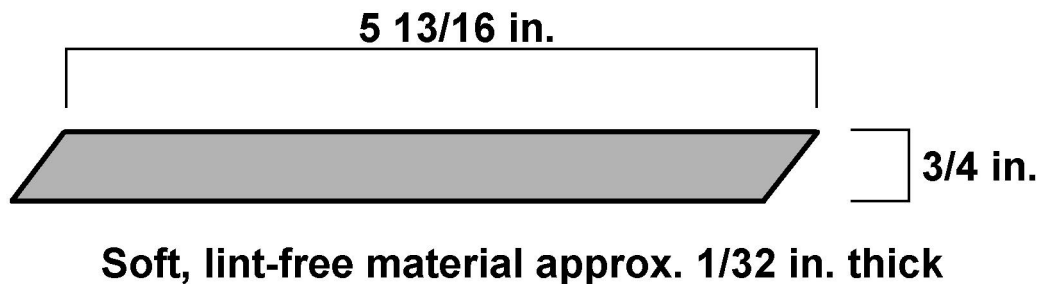
Fig. 7-1: Dimensions of light-proof ribbon in the Body cavity
