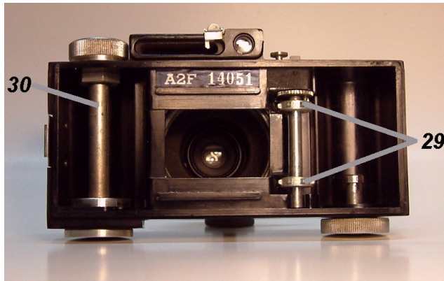
Fig. 4-6: Inside view of an Argus A2F
