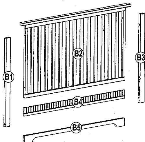
B1: Left Front leg (1pc) B4: Front Panel (1pc) B2: Front Frame(1pc) B5: Front Bottom rail (1pc) B3: Right Front leg (1pc)
