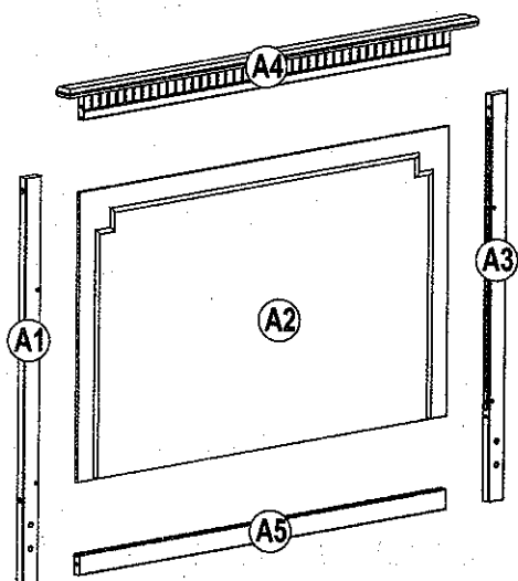
A1: Left back leg (1pc) A4: Back top (1pc) A2: Back Panel (1pc) A5: Back Bottom rail (1pc) A3: Right Back leg (1pc)
