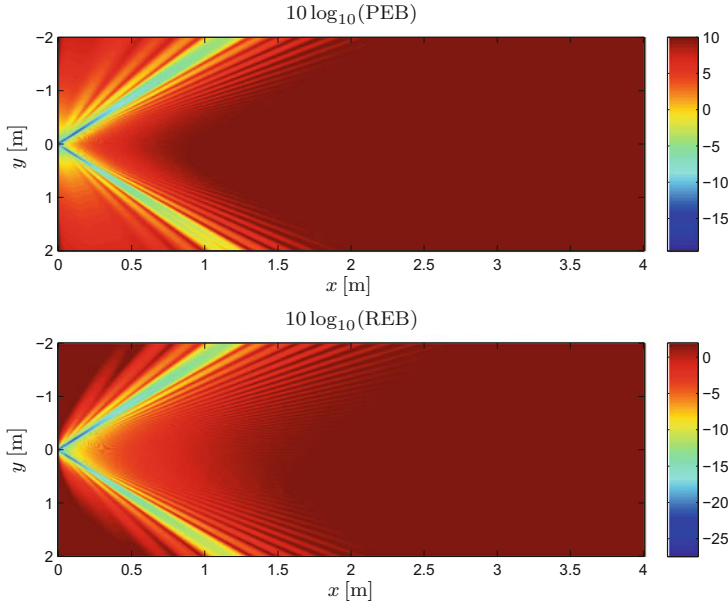
Fig. 9.18 Performances of the PEB ( top ) and REB ( bottom ) in the LOS for different locations of the MS and the BS located at \mathbf{q} [\text{m}] = [0, 0]^T , for a scenario with three beams in the directions [\pm\pi/3, \pi/3 + 0.01]
