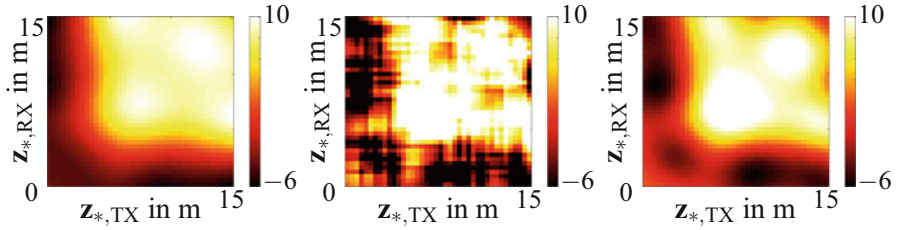
Fig. 10.7 Left: expected received power P_{RX,avg} for one realisation of the spatially correlated shadowing field for different expected positions \mathbf{z}_{*,TX} , and \mathbf{z}_{*,RX} , respectively. The channel is symmetric reciprocal along the diagonal ( \mathbf{z}_{*,TX} = \mathbf{z}_{*,RX} ), i.e., the field is symmetric. Middle: prediction of P_{RX,avg} using cGP. Right: prediction of P_{RX,avg} using uGP. Note, cGP and uGP maintain channel reciprocity in their prediction
