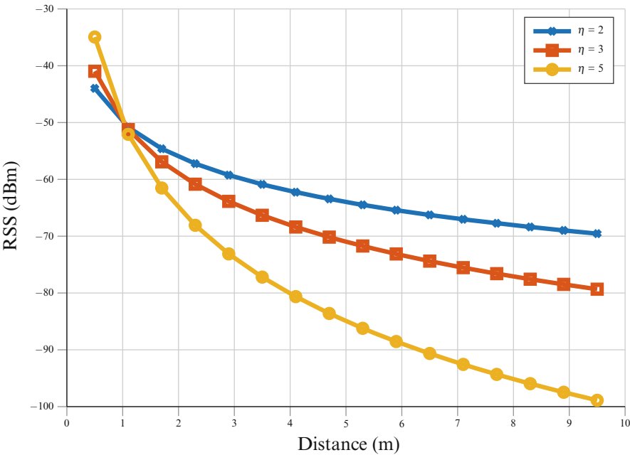
Fig. 8.3 Path-loss illustration with different exponents using log-distance model
