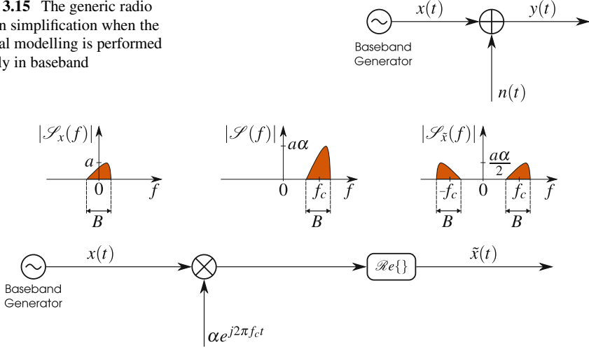
Fig. 3.16 Schematic diagram of the transmitter part
