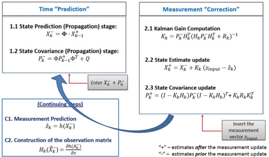
Fig. 5.8 The L1/E1 VDFLL estimation filter workflow [29]
