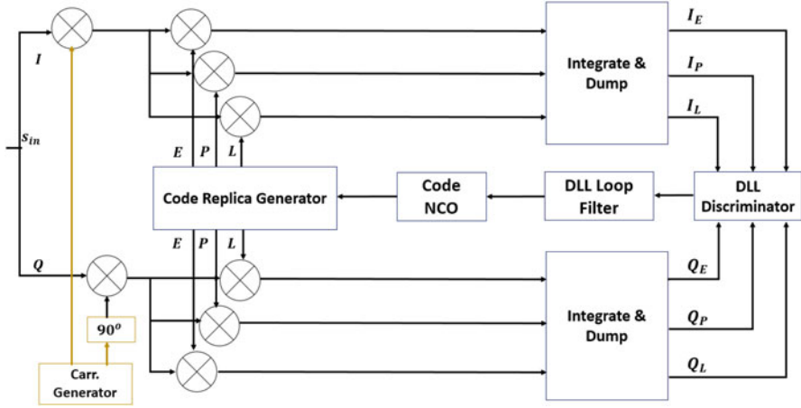
Fig. 5.3 GNSS Delay Lock Loop architecture. The orange blocks are related to the carrier tracking and are outside the DLL
