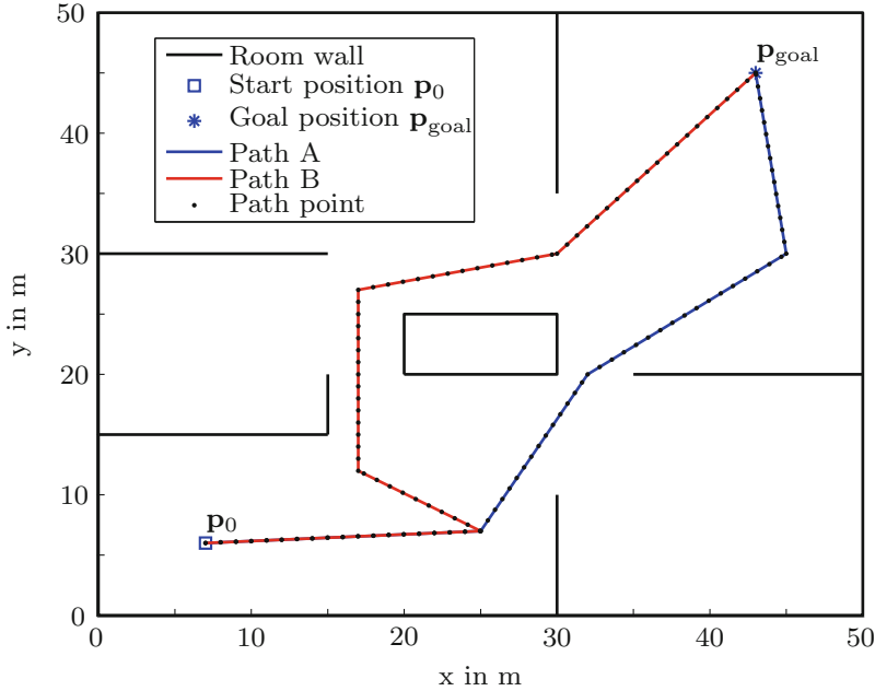
Fig. 10.1 A scenario with two paths A and B from a start position \mathbf{p}_0 = [7, 6]^T to a goal position \mathbf{p}_{\text{goal}} = [43, 45]^T . The objective of the agent is to determine which path has the lowest cost, while ensuring a certain positioning quality
