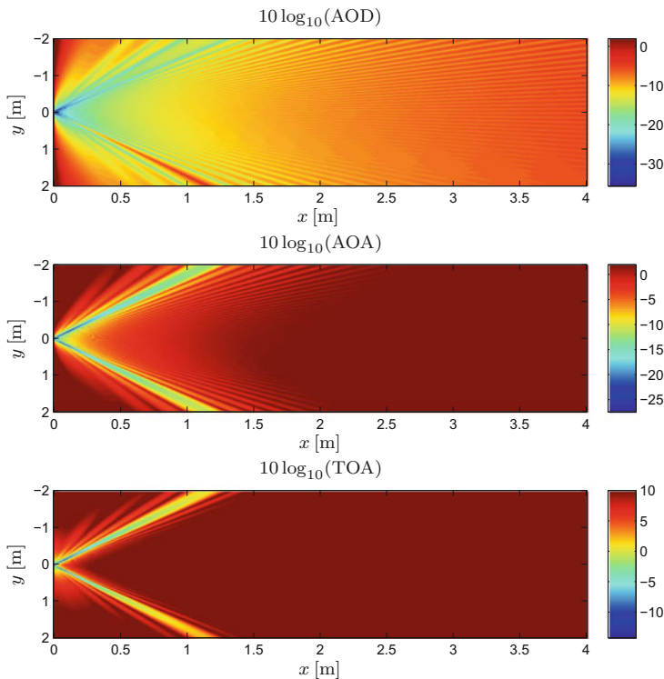
Fig. 9.17 Performances of the AOD, AOA, and TOA in the LOS for different locations of the MS and the BS located at \mathbf{q} [\text{m}] = [0, 0]^T , for a scenario with three beams in the directions [\pm\pi/3, \pi/3 + 0.01]
