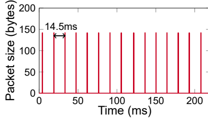
Fig. 24. Examples of VR traffic pattern (Airborne 1944 VR game in VRidge); Packets arrive at intervals 14.5 \pm 0.4\text{ms} .
