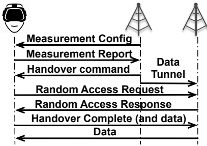
Fig. 8. Handover process.
