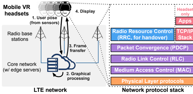
Fig. 1. Mobile VR over 4G (left); LTE protocol stack (right).
