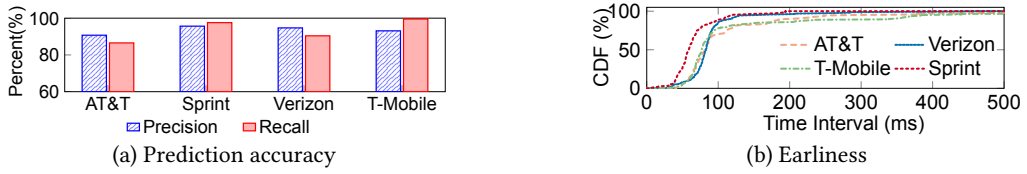
Fig. 22. Effectiveness of LTE-VR's handover prediction.
