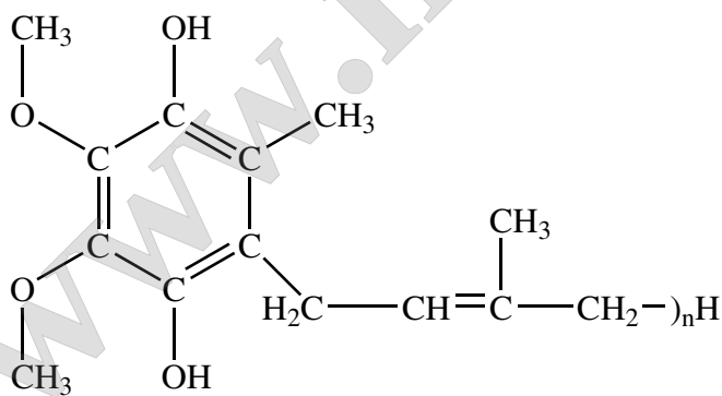
Reduced ubiquinolone
