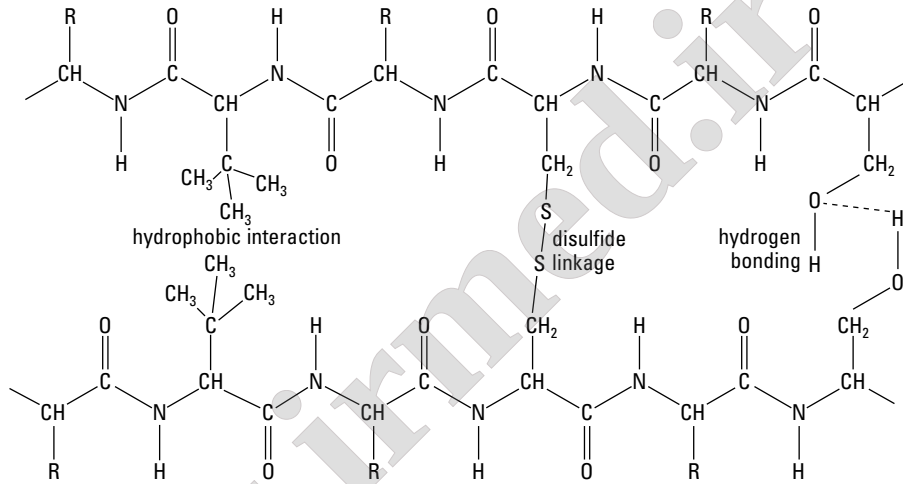
Figure 5-6: Some tertiary structures appearing in proteins.
