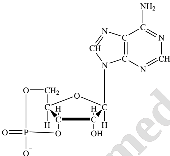
Figure 11-5: Structure of cyclic AMP.
