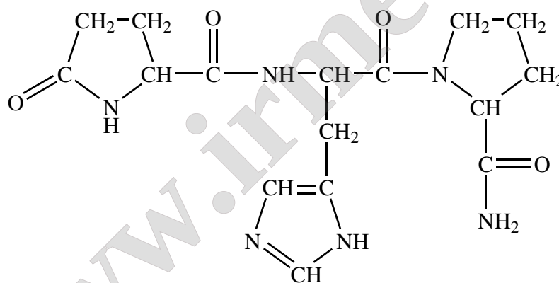
Figure 11-1: Structures of the growth- hormone- release- inhibitory factor and thyrotropin- releasing factor.
