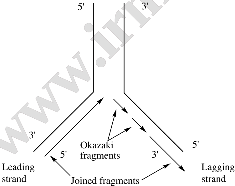
Figure 15-4: Detailed scheme of the replication of DNA.
