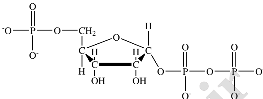
5-phospho-α-D-ribose 1-pyrophosphate (PRPP)
