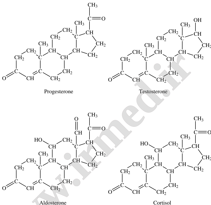
Figure 11-2: Structures of progesterone (an estrogen), testosterone (an androgen), and aldosterone and cortisol, adrenal cortical hormones.
