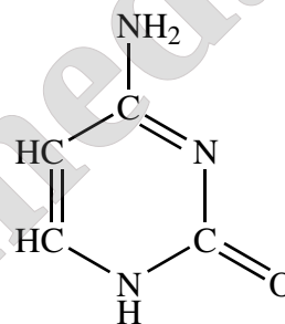
Cytosine (C)
