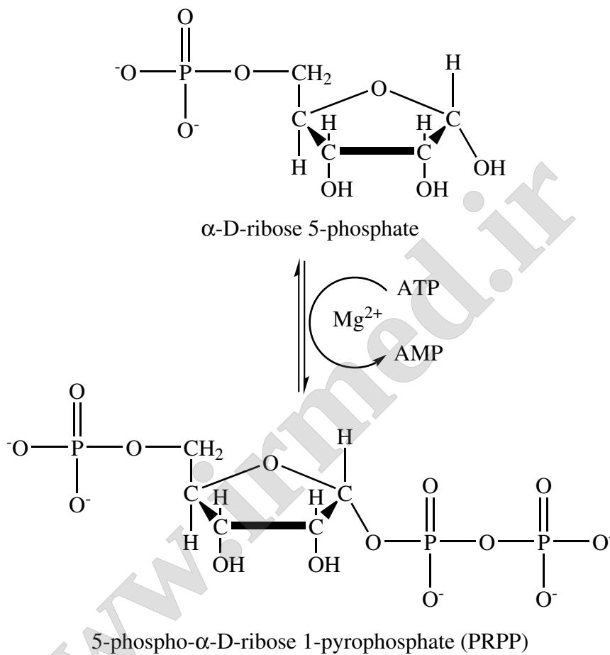
Figure 14-2: Activation of D-ribose-5'- phosphate.
