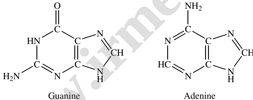
Figure 15-9: The purines.
