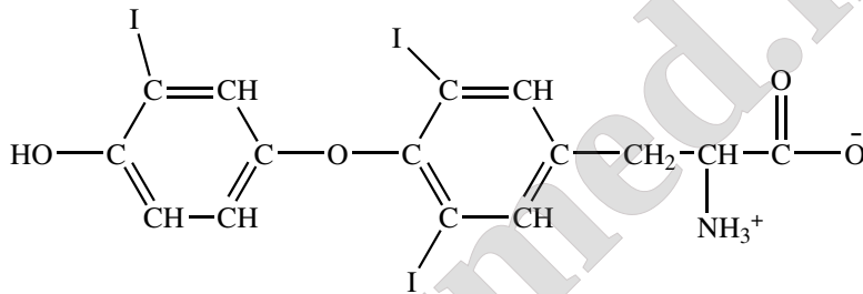
Triiodothyronine
