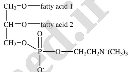
phosphatidylcholine
