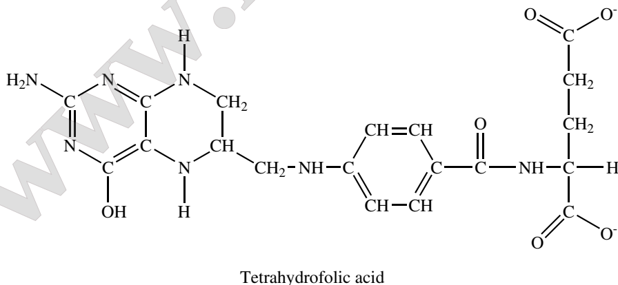
Figure 10-6: Structures of folic acid and tetrahydro- folic acid.
