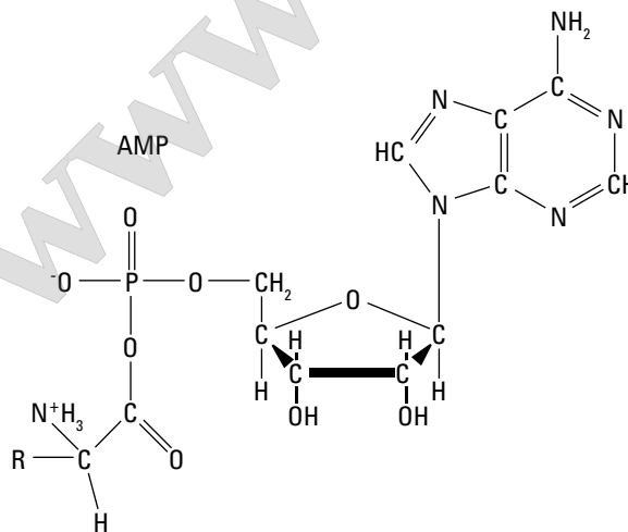
Figure 17-6: Structure of an aminoacyl adenylate.
