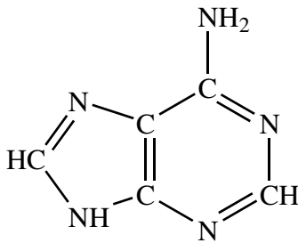
Adenine
