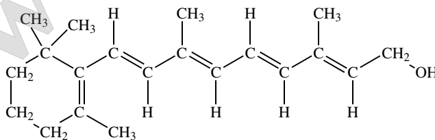
11-trans-retinol
