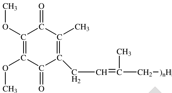
Oxidized ubiquinone
