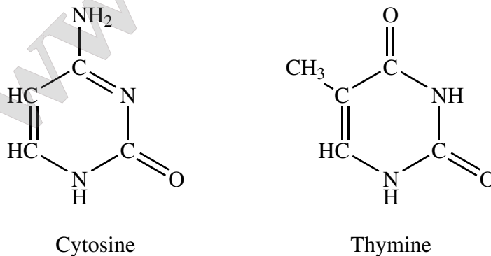
Figure 15-10: The pyrimidines.
