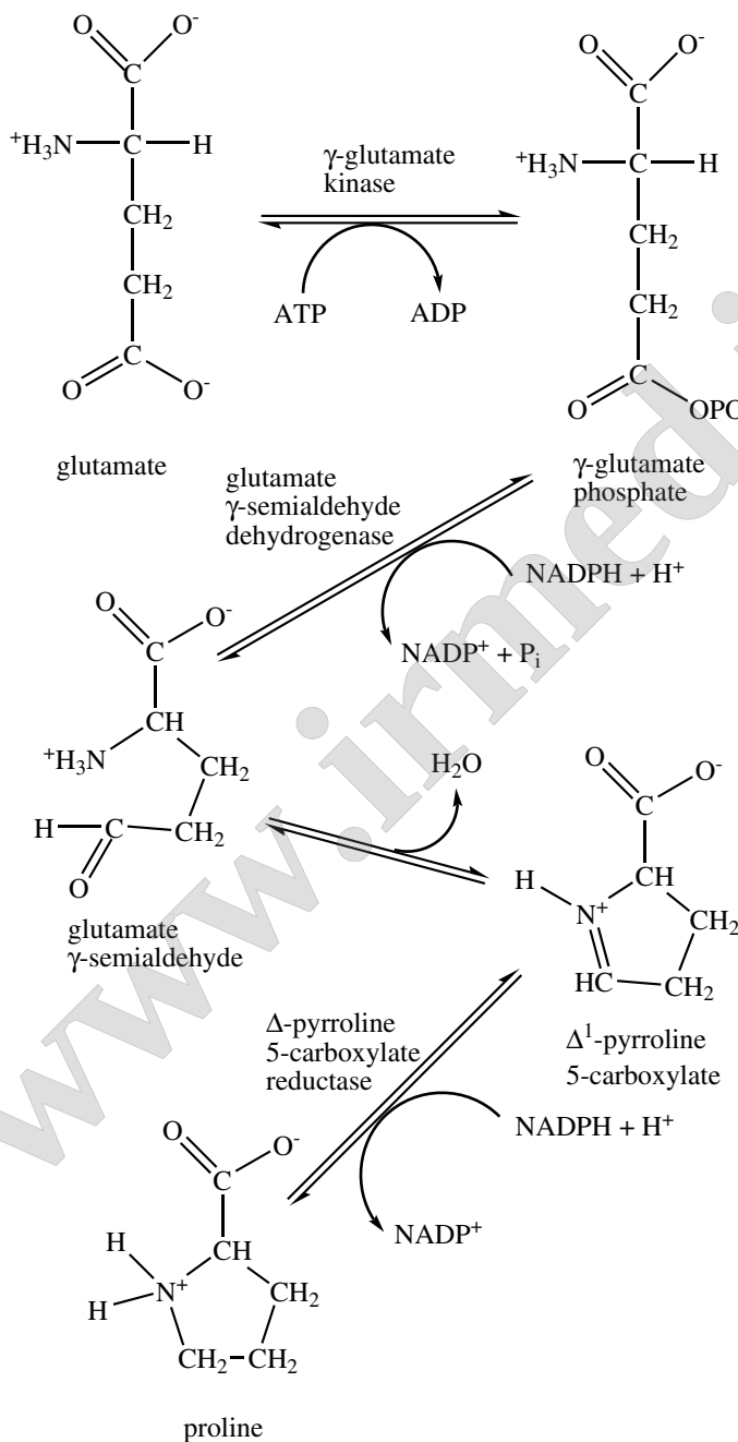
Figure 13-26: Synthesis of proline.
