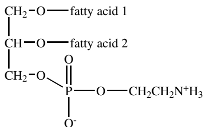
phosphatidylethanolamine
