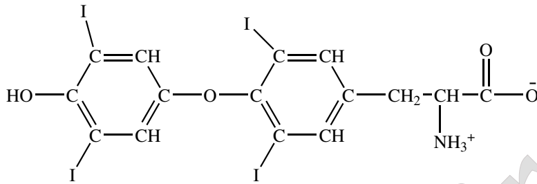
Thyroxine
