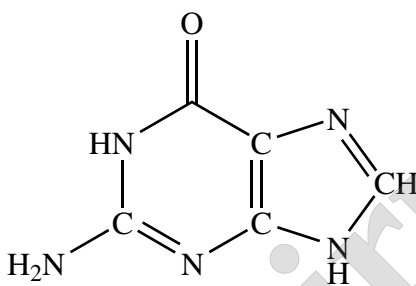
Guanine (G)
