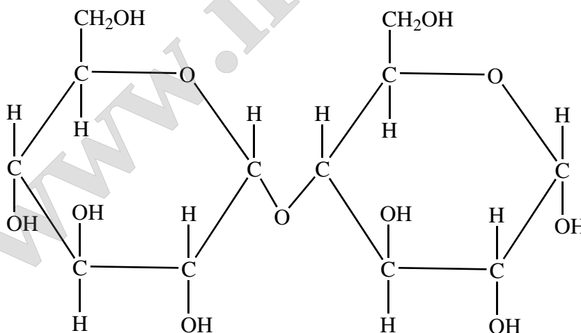
Figure 7-16: The structure of maltose with a \alpha(1-4) linkage present.
