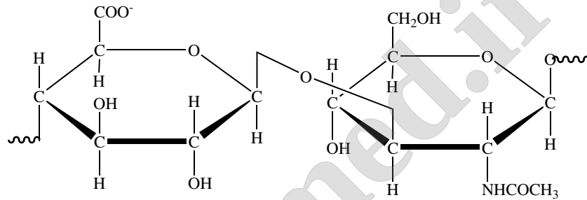
Hyaluronate
