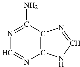
Adenine (A)
