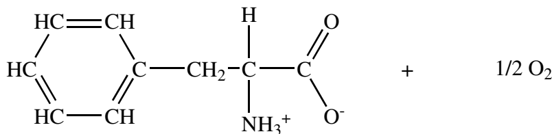
phenylalanine
