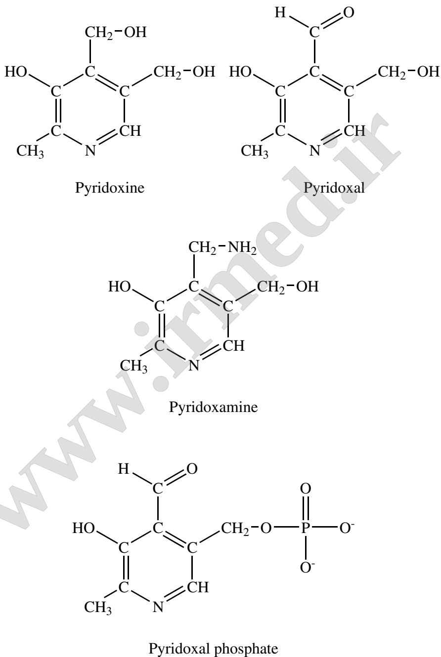
Figure 10-4: Structures of pyridoxine, pyridoxal, pyridoxa- mine, and pyridoxal phosphate.
