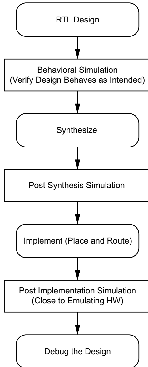
Figure 1-1: Simulation Flow
