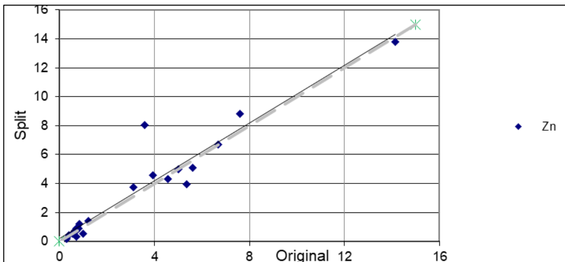
Figure 11.13 – El Mochito duplicate split sample results – Zn (n=22)
