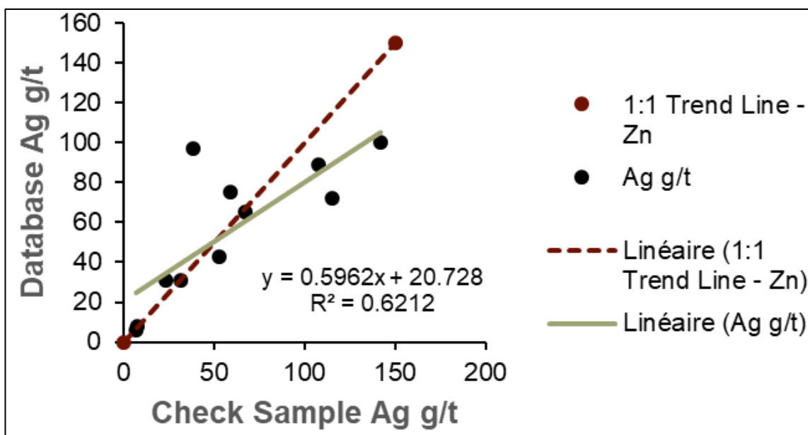
Figure 12.5 – Mercator quarter core check samples – silver (N=11)
