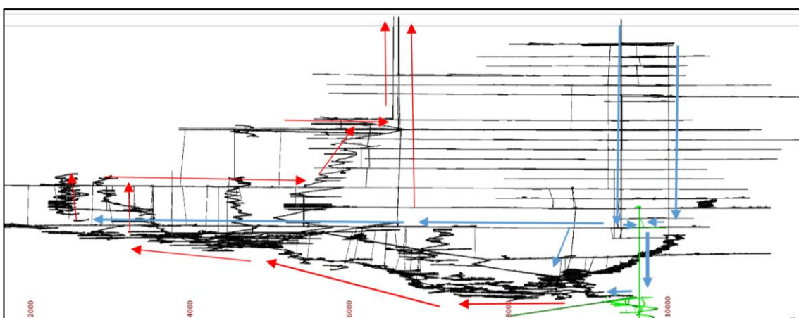
Figure 16.16 – Long section of El Mochito mine showing the proposed mine ventilation network, including the No. 8 shaft infrastructure
