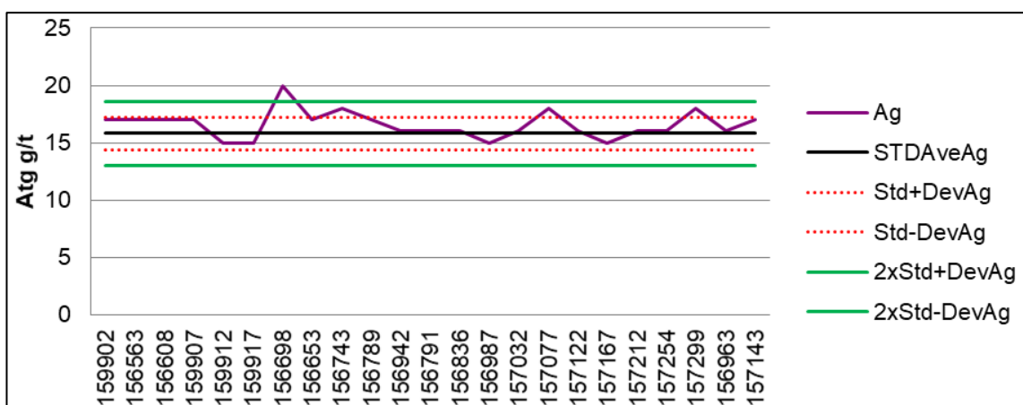
Figure 11.9 – 2017 El Mochito certified reference material (low) results – Ag (n=23)
