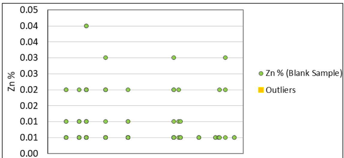
Figure 11.10 – El Mochito coarse blank sample results – Zn (n=119)
