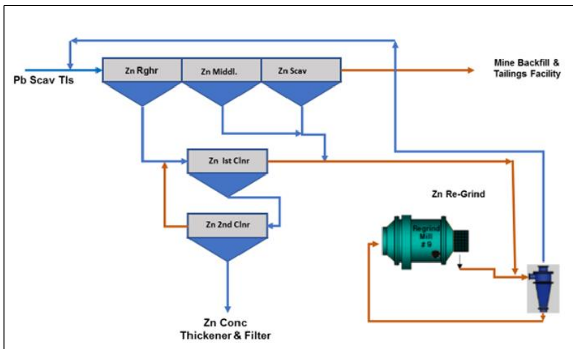
Figure 17.11 – El Mochito zinc flotation circuit
