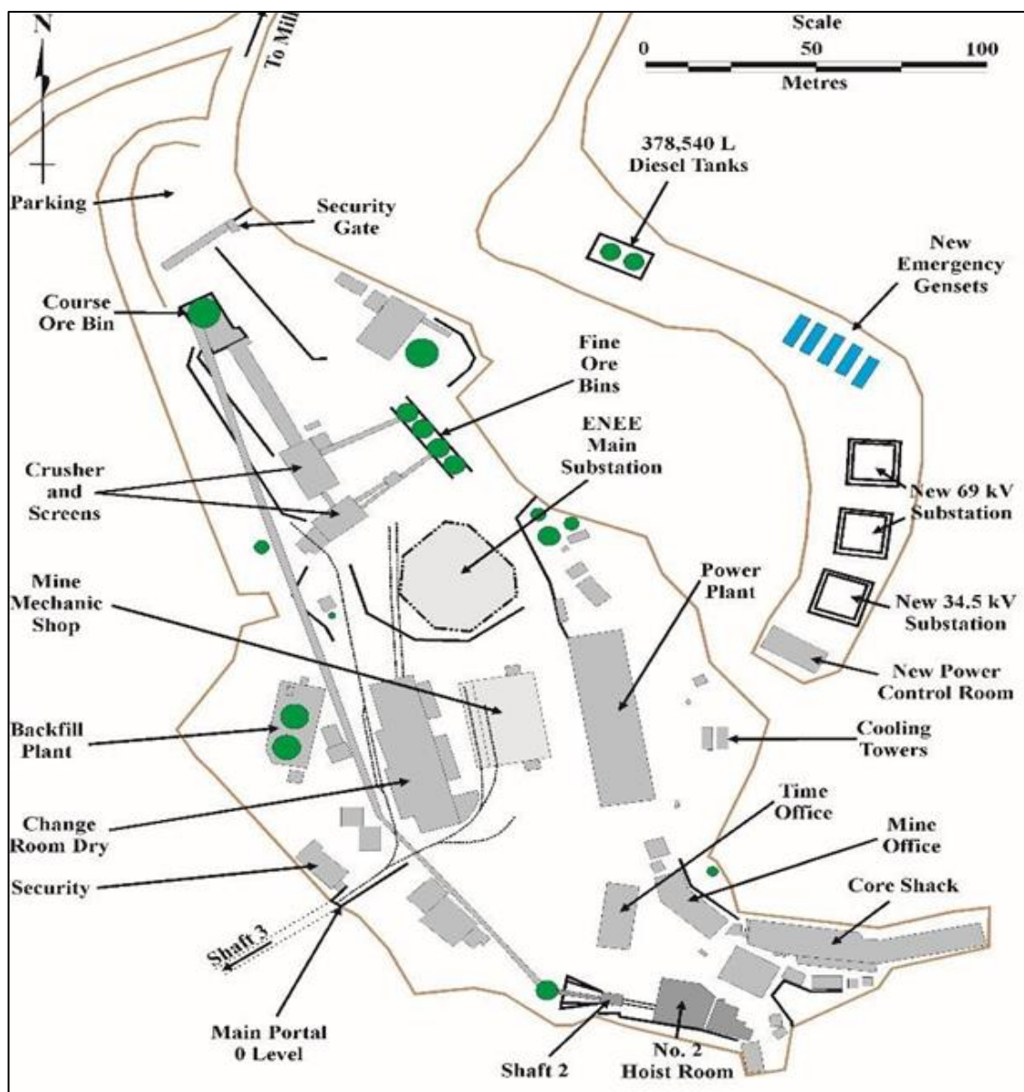
Figure 18.3– Mine surface infrastructure
