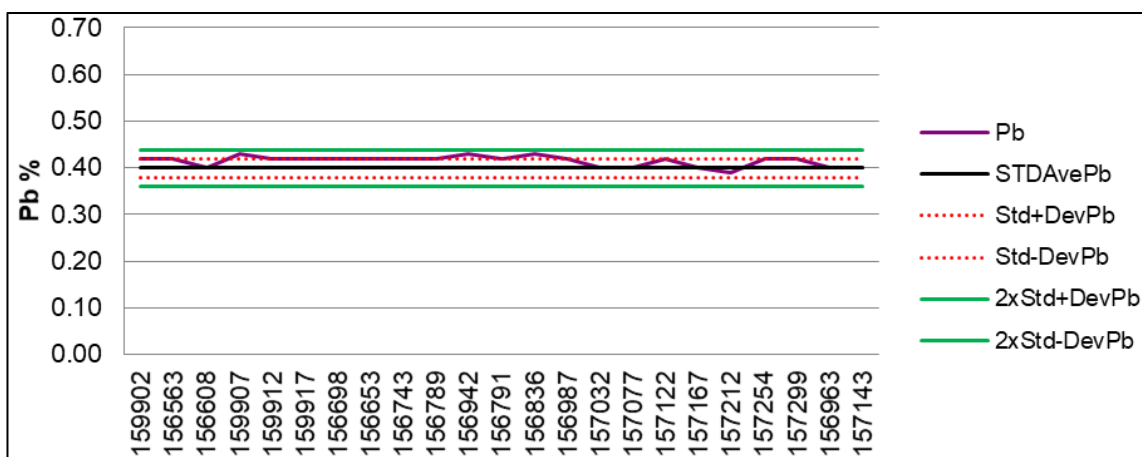
Figure 11.8 – 2017 El Mochito certified reference material (low) results – Pb (n=23)
