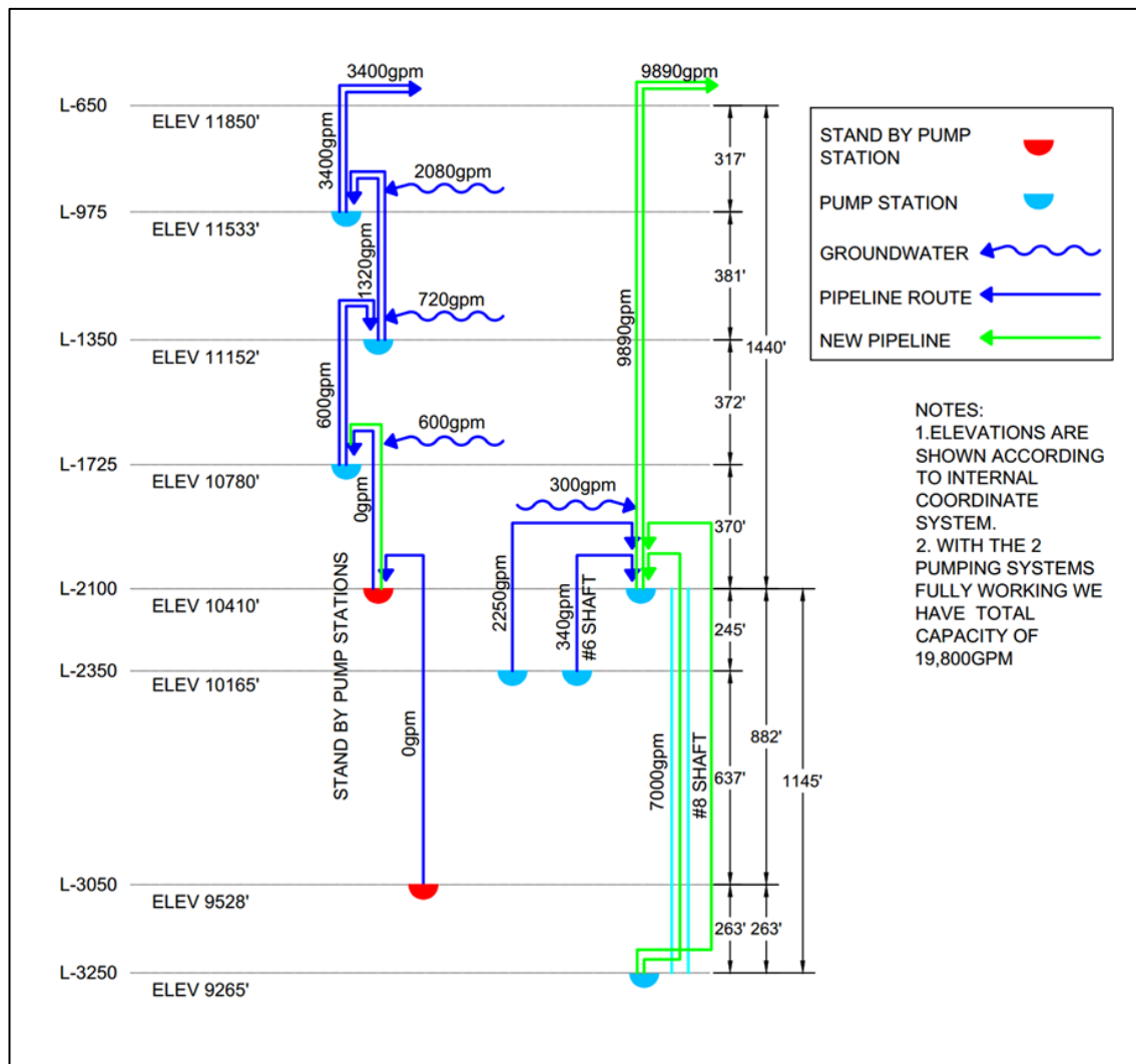
– New water configuration, Phase II, El Mochito mine (Figure 16.17)
