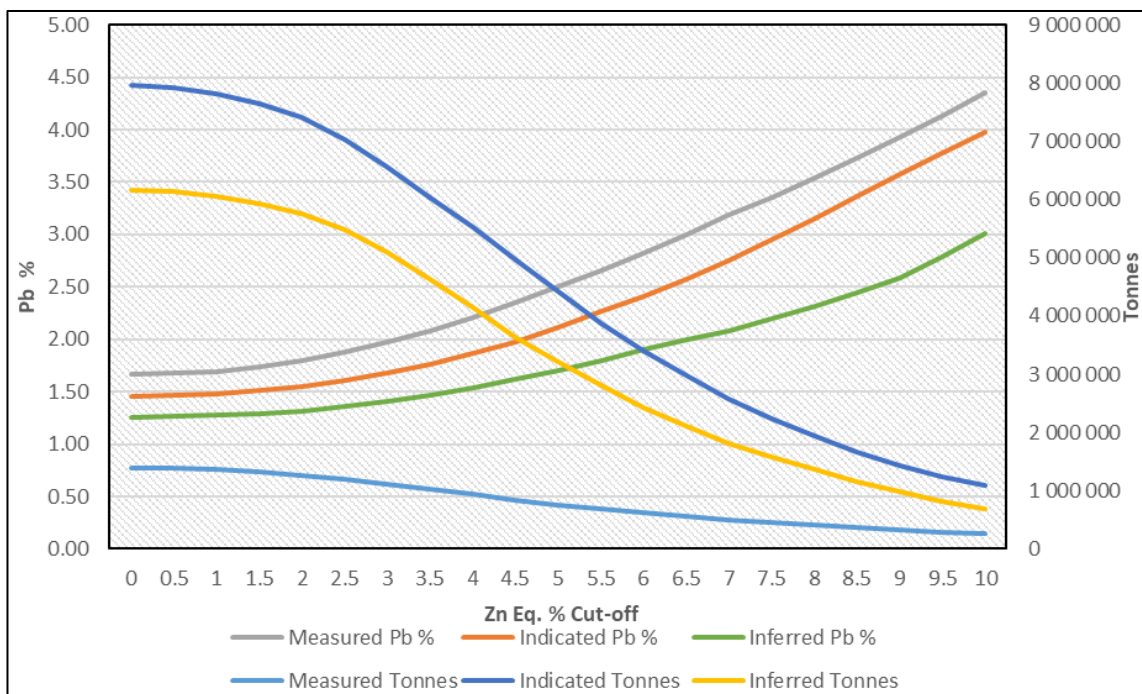
Figure 14.16 – El Mochito mine Pb% grade tonnage chart
