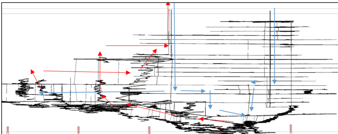
Figure 16.15 – Long section of El Mochito mine showing a simplified, existing mine ventilation network.
