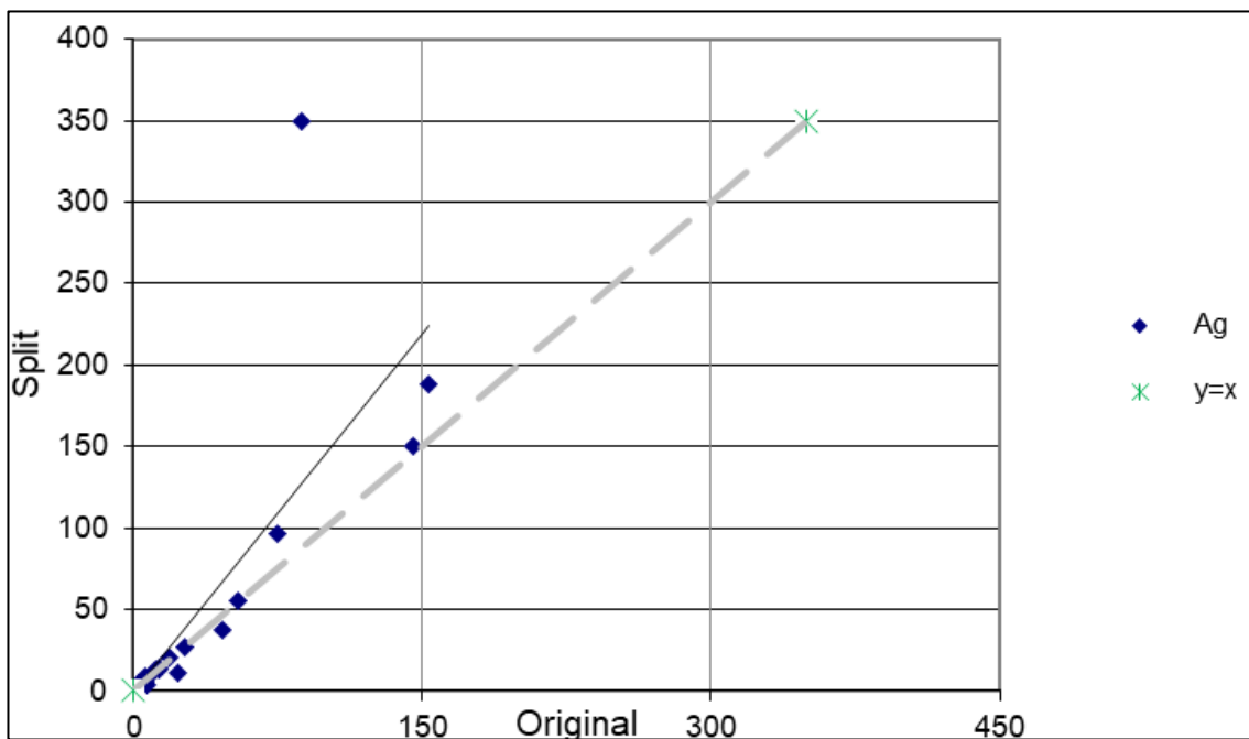
Figure 11.15 – 2017 El Mochito duplicate split sample results – Ag (n=22)
