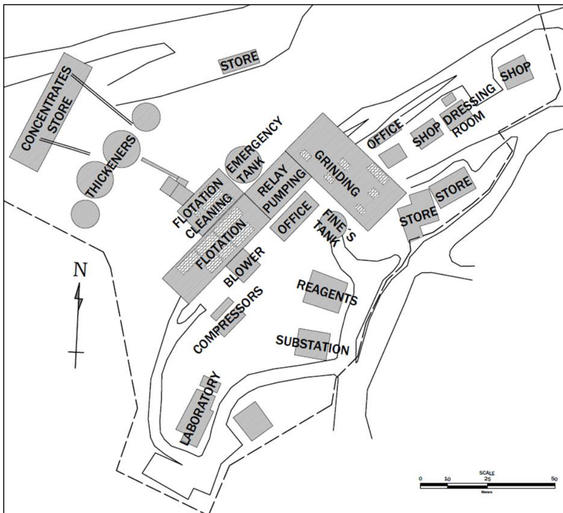
Figure 18.15 – Layout of the concentrator plant
