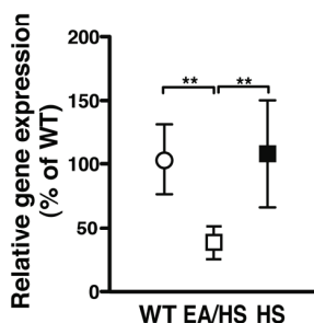
Fig. 8. Gene expression as related to hindlimb suppression and EA effect. Real-time RT-PCR analysis of expression of Mstn (myostatin) (a), MuRF-1 (b), and MAFbx (c) genes in control, HS, and EA/HS mice (for each group, n = 7 ). Relative transcript levels are shown (means \pm S.D.). Open circle, control mice; closed squares, HS mice; open squares, EA/HS mice; * P < 0.05 ; ** P < 0.01 ; *** P < 0.005 ; NS, not significant.
