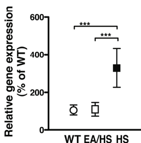
Fig. 8. Gene expression as related to hindlimb suppression and EA effect. Real-time RT-PCR analysis of expression of Mstn (myostatin) (a), MuRF-1 (b), and MAFbx (c) genes in control, HS, and EA/HS mice (for each group, n = 7 ). Relative transcript levels are shown (means \pm S.D.). Open circle, control mice; closed squares, HS mice; open squares, EA/HS mice; * P < 0.05 ; ** P < 0.01 ; *** P < 0.005 ; NS, not significant.
